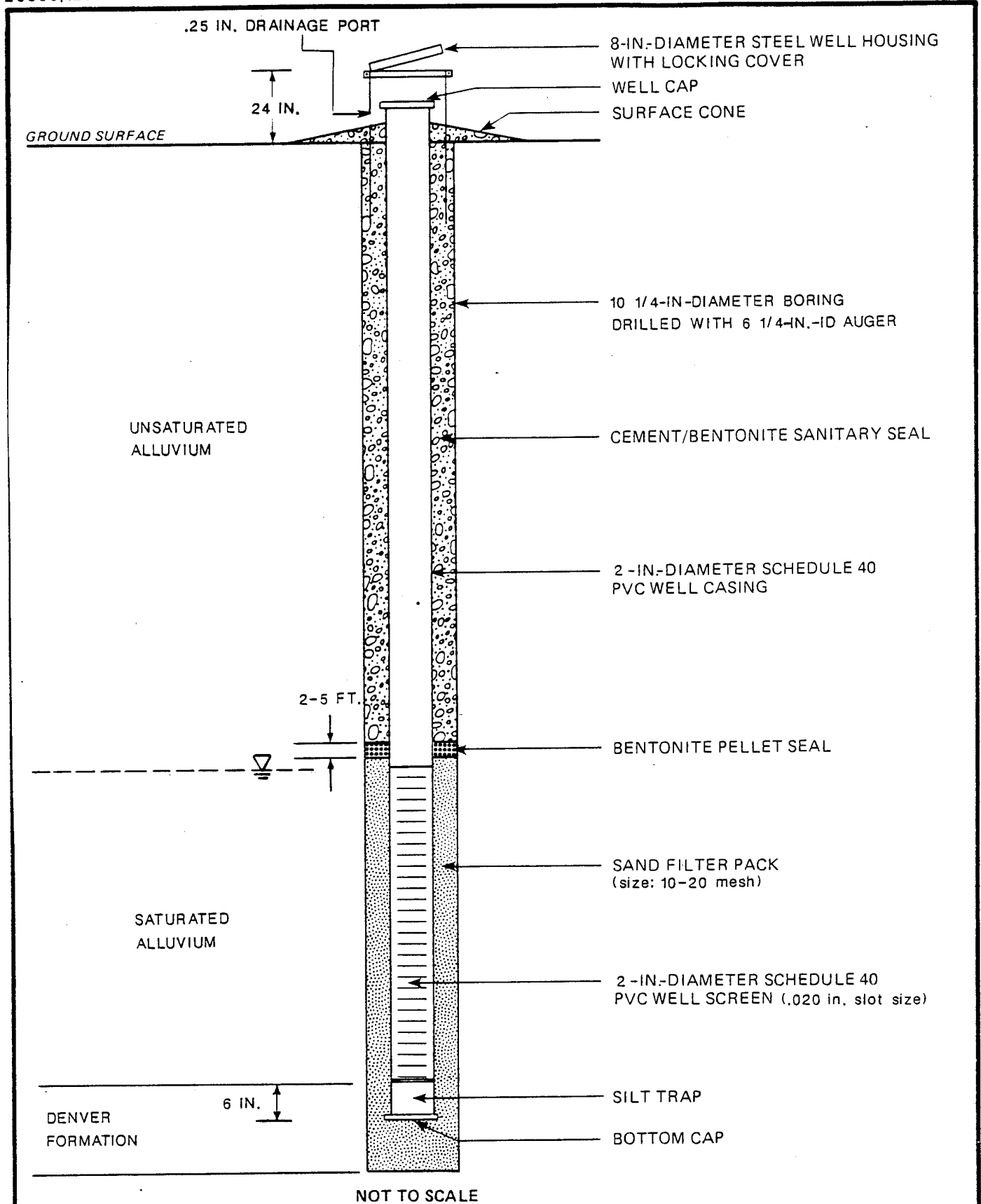
Figure 3.2 GENERALIZED CONSTRUCTION FOR ALLUVIAL/UNCONFINED PIEZOMETER
