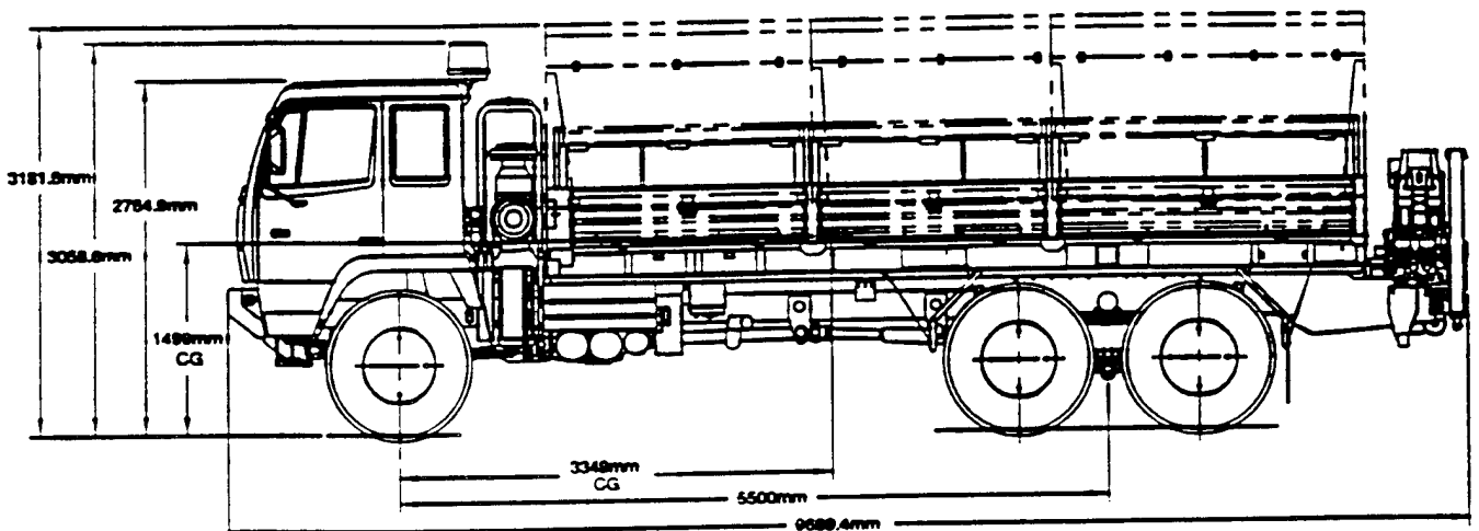
Vehicle Model .....M1086
