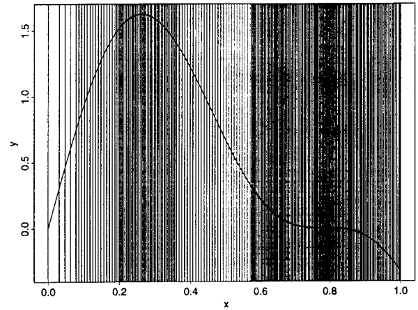
Figure 17: How CLA-2 chooses to sample its points. Vertical lines have been drawn at the x values where the CLA queried the oracle for the corresponding function value.
