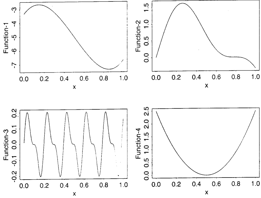
Figure 16: Four functions with bounded derivative considered in the simulations. The uniform bound on the derivative was chosen to be d = 10 .
