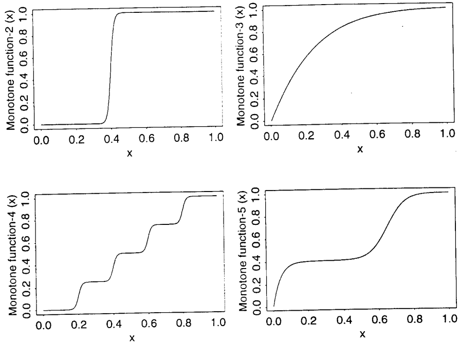
Figure 9: Four other monotonic functions on which simulations have been run comparing random, uniform, and active sampling strategies.
