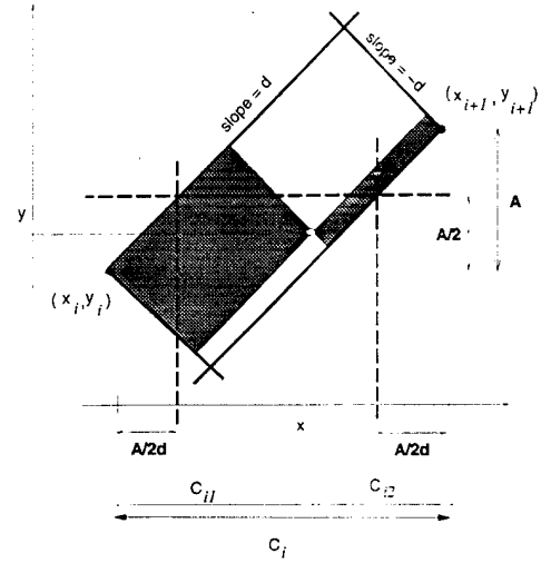
Figure 15: A figure to help the visualization of Lemma 4. For the x shown, the set \mathcal{F}_D is the set of all values which lie within the parallelogram corresponding to this x , i.e., on the vertical line drawn at x but within the parallelogram.
