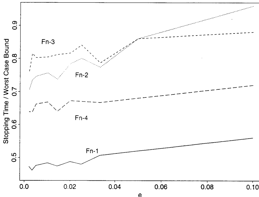
Figure 20: Variation with epsilons.
