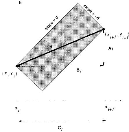
Figure 13: A zoomed version of the i th interval.
