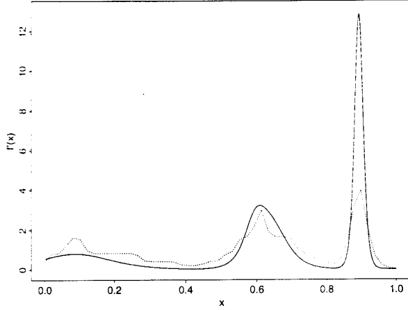
Figure 6: The dotted line shows the density of the samples along the x-axis when the target was the monotone-function of the previous example. The bold line is a plot of the derivative of the function. Notice the correlation between the two.
