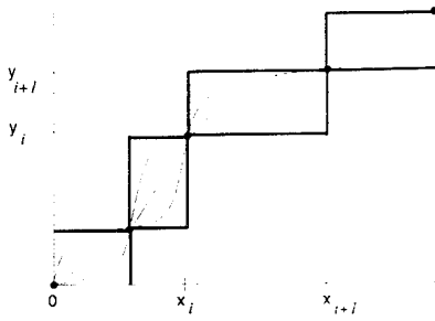
Figure 2: A depiction of the situation for an arbitrary data set. The set \mathcal{F}_D consists of all functions lying in the boxes and passing through the datapoints (for example, the dotted lines). The approximating function h is a linear interpolant shown by a solid line.
