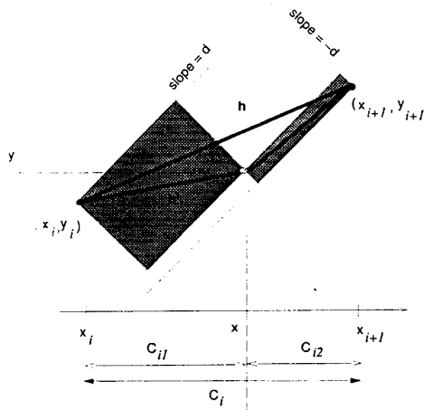
Figure 14: Subdivision of the i th interval when a new data point is obtained.
