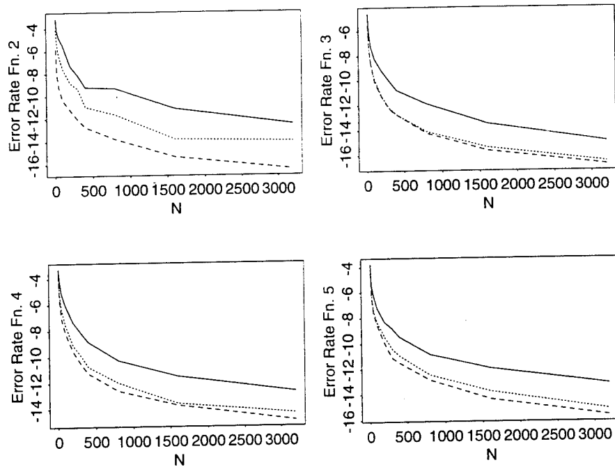
Figure 10: This figure plots the log of the error ( L_1 error) against N the number of examples for each of the 4 monotonic functions shown in fig. 9. The solid line represents error rates for random sampling, the line with small dashes represents uniform sampling and the line with long dashes represents results for CLA. Notice how CLA beats random sampling by large amounts and does slightly better than uniform sampling.
