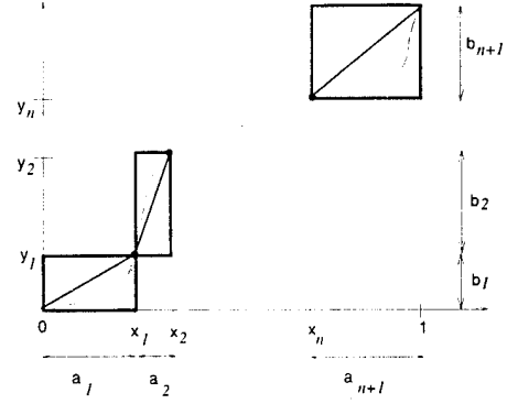
Figure 7: The situation when a function f \in \mathcal{F} is picked, n sample points (the x 's) are chosen and the corresponding y values are obtained. Each choice of sample points corresponds to a choice of the a 's. Each choice of a function corresponds to a choice of the b 's.
