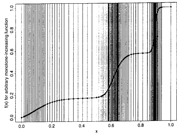
Figure 5: How the CLA chooses its examples. Vertical lines have been drawn to mark the x-coordinates of the points at which the algorithm asks for the value of the function.
