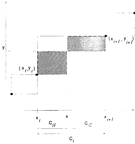
Figure 4: The situation when the interval C_i is sampled yielding a new data point. This subdivides the interval into two subintervals and the two shaded boxes indicate the new constraints on the function.
