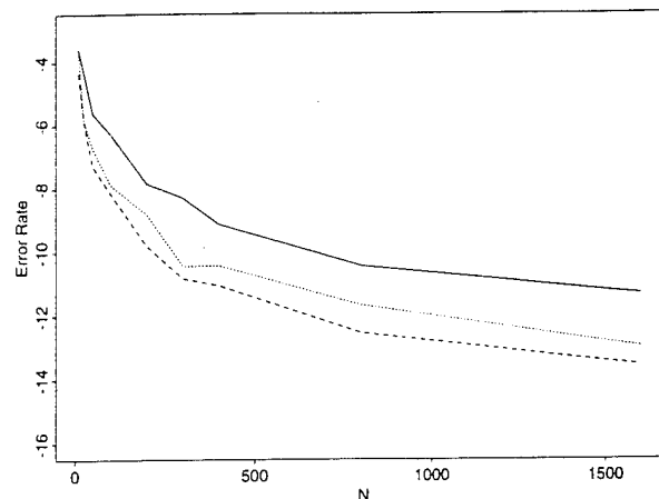
Figure 8: Error rates as a function of the number of examples for the arbitrary monotone function shown in a previous figure.
