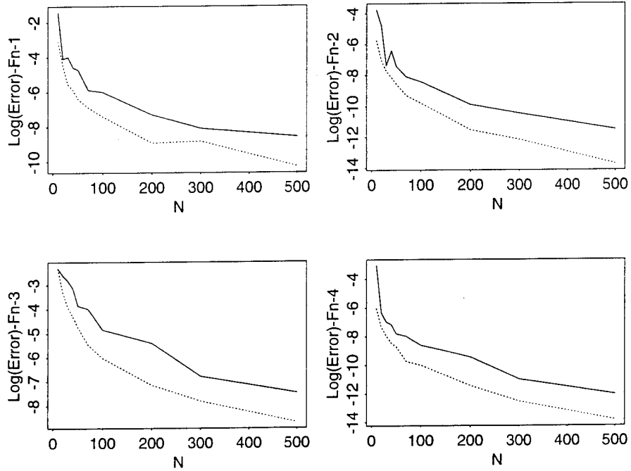
Figure 19: Results of Simulation B. Notice how the sampling strategy of the active learner causes better approximation (lower rates) for the same number of examples.
