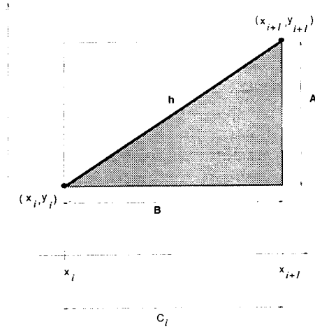
Figure 3: Zoomed version of interval. The maximum error the approximation scheme could have is indicated by the shaded region. This happens when the adversary claims the target function had the value y_i throughout the interval.
