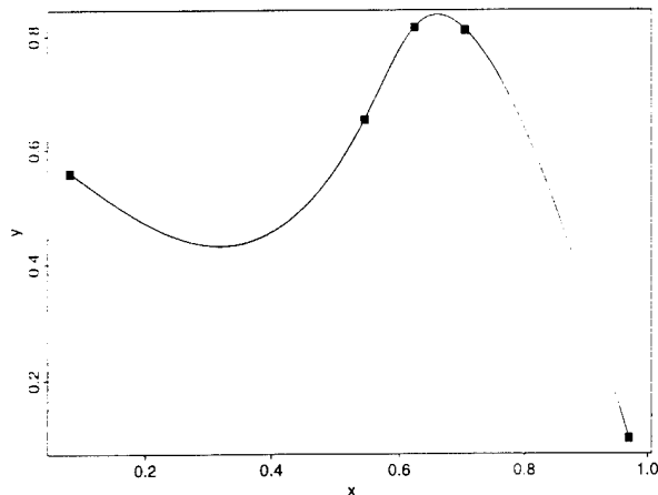
Figure 1: An arbitrary data set fitted with cubic splines
