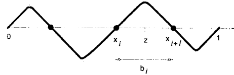
Figure 11: Construction of a function satisfying Lemma 2.
