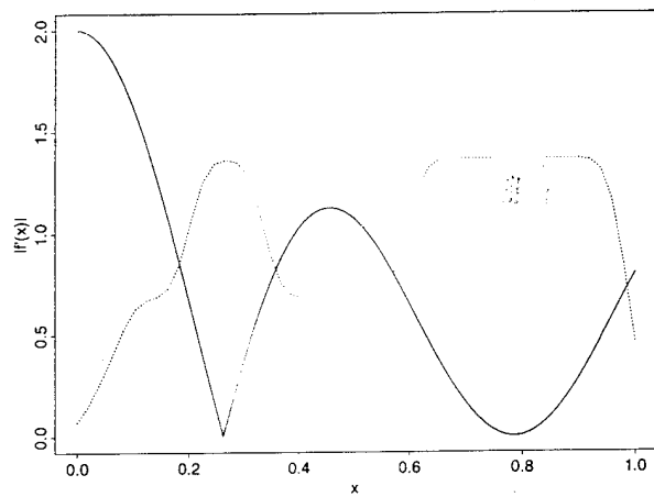
Figure 18: How CLA-2 chooses to sample its points. The solid line is a plot of |f'(x)| where f is Function-1 of our simulation set. The dotted line shows the density of sample points (queried by CLA-2) on the domain.
