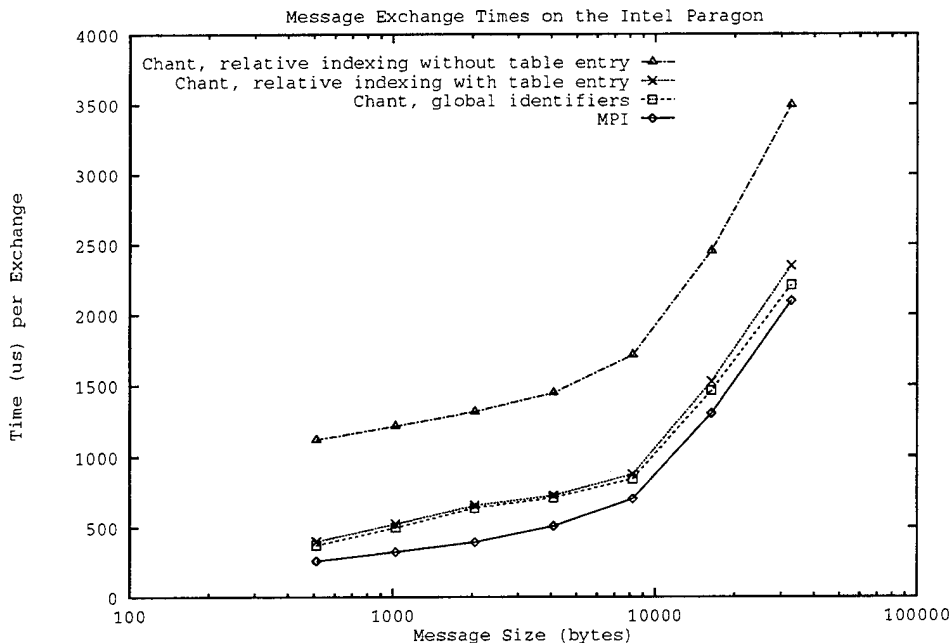
Figure 7: Execution times for point-to-point communication
