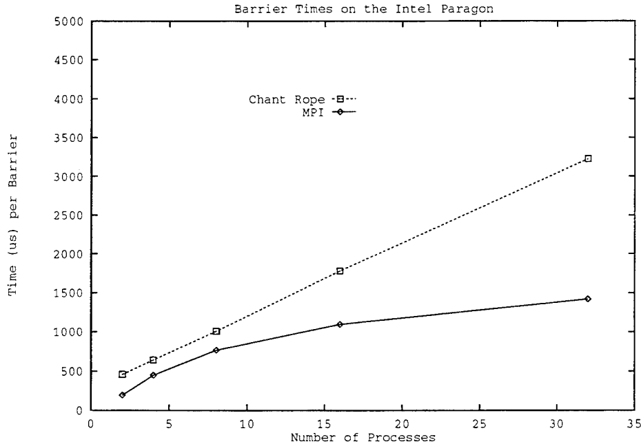
Figure 8: Execution times for barrier
