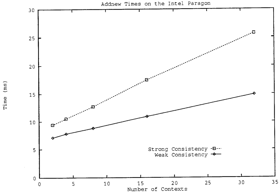
Figure 6: Execution times for rope_addnew, 4 threads per context
