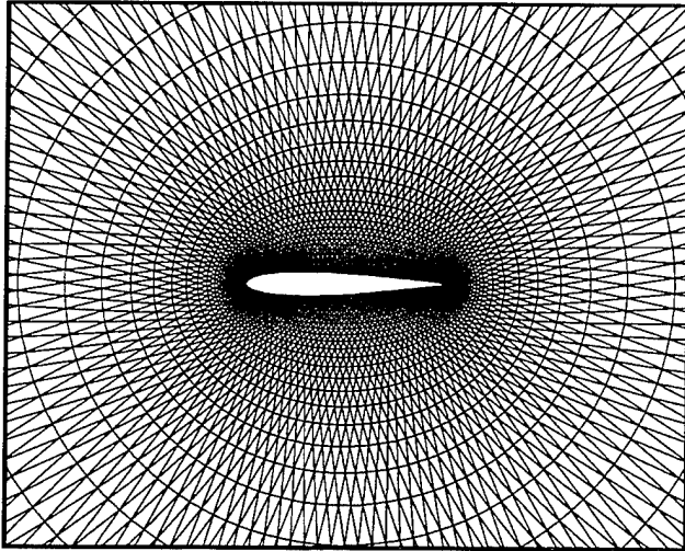
Figure 7: Grid about an NACA0012 airfoil with 4412 vertices.
