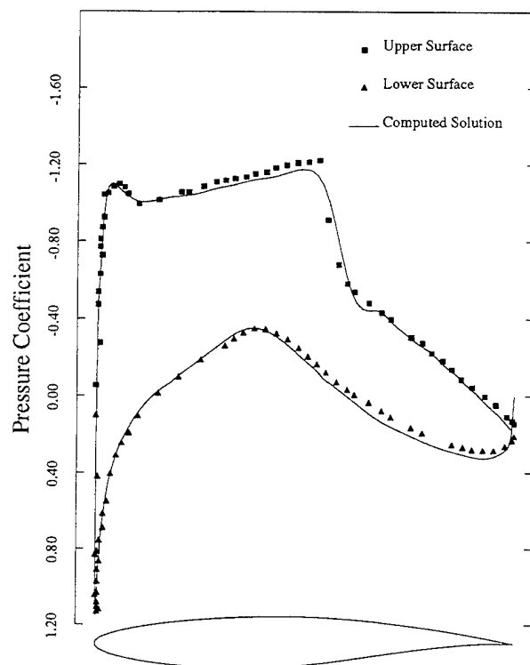
Figure 12: Computed surface pressure distribution for Case 6 ( M_\infty = 0.729 , \alpha = 2.31^\circ ) and Reynolds number = 6.5 \times 10^6 .
