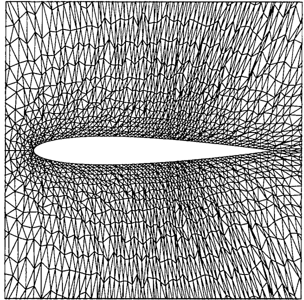
Figure 21: GRID2 about an NACA0012 airfoil with 6336 vertices.
