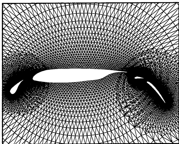
Figure 9: Grid about a four-element airfoil with 10395 vertices.
