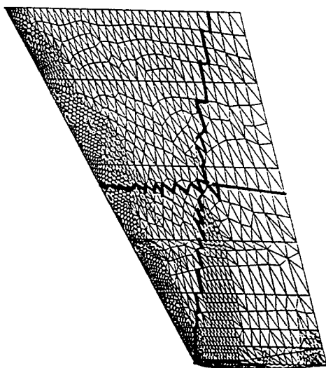
Figure 39(a): Adapted grid with the initial partitioning.
