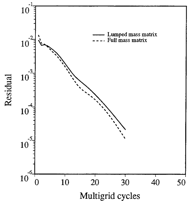
Figure 23: Histories of the unsteady residual at a particular time step.
