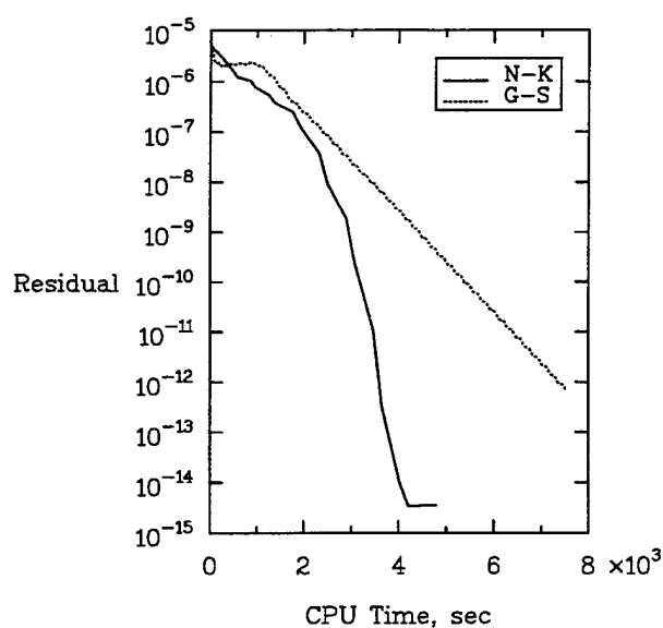
Figure 16(b): Convergence histories of the Newton-Krylov and multi-color Gauss-Seidel techniques as a function of CPU time.
