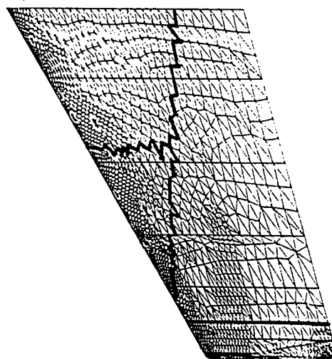
Figure 39(b): Partitions that result from applying the load balancing algorithm.
