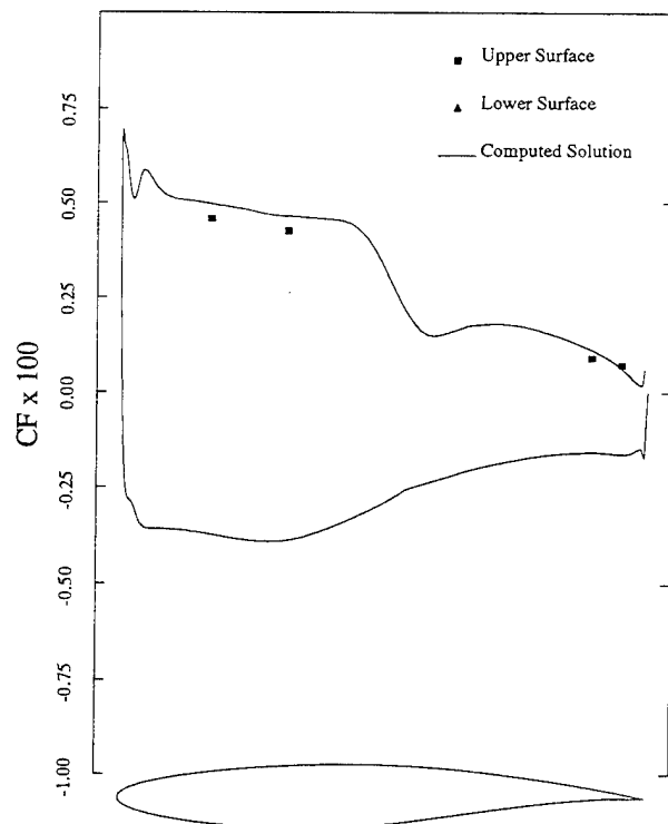
Figure 13: Skin friction distribution for Case 6.
