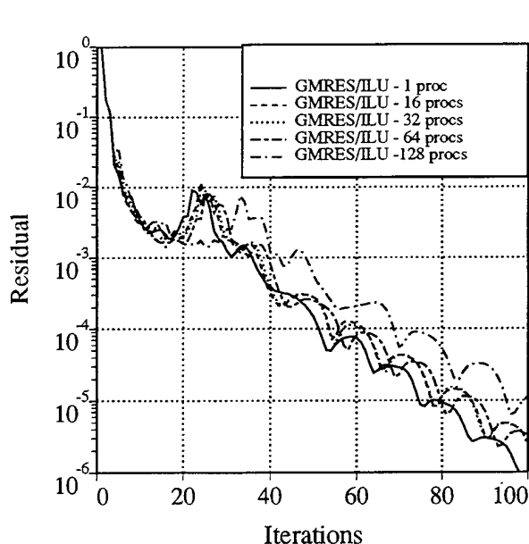
Figure 33: Convergence histories with GMRES/ILU on the fine mesh.
