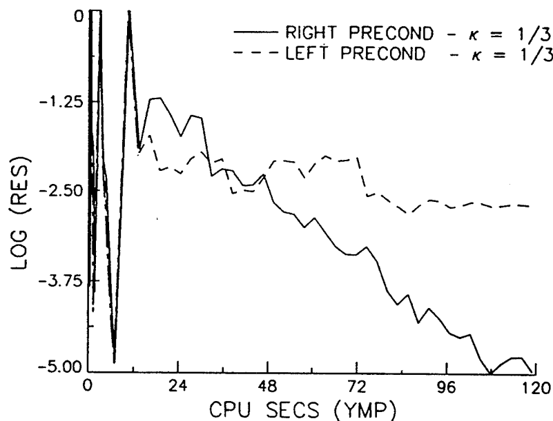
Figure 6: Convergence histories with left and right preconditioning for laminar viscous flow over an NACA0012 airfoil.
