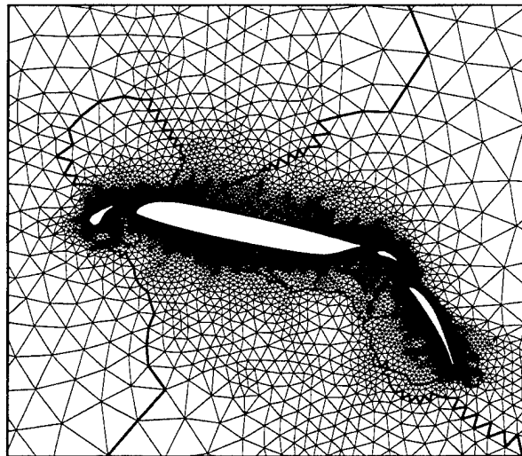
Figure 30(b): 8-way decomposition with graph bisection using level sets. processors.
