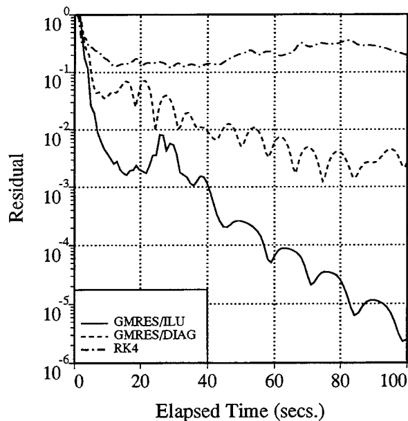
Figure 34: Convergence histories as a function of elapsed times on the fine mesh with 64 processors.
