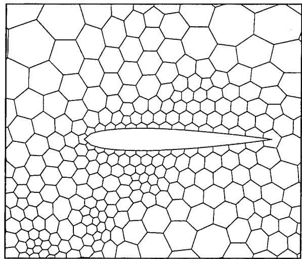
Figure 29: Dual graph.
