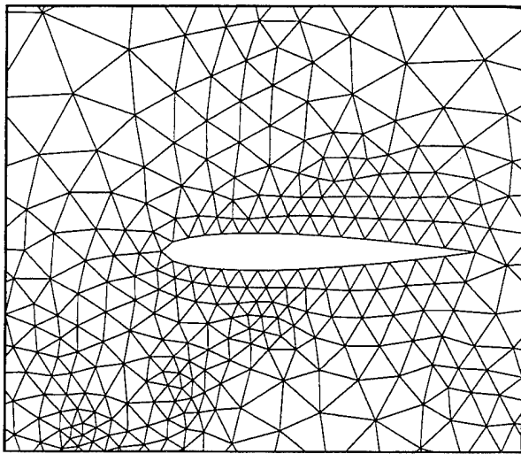
Figure 28: A triangulation.
