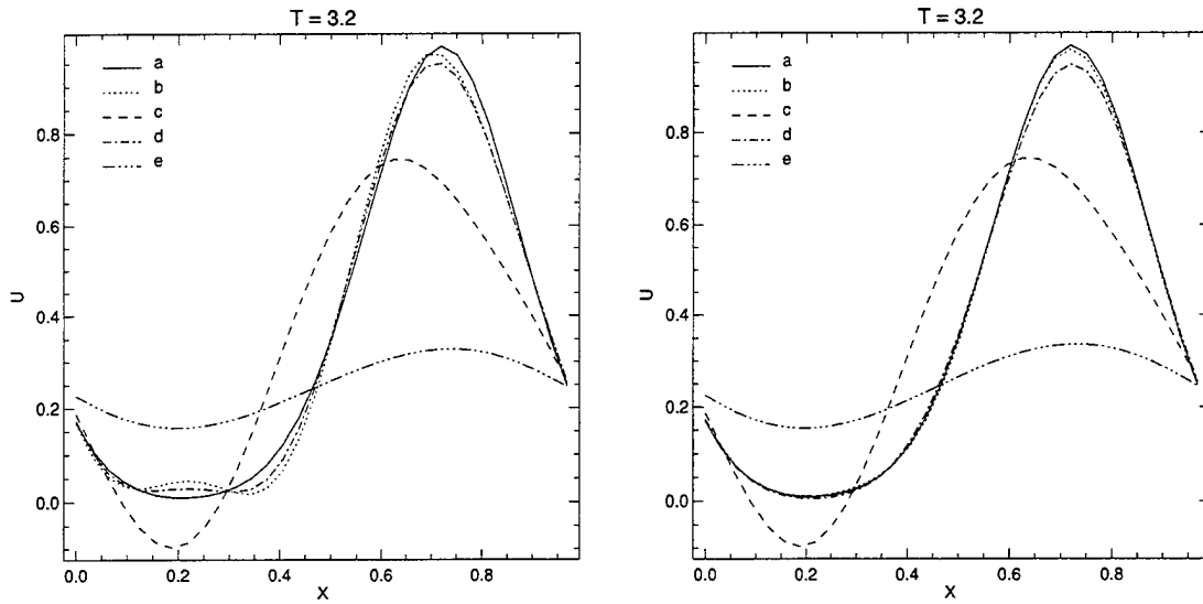
Figure 10: Solution of u_t + (1 + 0.3 \sin(2\pi x))u_x + 0.3(1 + 0.4 \cos(2\pi y))u_y = 0 , with u_0 = e^{-20(x^2 + y^2)} . Left : (a) the fine grid solution (b) the LDS( d = 1, \gamma = 20 ) solution when using quintic interpolation (c) coarse grid solution (d) the LDS( d = 1, \gamma = 20 ) solution when using cubic interpolation (e) the LDS( d = 1, \gamma = 20 ) solution when using linear interpolation. Right : (a) the fine grid solution (b) the LDS( d = 2, \gamma = 20 ) solution when using quintic interpolation (c) coarse grid solution (d) the LDS( d = 2, \gamma = 20 ) solution when using cubic interpolation (e) the LDS( d = 2, \gamma = 20 ) solution when using linear interpolation.
