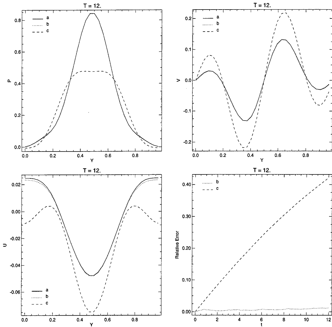
Figure 15: The acoustics equation on periodic domain, with initial data p_0 = e^{-35(x^2+y^2)} , u_0 = 0 , v_0 = 0 . In the plots of the solutions : (a) the fine grid solution (b) the LDS( d = 1, \gamma = 80 ) solution when adding sixth order dissipation (c) the coarse grid solution. In the plot of the relative error : (b) the relative error in the LDS( d = 1, \gamma = 80 ) solution (c) the relative error in the coarse grid solution.
