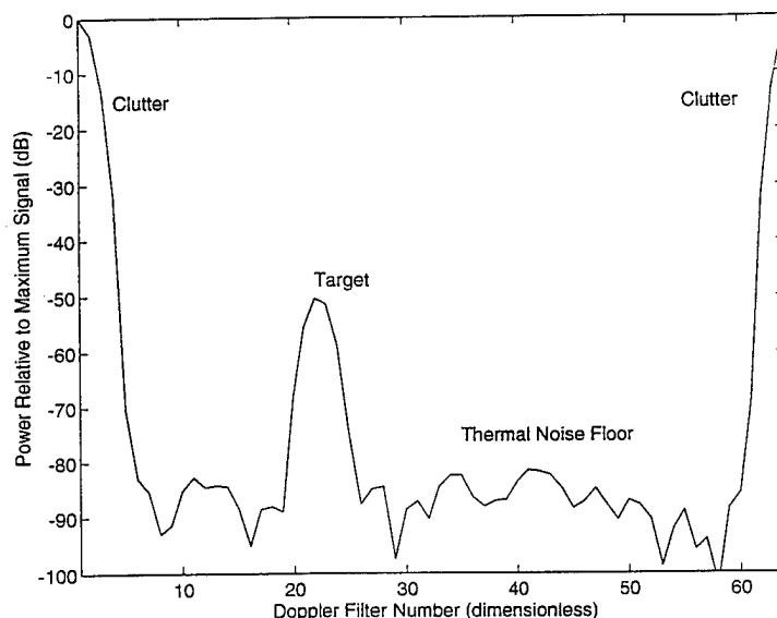
Fig. 3 — Single range cell of ambiguity diagram containing clutter, target, and thermal noise
