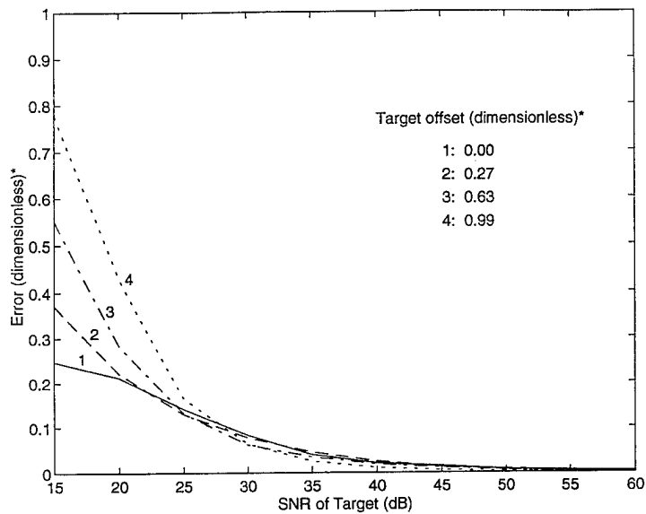
Fig. 8 — RMS error of azimuth estimate. These four curves have been extracted from Fig. 7 and plotted here for further clarity. (*Target offset and error are measured in fractions of a one-way 3 dB beamwidth.)
