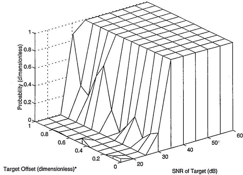
Fig. 11 — Probability that the error is less than 0.3 of a 3 dB beamwidth (*measured in fractions of a 3 dB beamwidth)
