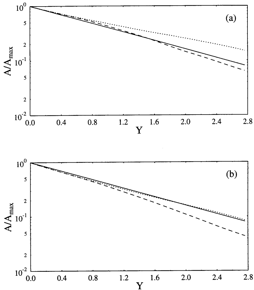
Figure 12: The decay rates of the wave amplitude across the channel in a rotating channel with \beta = 0.6 . (a) over a constant depth; (b) over a 2-D shelf. - - -, in the plane perpendicular to the right-hand sidewall; \cdots , along the curved wave crest; —, predicted by the linear theory.
