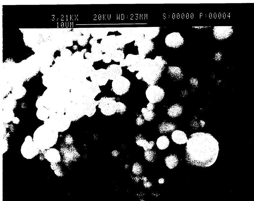
Figure 19. Scanning Electron Microscope Pictures of \text{Al}_2\text{O}_3 Collected in the Probe.
