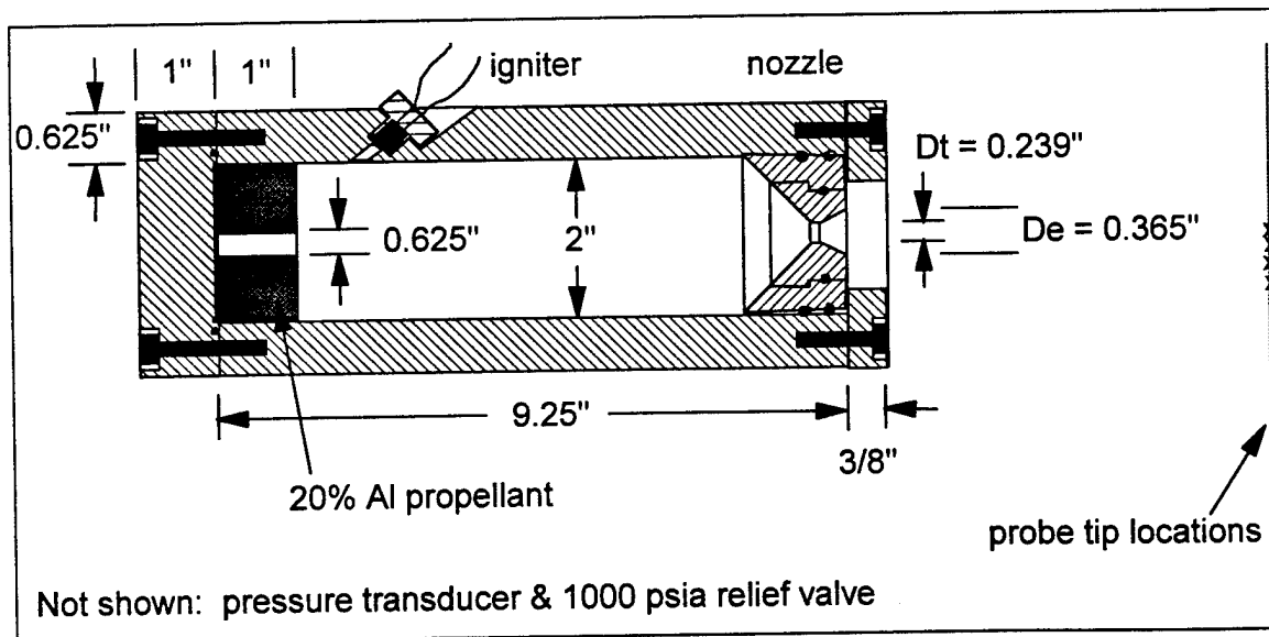
Figure 5. Sub-Scale Motor.
