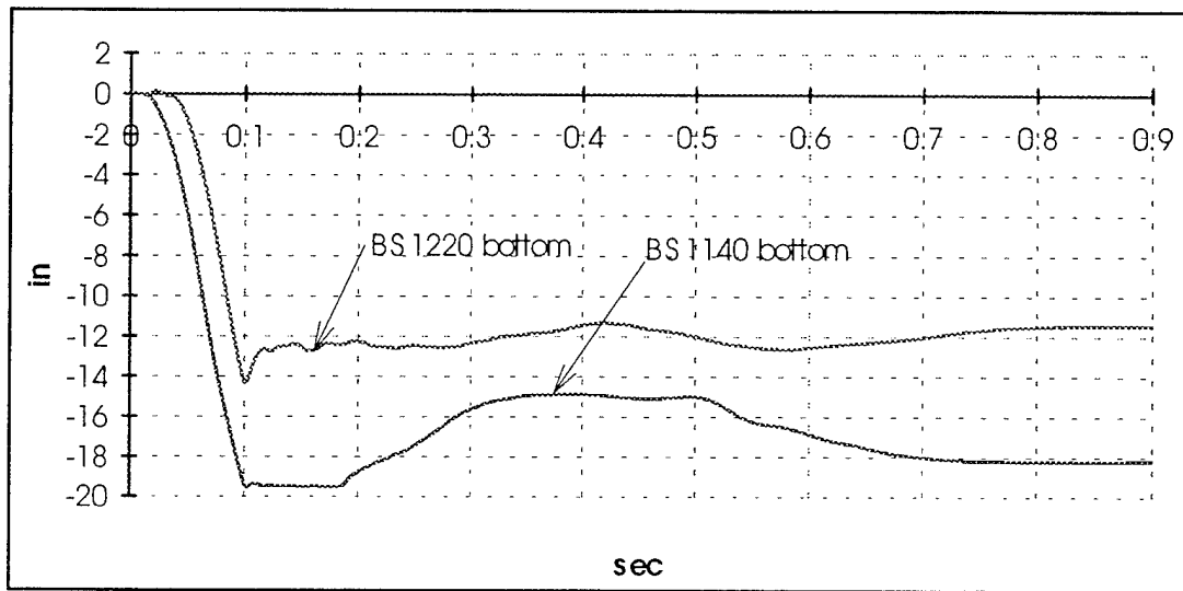
FIGURE 21. FUSELAGE DEFORMATIONS
