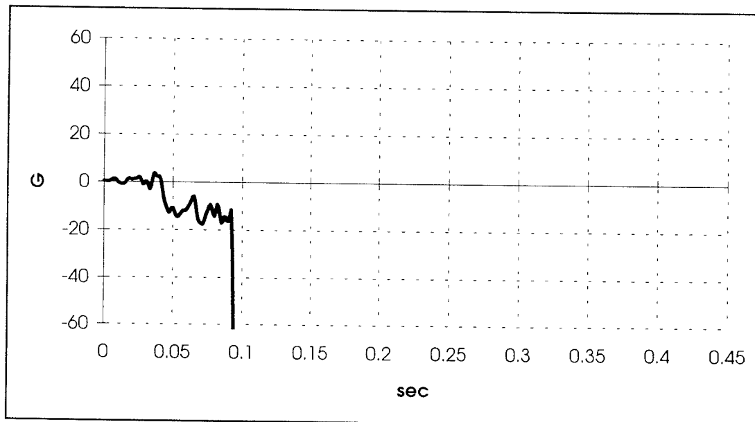
FIGURE A-40: BS1240 C&D VERTICAL ACCELERATION
