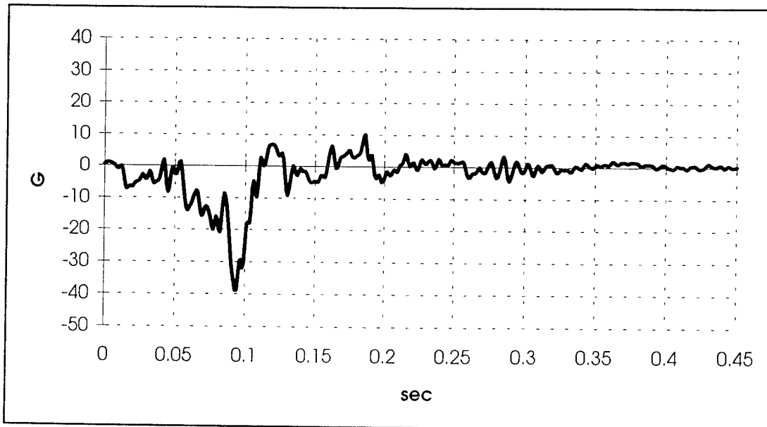
FIGURE A-3: BS1180 TOP PORT VERTICAL ACCELERATION
