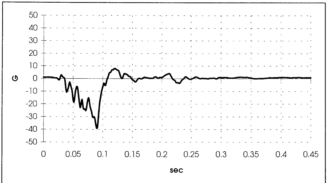
FIGURE A-67: TANK REAR STARBOARD VERTICAL ACCELERATION
