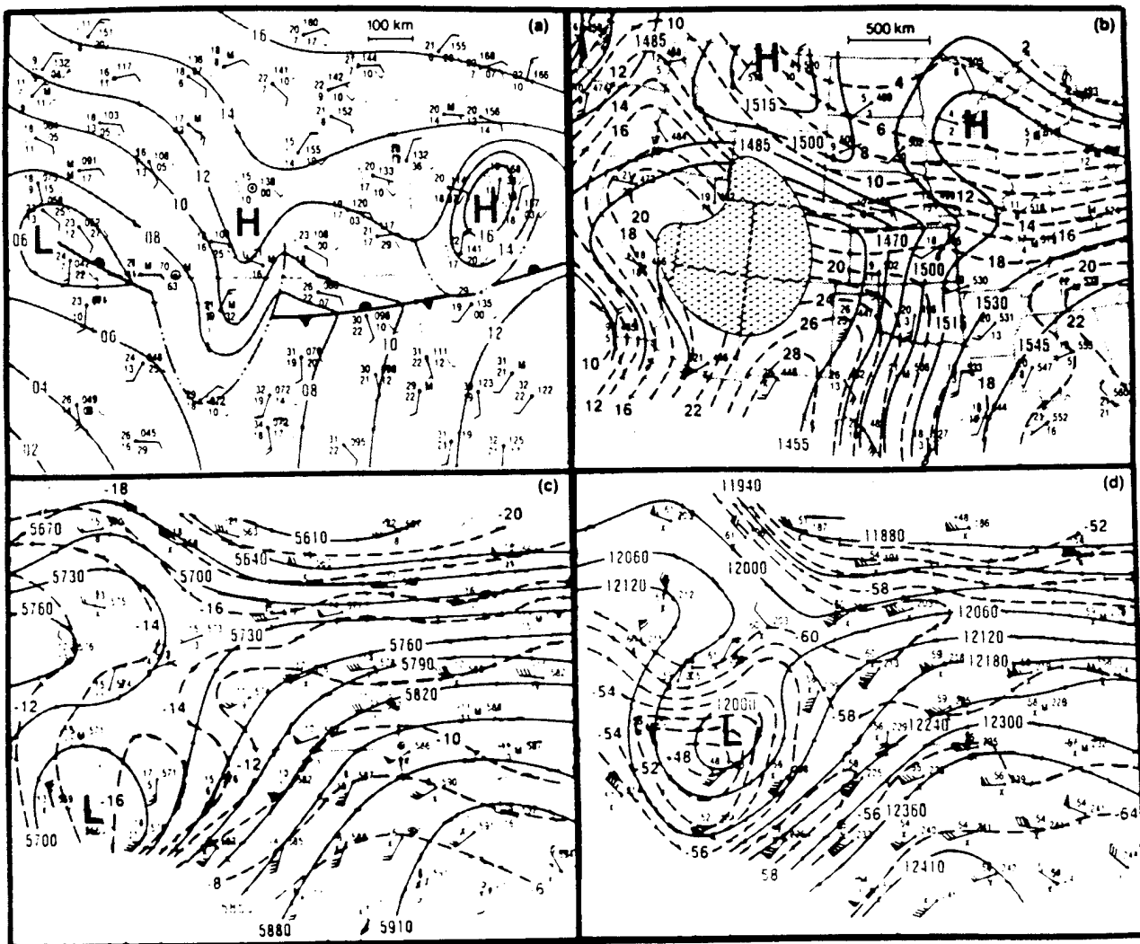
Synoptic-scale analyses at 0000 UTC 4 June 1985 at (a) surface, (b) 850 mb, (c) 500 mb, and (d) 200 mb. Isotherms (°C) are dashed in (b)-(d); solid contours represent mean sea level pressure (mb, leading "10" omitted) in (a), geopotential height (m MSL) in (b)-(d). Horizontal scale in (b) applies to (b)-(d).
