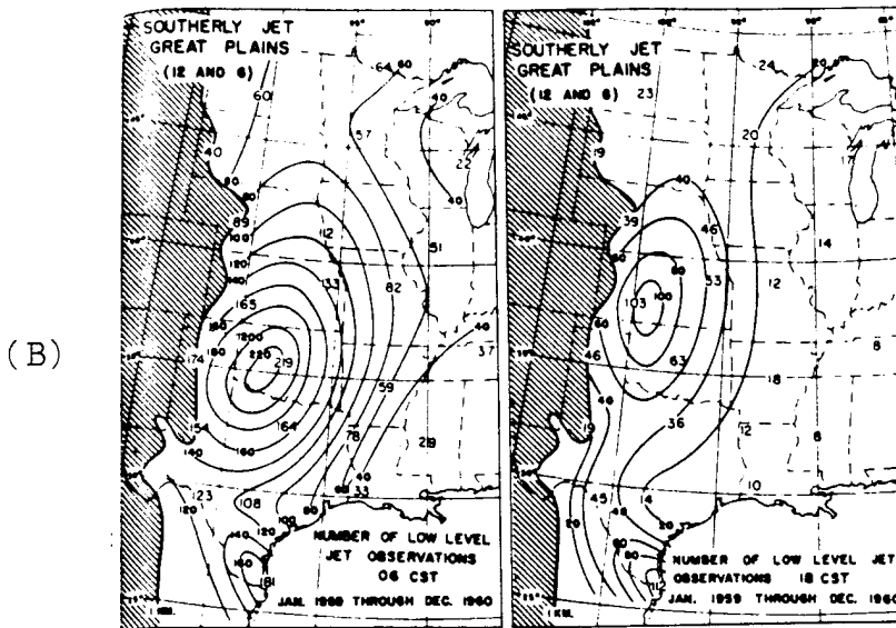
Numbers of Criterion 1 "southerly jet" observations at 06 csr (left) and 18 csr (right). Two years of data.
