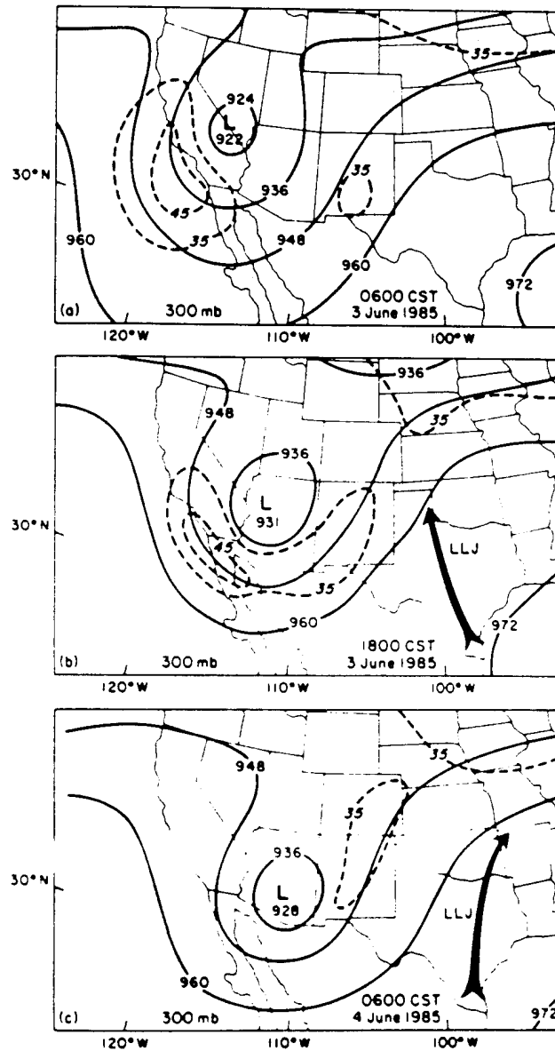
300-mb analysis with geopotential height contours (solid) analyzed in 12-dam intervals with the 35 and 45 \text{m s}^{-1} isotachs (dashed) at (a) 0600 CST 3 June, (b) 1800 CST 3 June, and (c) 0600 CST 4 June 1985. The bold arrow schematically illustrates the approximate streamline of the low-level jet in (b) and (c).
