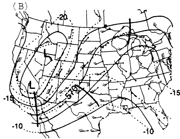
Upper-air analyses at 0000 UTC 12 May
