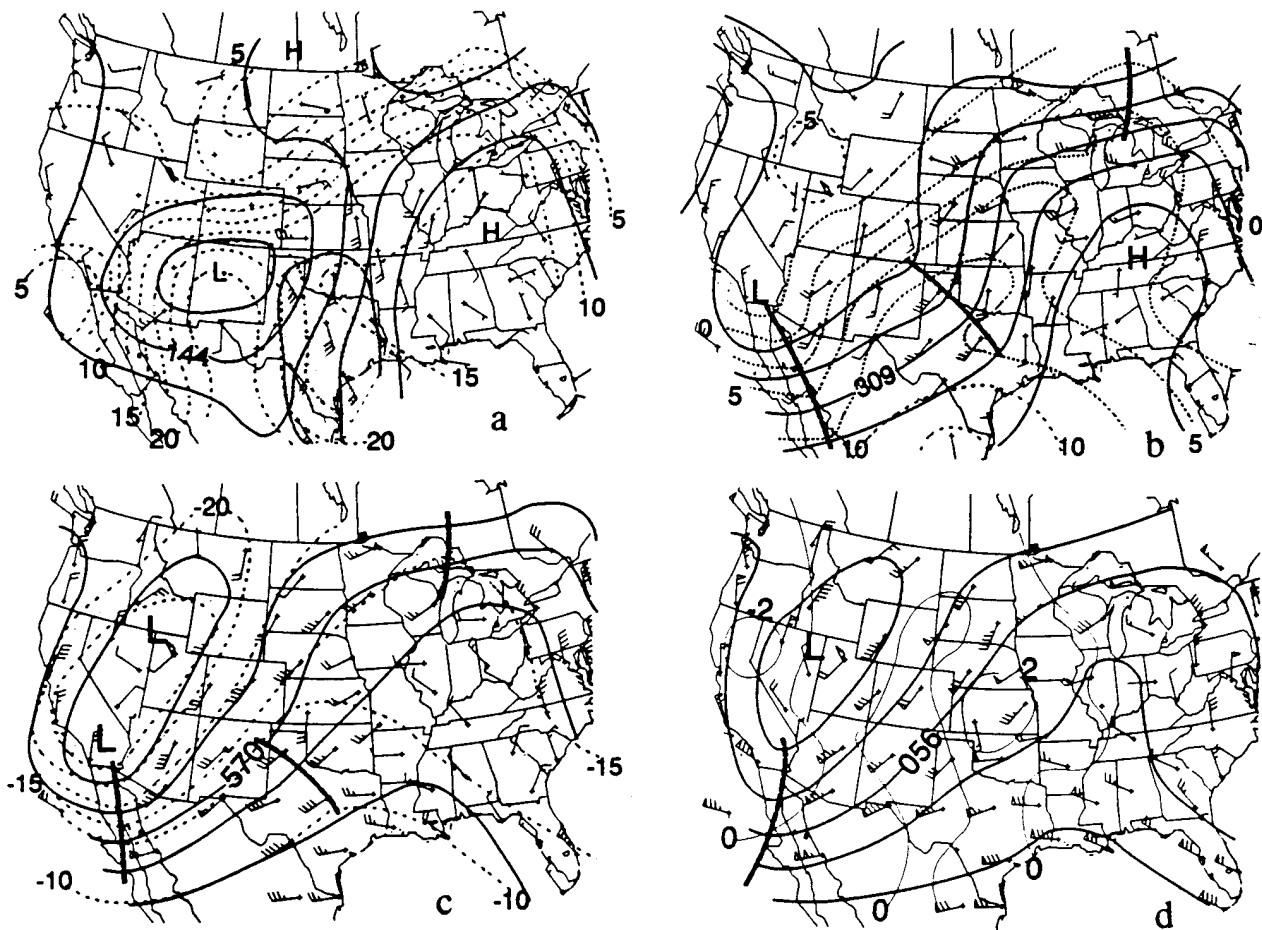
Upper-air analyses at 0000 UTC 12 May for (a) 850 mb, (b) 700 mb, (c) 500 mb, and (d) 250 mb. Winds are in knots. Solid lines denote geopotential height contours, dotted lines denote temperature contours ( ^{\circ}\text{C} ), and thick dashed lines denote short-wave positions. Stippled region in (a) denotes mixing ratios greater than 10 \text{ g kg}^{-1} . Thin solid line in (d) denotes divergence contours in units of 10^{-3} \text{ s}^{-1} . Height contours at 30-m intervals at 850 and 700 mb, 60 m at 500 mb, and 120 m at 250 mb.
