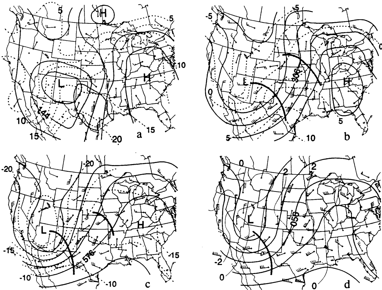
Upper-air analyses at 1200 UTC 12 May for (a) 850 mb, (b) 700 mb, (c) 500 mb, and (d) 250 mb. Winds are in knots. Solid lines denote geopotential height contours, dotted lines denote temperature contours ( ^{\circ}\text{C} ), and thick dashed lines denote short-wave positions. A shaded region in (a) denotes mixing ratios greater than 10 \text{ g kg}^{-1} . Thin solid line in (d) denotes divergence contours in units of 10^{-5} \text{ s}^{-1} . Contours at 30-m intervals at 850 and 700 mb, 60 m at 500 mb, and 120 m at 250 mb.
