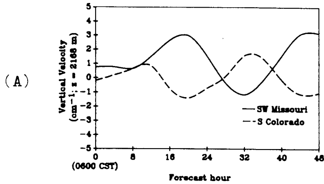
Vertical velocity forecast ( \text{cm s}^{-1} ) at 2168 m for grid points in southwest Missouri (solid) and southern Colorado (dashed) for the dry soil case.
