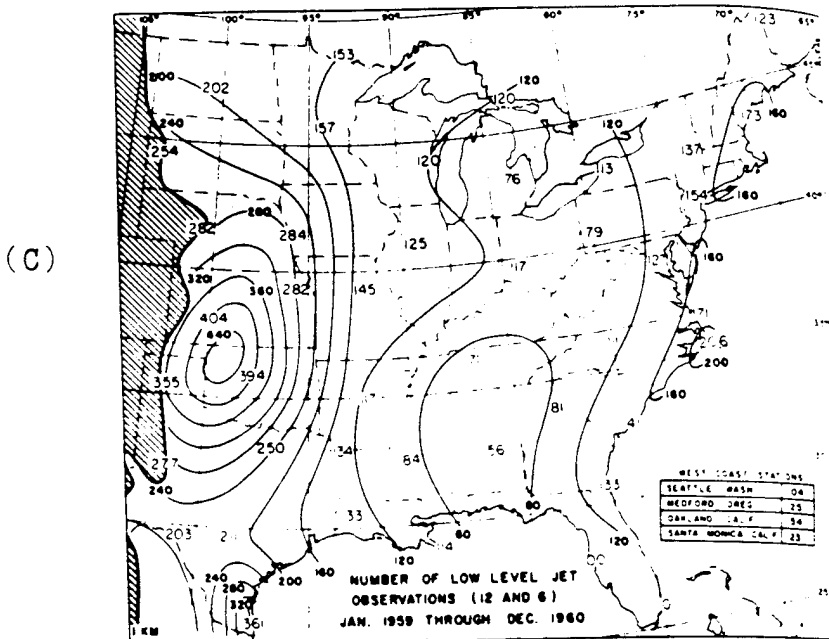
Number of Criterion 1 low level jet observations from January 1959 through December 1960. 18 csr and 06 csr combined.
