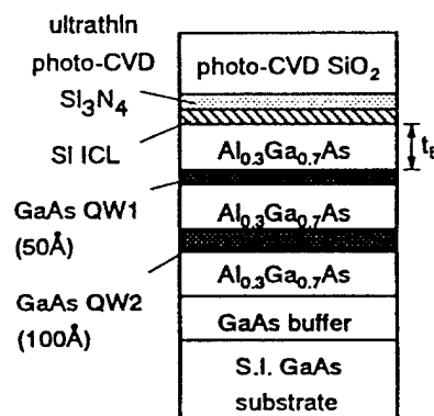
Fig.1 Sample structure
