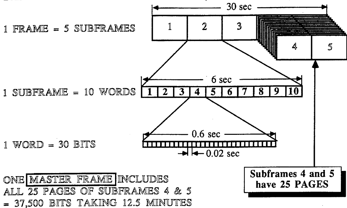
Figure 3.6 GPS Message Format
