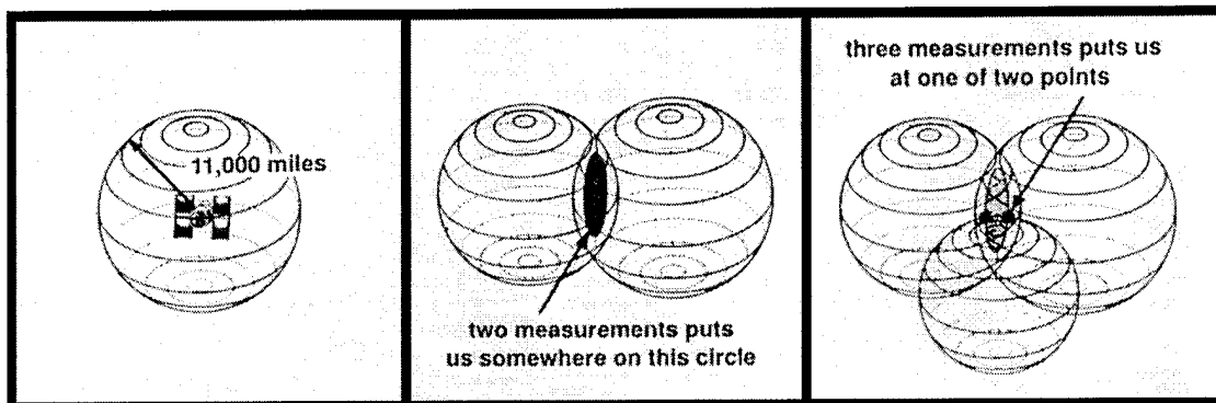
Figure 3.2 Satellite Ranging
