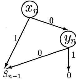
Figure 4: MTBDD for S_n
