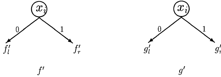
Figure 6: BDDs for f' and g'
