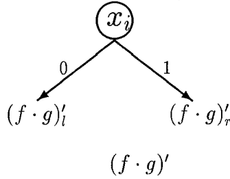
Figure 7: BDD of (f \cdot g)'
