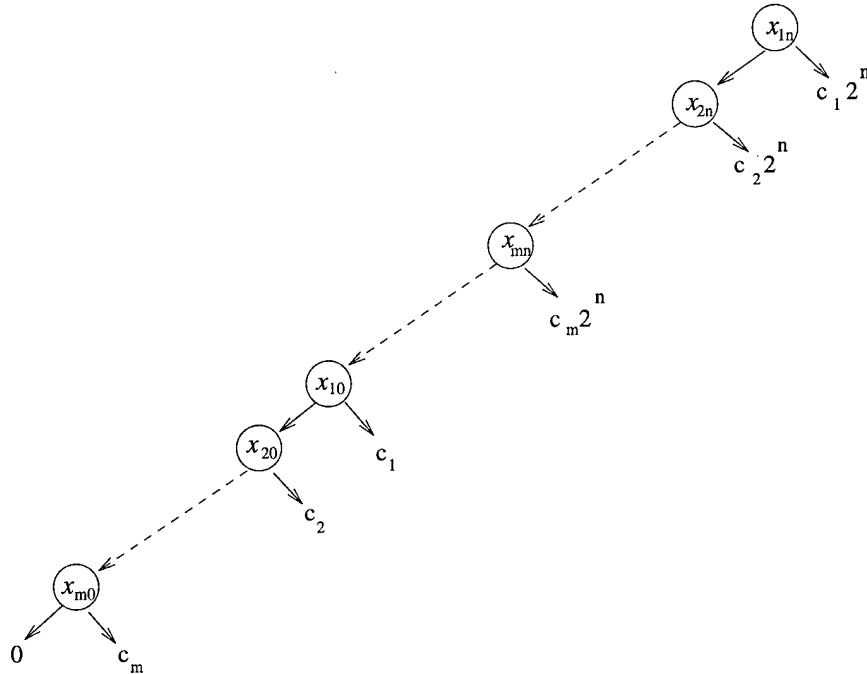
Figure 8: BMD for \sum_{i=1}^m c_i f_i
