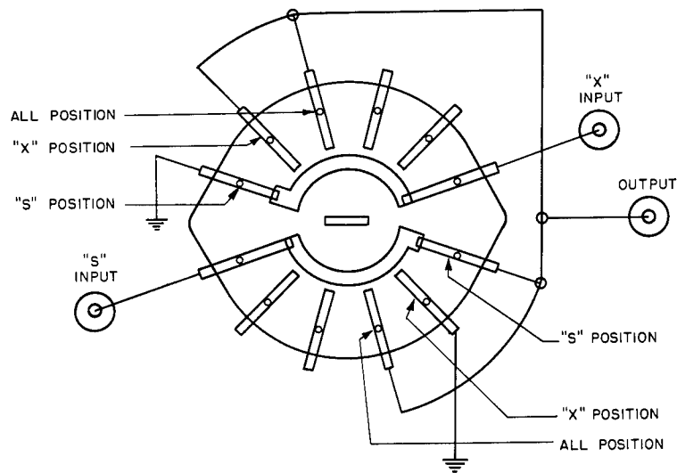
Fig. 30 - Improved band selector switch (for filter-crystal unit)
