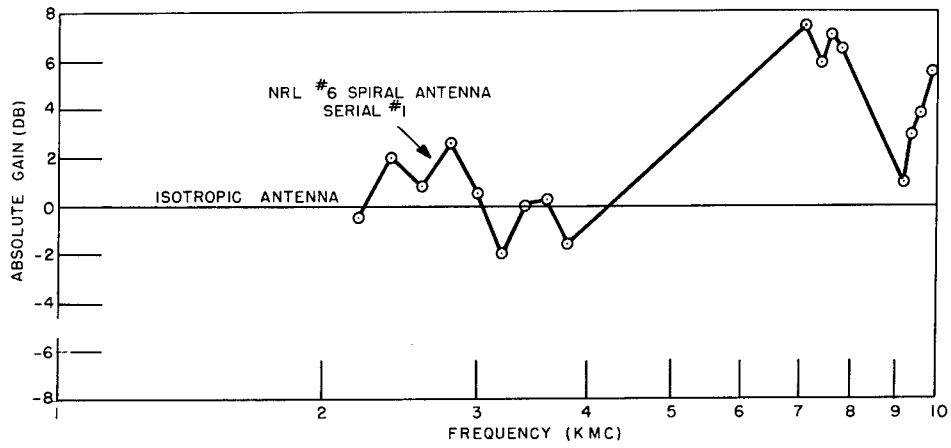
Fig. 15 - Spiral antenna -- Gain curve
