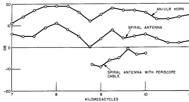
Fig. 17 - Spiral antenna vs horn -- Gain curves
