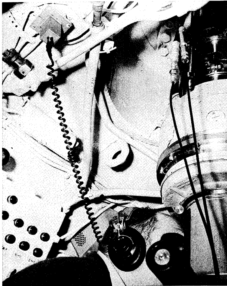
Fig. 4 - Submarine control compartment overhead showing cable runs
