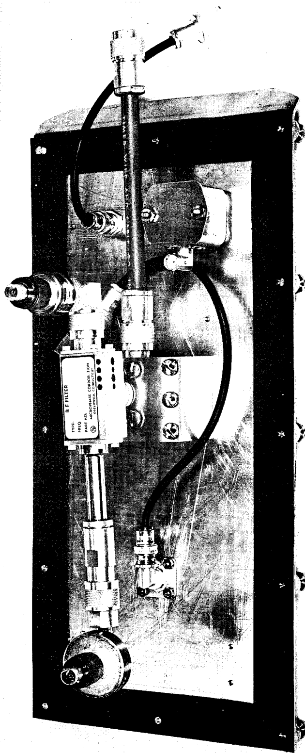
Fig. 22 - Filter-crystal unit -- Rear view
