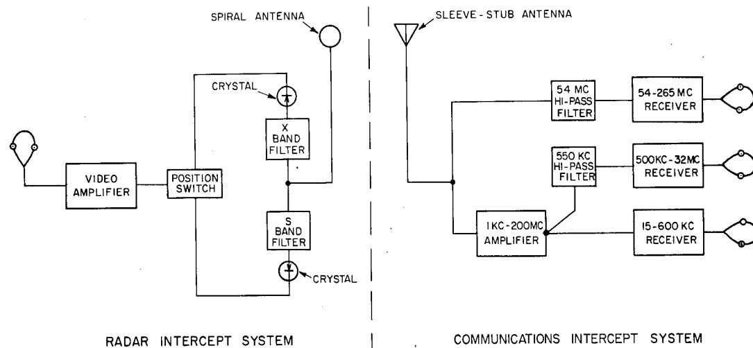
Fig. 1 - The complete intercept system -- Block Diagram
