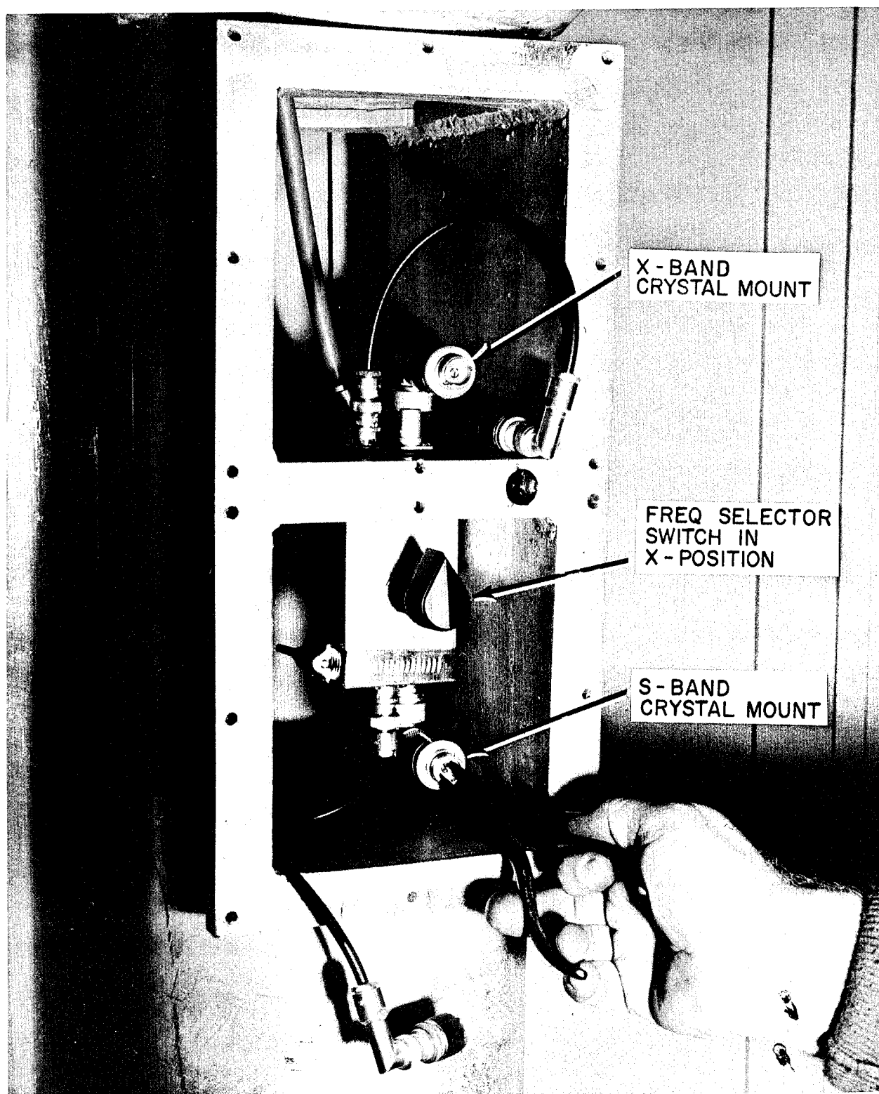
Fig. 23 - Filter-crystal unit -- Band selector switch mounting
