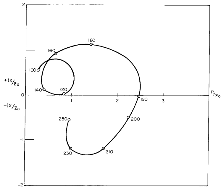
Fig. 29 - Improved sleeve-stub antenna impedance characteristics
