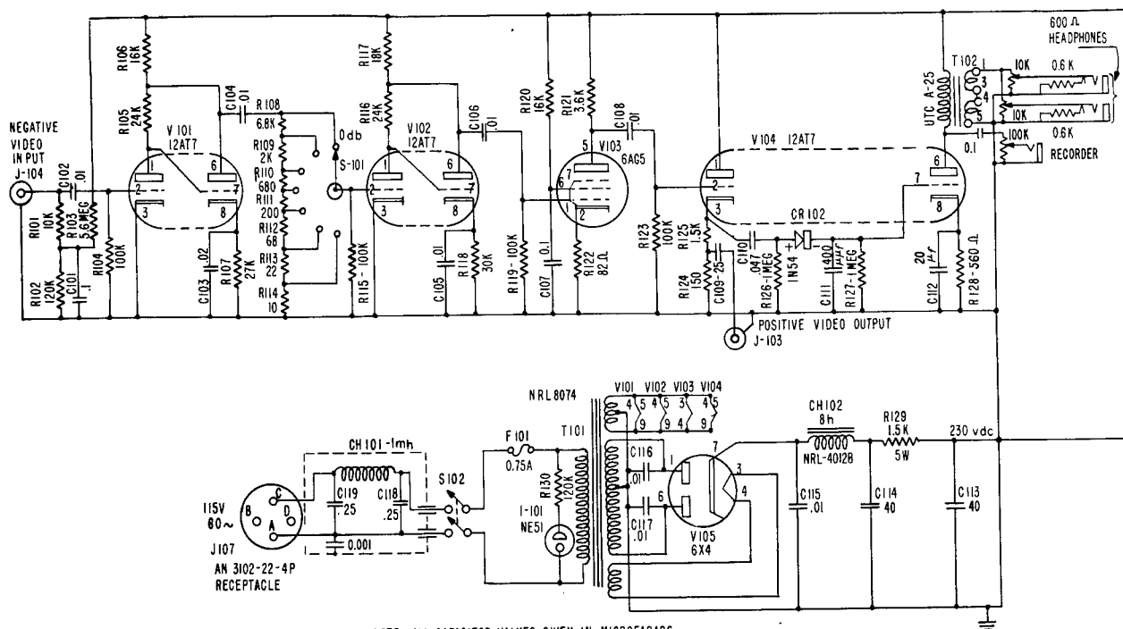
Fig. 27 - Video amplifier -- Schematic
