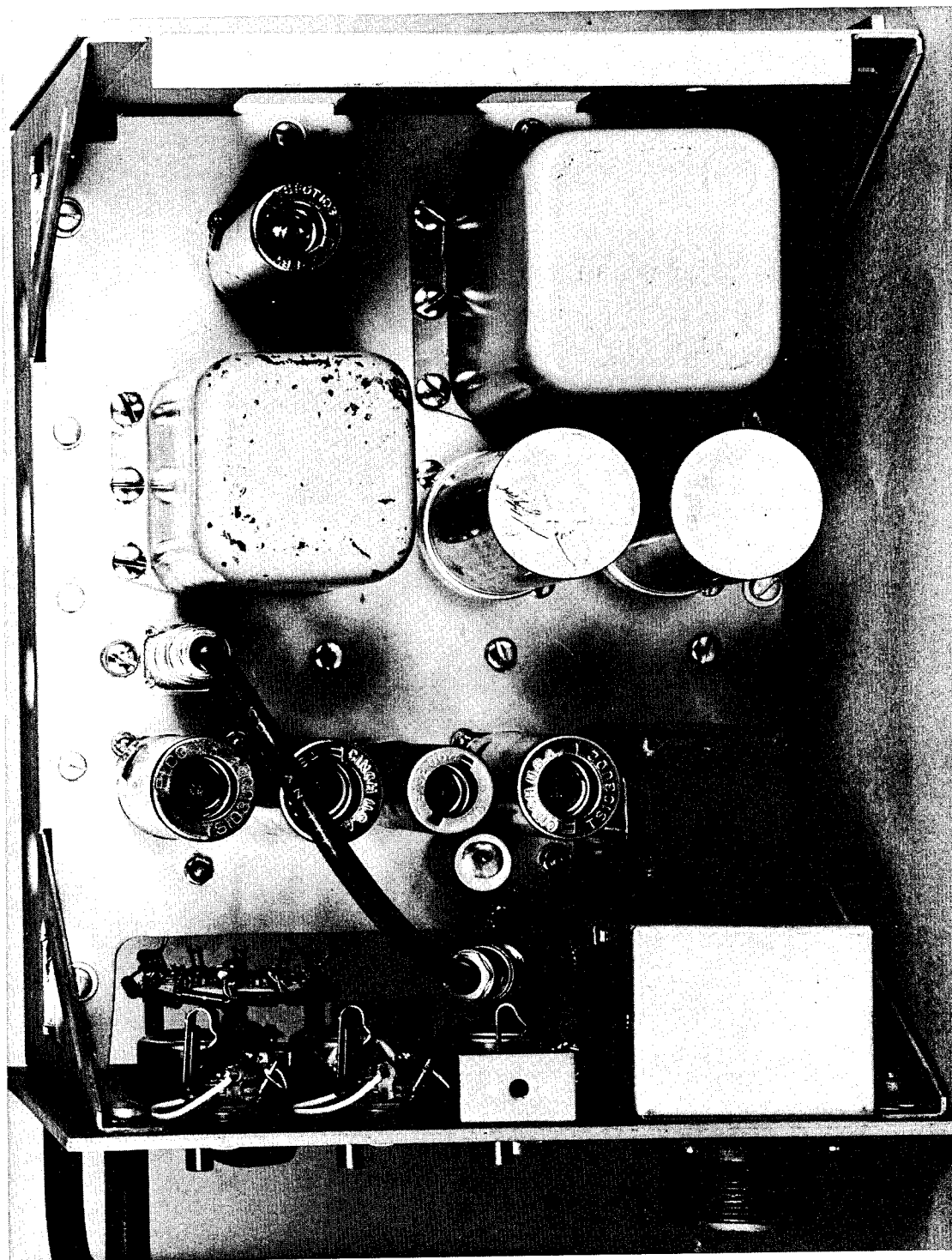
Fig. 25 - Video amplifier -- Top view
