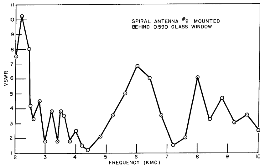
Fig. 16 - Spiral antenna - VSWR curve
