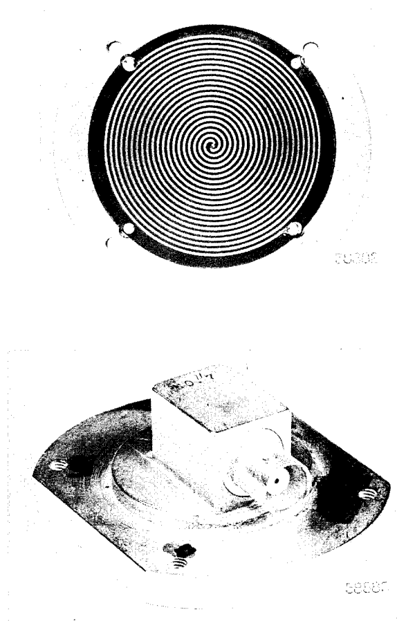
Fig. 14 - Spiral antenna — Front and side view
