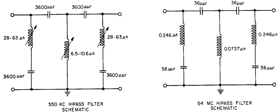
Fig. 8 - High-pass filters -- Schematics
