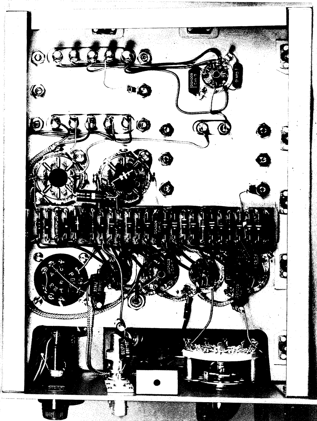
Fig. 26 - Video amplifier -- Bottom view
