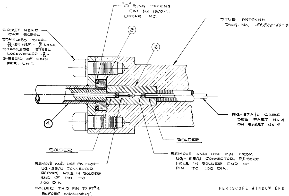
Fig. 7 - Antenna feed-line end fittings — Details
