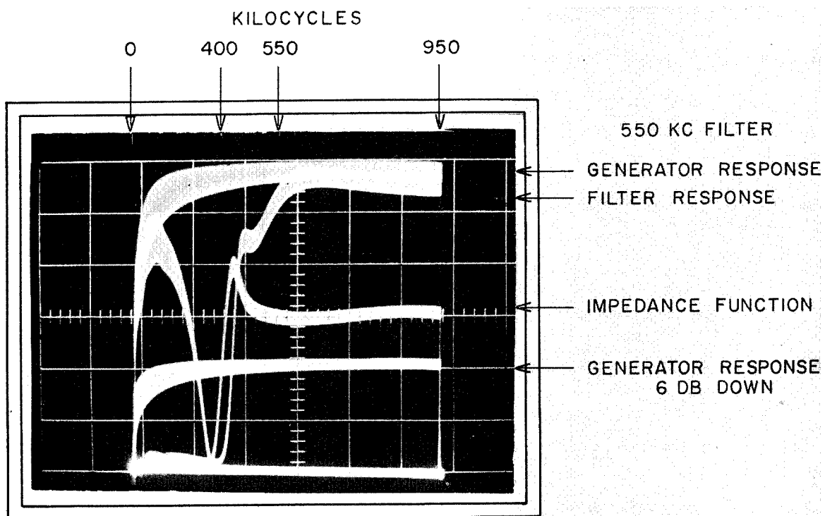
Fig. 11 - High-pass filters -- Characteristics
