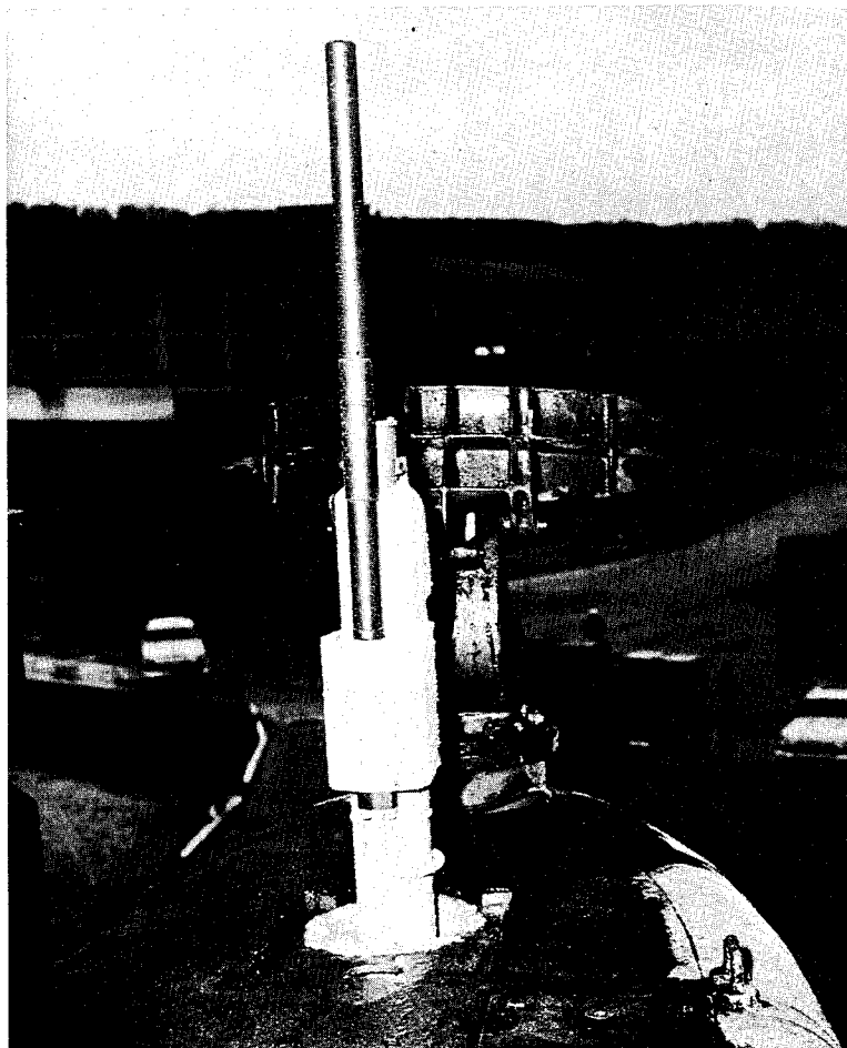
Fig. 2 - Sleeve-stub antenna mounted on periscope
