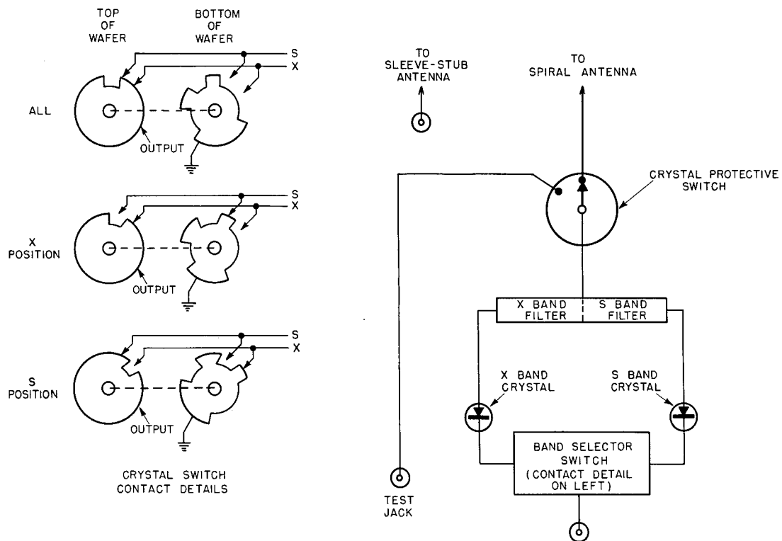
Fig. 19 - Filter-crystal unit -- Schematic
