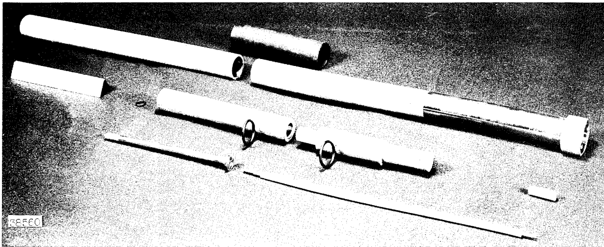
Fig. 28 - Improved sleeve-stub antenna -- Disassembled view
