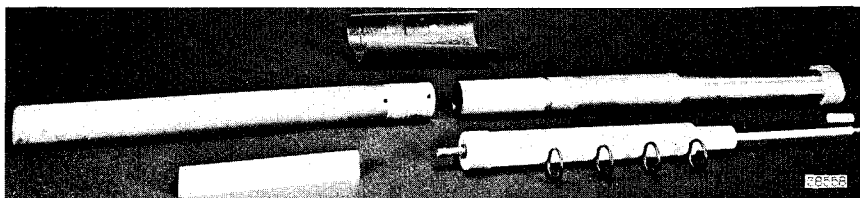
Fig. 6 - Sleeve-stub antenna -- Assembled and disassembled views
