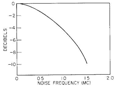
Fig. 1 - X-band video characteristics of a standard AN/ALT-2 with an internal modulator
