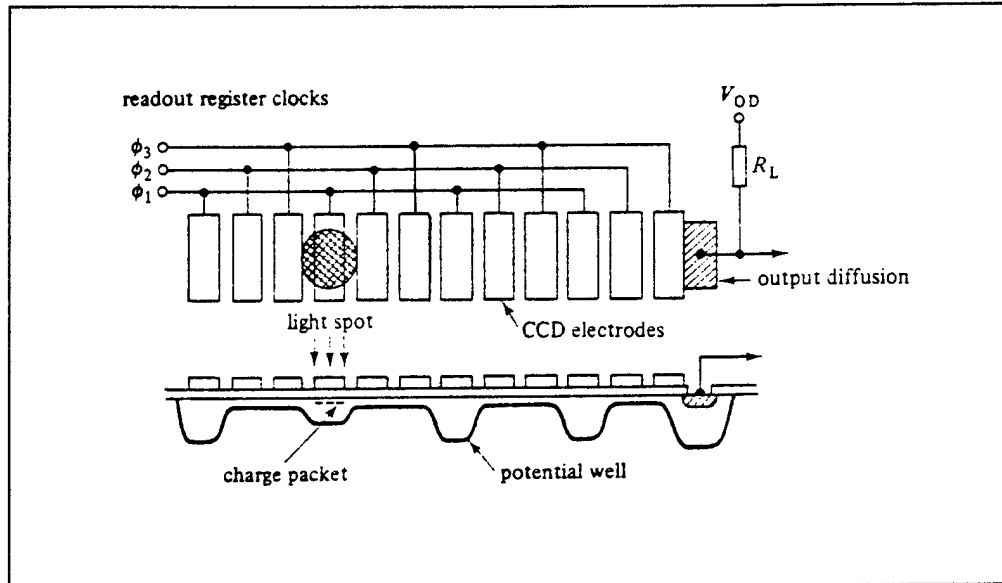
Figure 8. Basic Principal of CCD Imaging. From Ref. [6].
