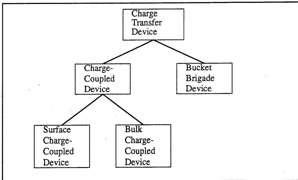
Figure 2. Family of Charge Transfer Devices
