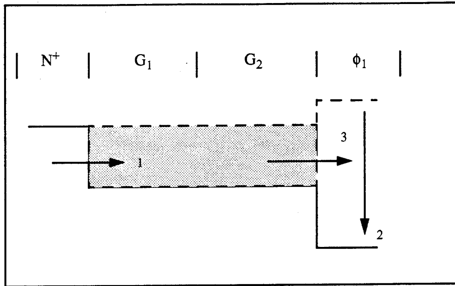
Figure 25. Pulsed Diffusion Input Technique. Modified from Ref. [11].
