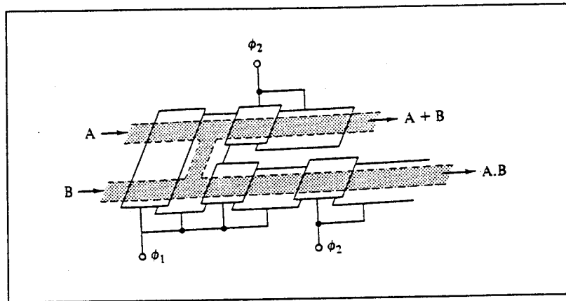
Figure 13. 2-Input OR/AND Gate Utilizing a Two-Phase CCD. From Ref. [6].
