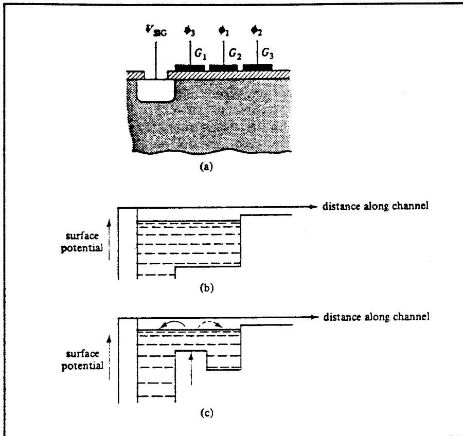
Figure 23. Diode Cut-Off Technique. From Ref. [6].
