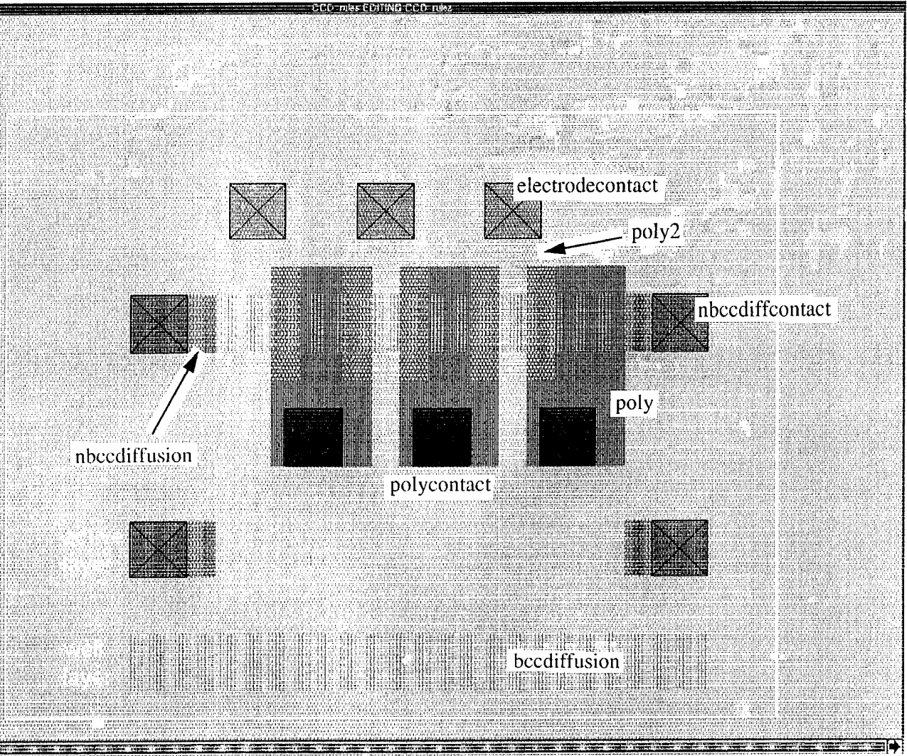
Figure 30. Magic Layout of a Buried-Channel Charge-Coupled Device.
