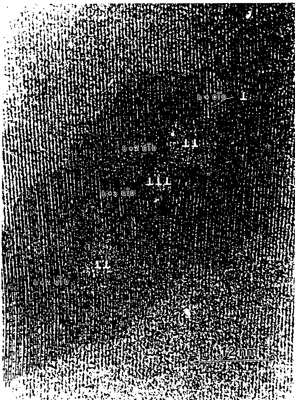
Figure 10: HREM image of a low angle tilt boundary in a DCHD droplet. The lattice fringes being imaged are the (010) planes with a spacing of 1.2 nm and correspond to the spacing between chains. The image has lines drawn to highlight the dislocations along the tilt boundary. The Burgers vector is [010] with a magnitude of 1.2 nm. Around the dislocations there is a region of crystal that the contrast does not give rise to lattice fringes, these areas measure from approximately 6nm to 36 nm. The angle of the tilt changes from 4° to 6° along the boundary. The distance between the imaged dislocations is approximately 7.0 to 12.0 nm.
