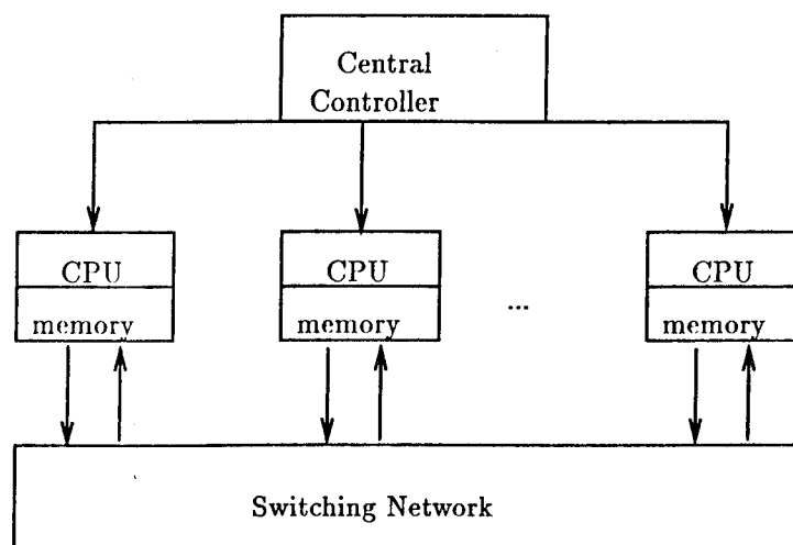
Figure 9: General Structure of a SIMD Array Architecture
