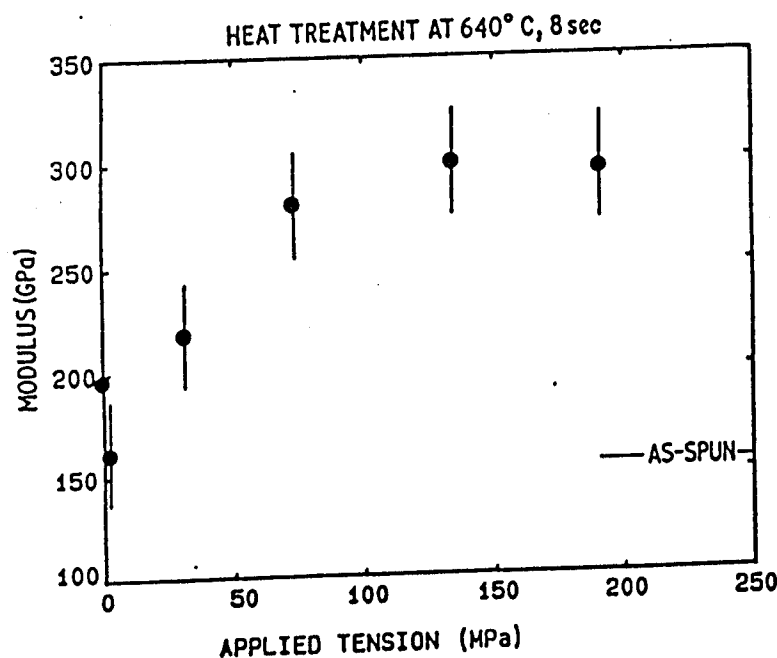
Figure 4 Modulus of 640°C, 8 sec tensioned heat-treated fibres.
