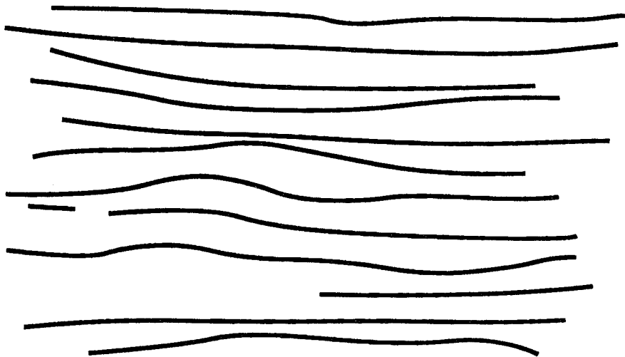
"Ideal" Polymer
