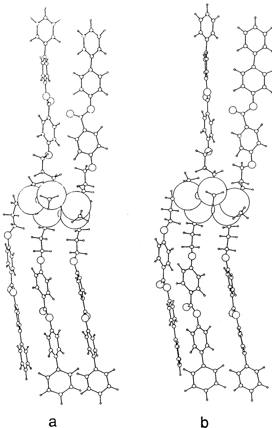
Figure 6: Two Different Projection of the Lowest Energy Molecular Structure After 50 picosecond Dynamics Simulation.
