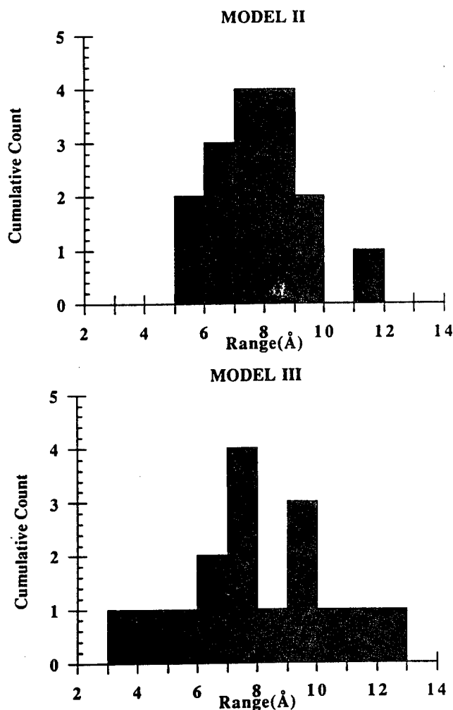
Figure 7. Cumulative count of \delta_i (as explained in the text; Å) during the dynamics simulation for the molecular systems II and III.
