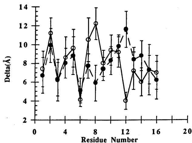
Figure 6. The \delta_i variations (as explained in the text) of side-chain-side-chain distances (Å) during the dynamics simulation for the molecular systems II—full circle and III—open circle.
