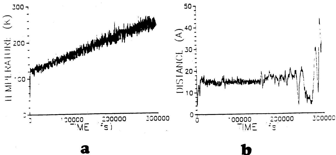
Figure 1.8 Plot of temperature (a) and intermolecular distance (b) versus simulation time for {B} pairs during MD simulation.
