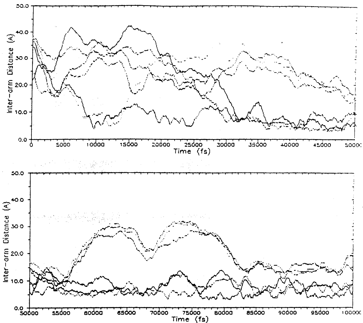
Figure 7. The distances between mesogens for the (4B) star as a function of time during the simulation, using the original force field: (top) from 0 to 50 ps and (bottom) from 50 to 100 ps.
