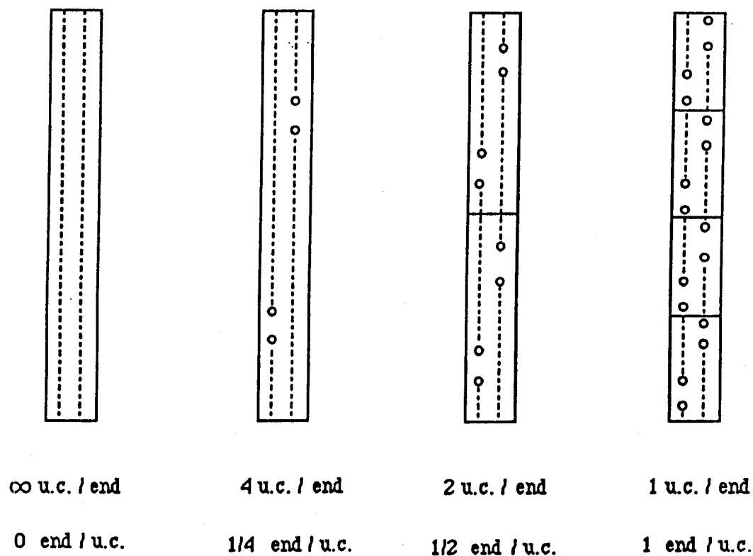
Figure 3: Proposed scheme for studying the influence of chain end defects. The route is similar to that used for investigating the twist defects. Here, it may be necessary to decrease the defect concentration enough to insure that it is possible for the molecules to interact with one another through frictional forces across their non-bonded lateral surfaces.
