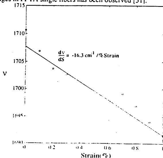
Figure 3: Change in 1711 \text{cm}^{-1} mode frequency of PPTA as a function of the percentage strain applied; the solid line denotes a linear fit
