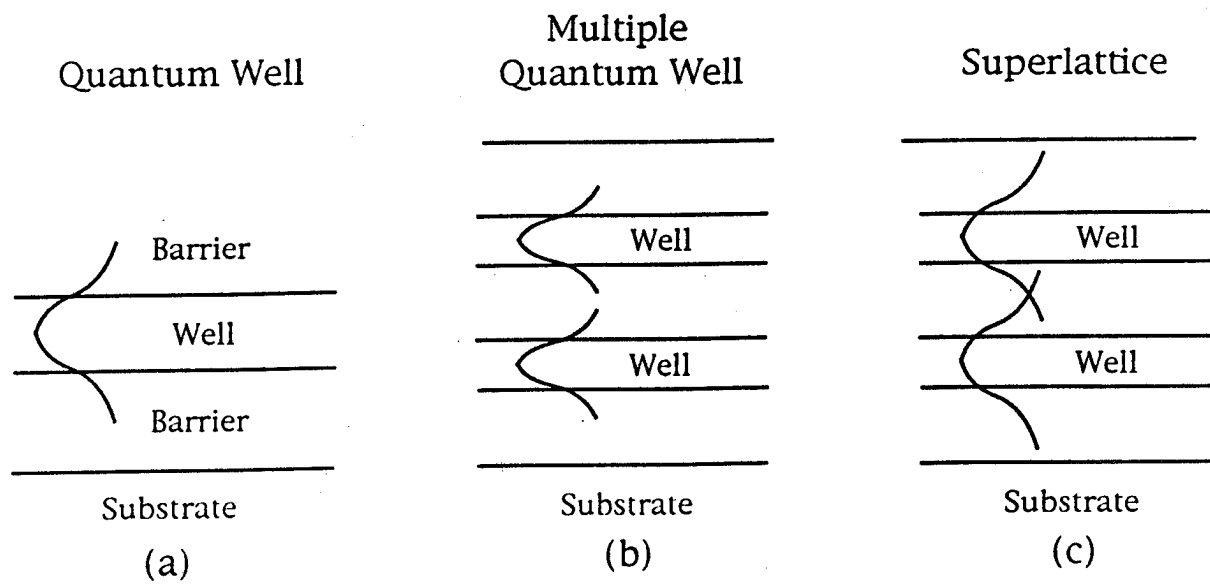
Figure 1. Quantum effect devices. The wave functions of the confined carrier must overlap for a superlattice.
