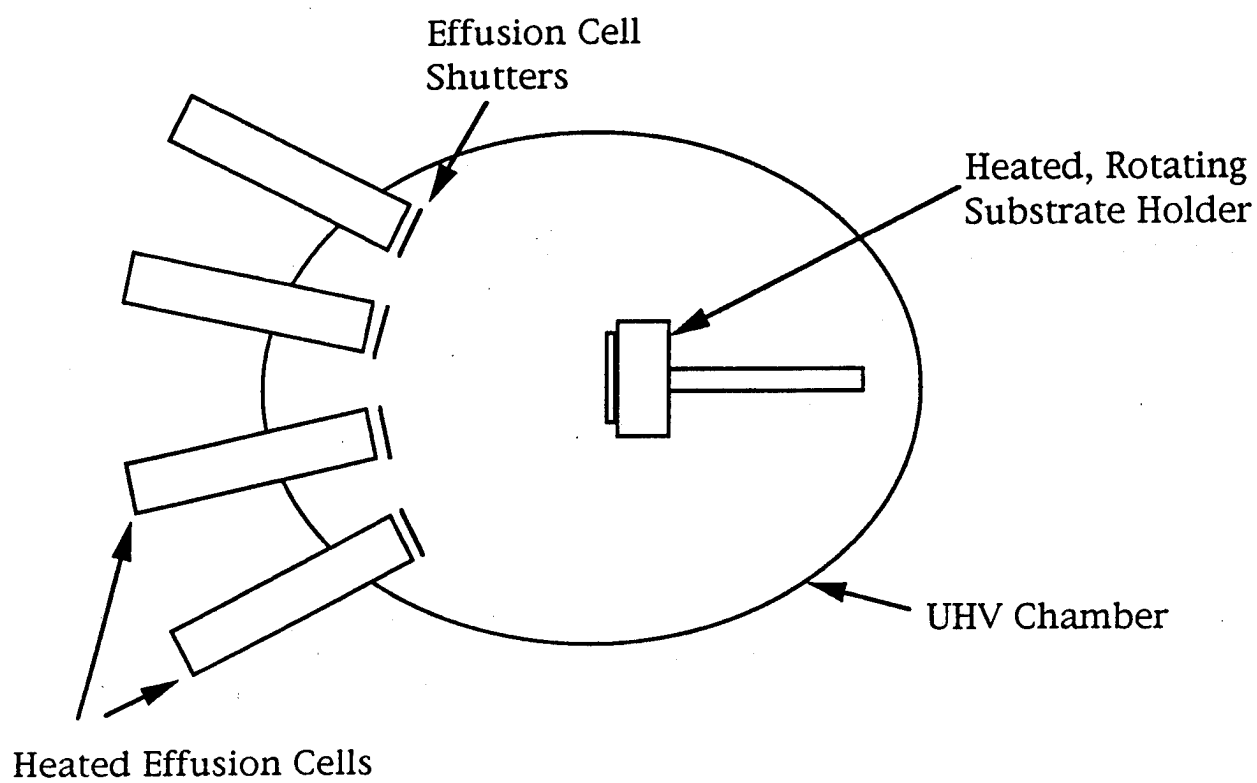
Figure 2. Diagram of the molecular beam epitaxy process.
