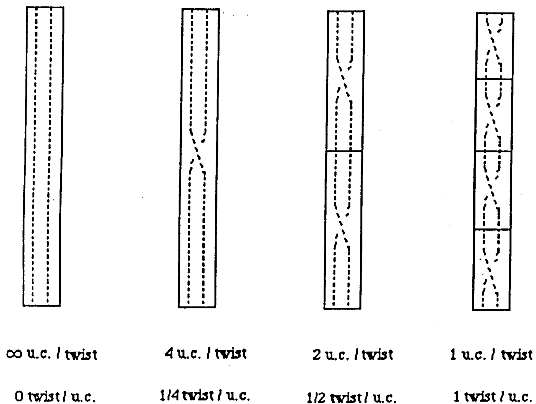
Figure 1: We have shown that it is possible to investigate intermolecular twist defects in extended polymer chains by creating a periodic two-chain simulation and connected the end of chain 1 to the head of chain 2 and vice versa. The defect density can be altered by increasing the length of simulation in the chain direction. As the number of unit cells per defect increases, the defect density decreases, eventually reaching the non-defective case as a limit.
