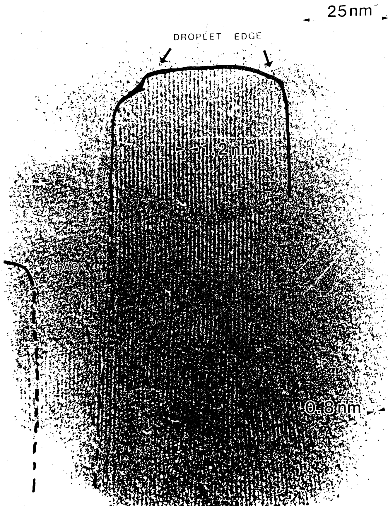
Figure 6: HREM image of the edge of a poly(DCHD) droplet with the edge perpendicular to the chain axis. There are two different orientations of the polymer chains visible, one with a spacing of 1.2 nm (010) and one with a spacing of 0.8 nm (200). A 0.6 nm fringe region stretching across the droplet in the middle of the image is believed to indicate a thickness of 100 nm.
