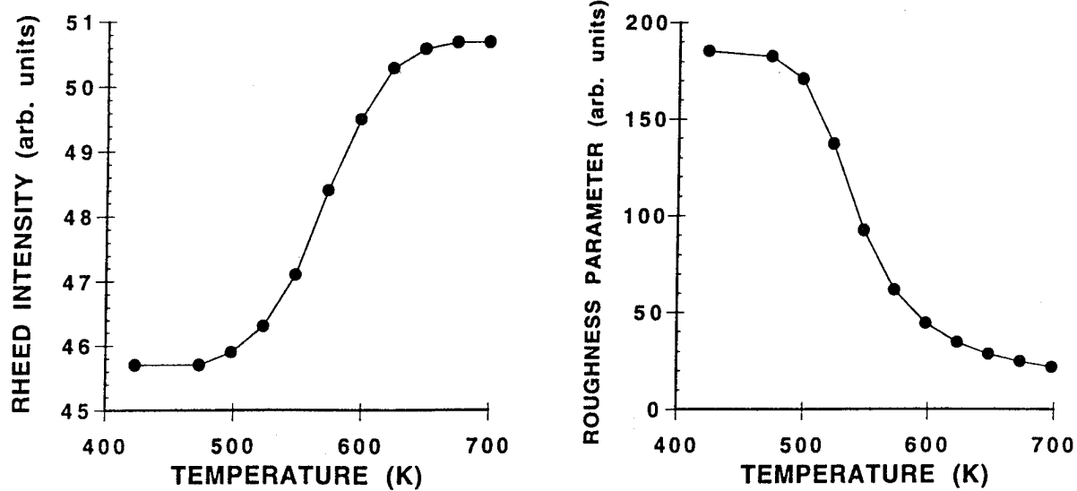
Figure 4. Comparison of the average RHEED intensity to the surface roughness predicted by the stochastic model for Ge (100) growth.
