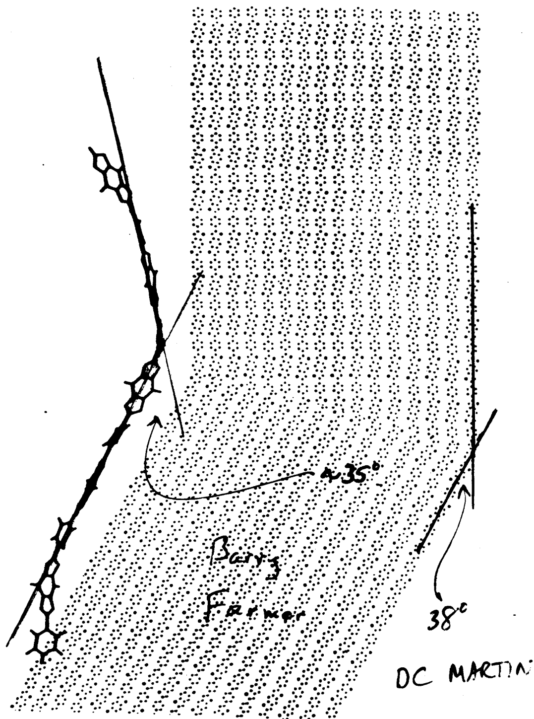
Figure 6.14: Molecular interpretation of Figure 6.13 which is consistent with the experimental HREM contrast. The molecules undergo a sharp bend as they change from one orientation to the other across the boundary. This would require the bending of covalent bonds in each polymer which passes through the ACR boundary.
