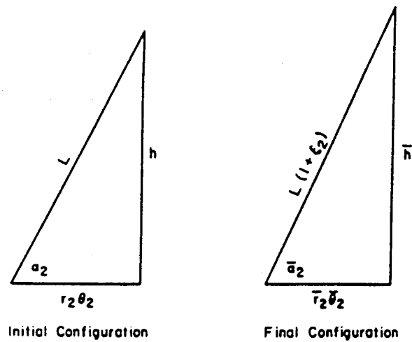
FIGURE 3.4. Developed view of outer wire centerline.
