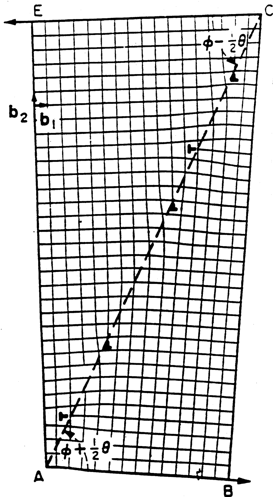
Figure 11: A graphical representation of a low angle tilt boundary of the type in figure 10 showing the inclusion of several dislocations located D from each other to incorporate the tilt. For figure 10, D is calculated to be 11.5 nm. [27]
