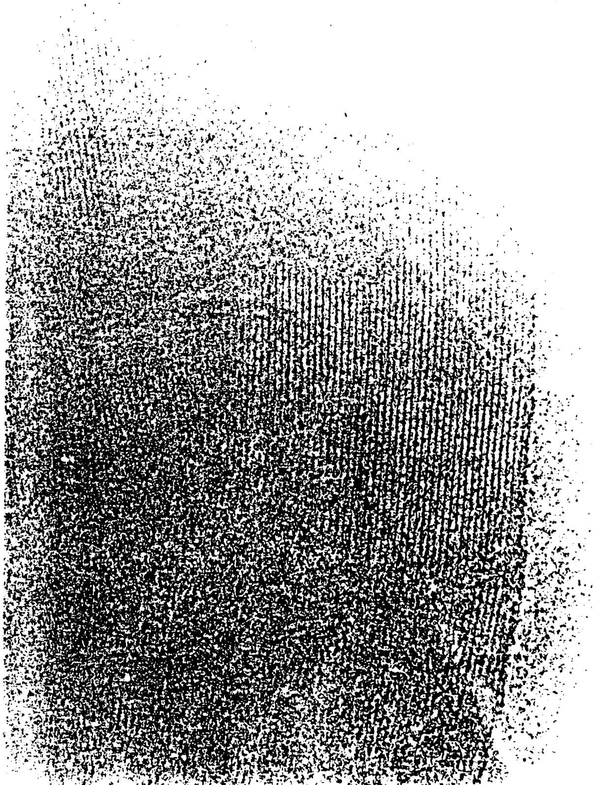
Figure 8: HREM image of poly(DCHD) droplet edge with fringes from (010) planes bent. On close inspection the bending is actually a series of tilt boundaries possible formed by the polygonalization of defects.
