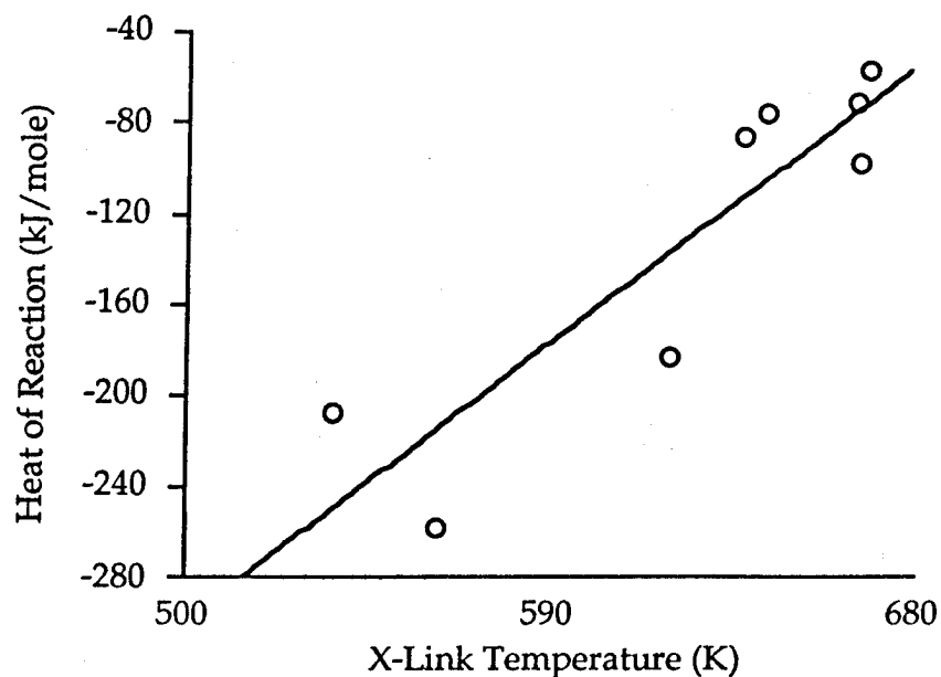
Figure 1: Plot of heat of reaction vs. maximum cross linking temperature for the BCB model compounds listed in Table 1.
