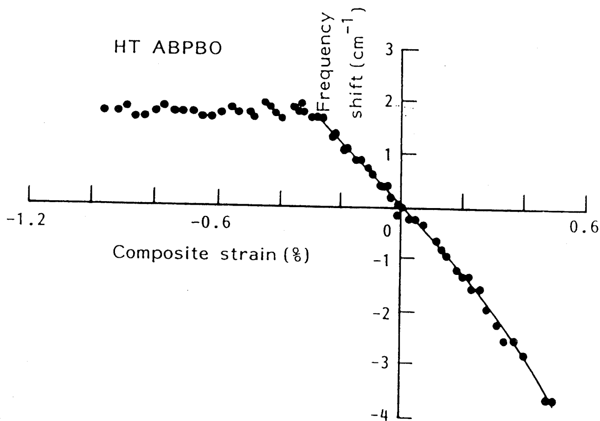
Figure 10 Dependence of peak position for the 1555 cm -1 Raman band upon both tensile (positive) and compressive (negative) strain for embedded fibres of (a) AS ABPBO and (b) HT ABPBO. The full curves are fits of the experimental data during elastic deformation to third-order polynomials
