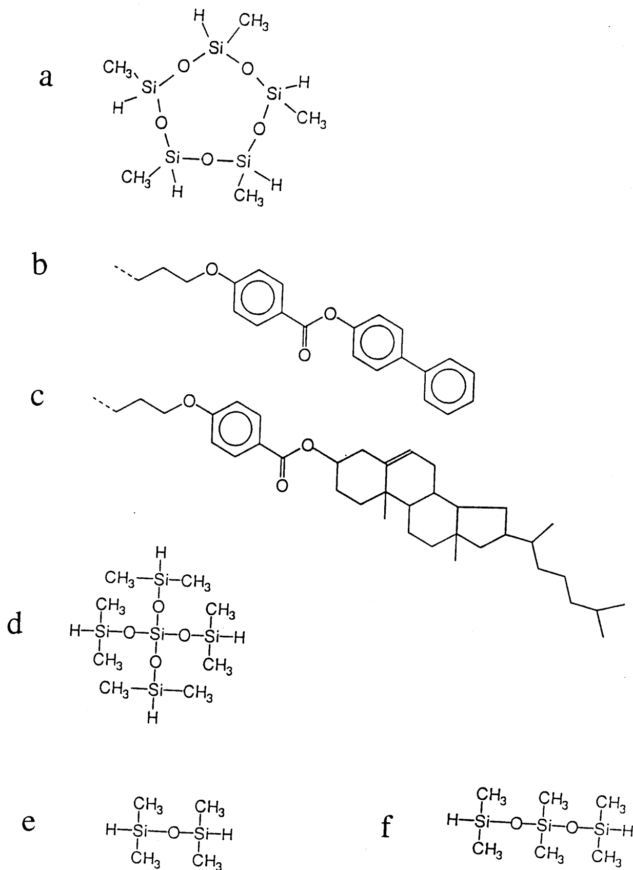
136 Figure 1. Siloxane and mesogen structures (schematic). (a) Five-membered siloxane ring. (b) Biphenyl mesogen with leader group. (c) Cholesteryl mesogen with leader group. (d) Star siloxane. (e) Linear dimer. (f) Linear trimer.
