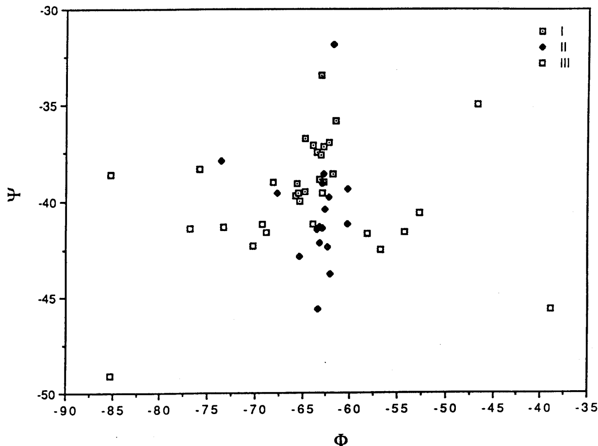
Figure 4. Backbone dihedral angles in the unsubstituted model I, and substituted models II and III. The dihedral angle values are those of the mode, which is the angle for which the largest number of conformations were found during the dynamics simulation, as explained in the text.
