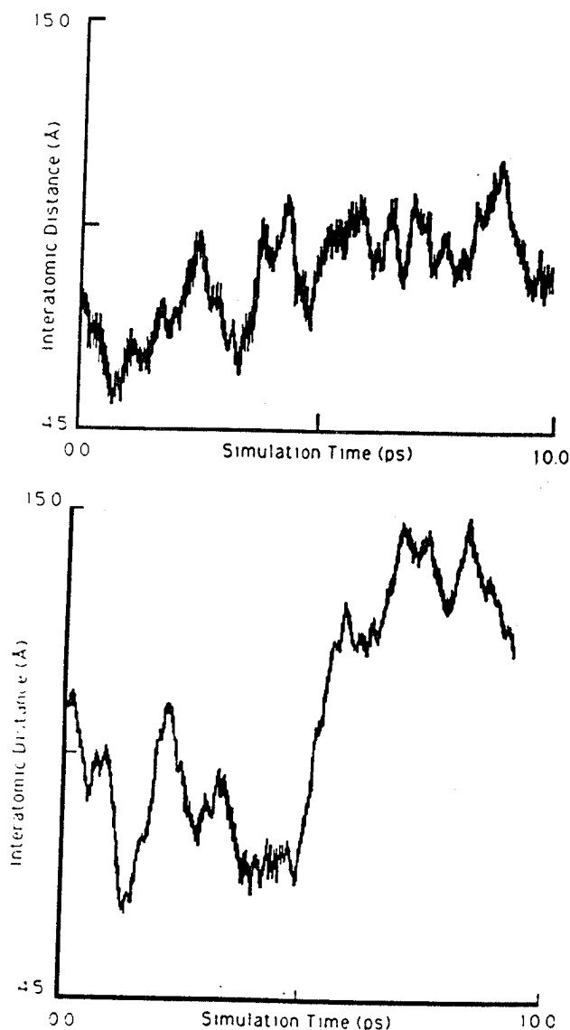
Figure 8. Distance (Å) fluctuations during the simulation between the side chains of residues {7} and {11}, for the (a) II- and (b) III-substituted analogues.
