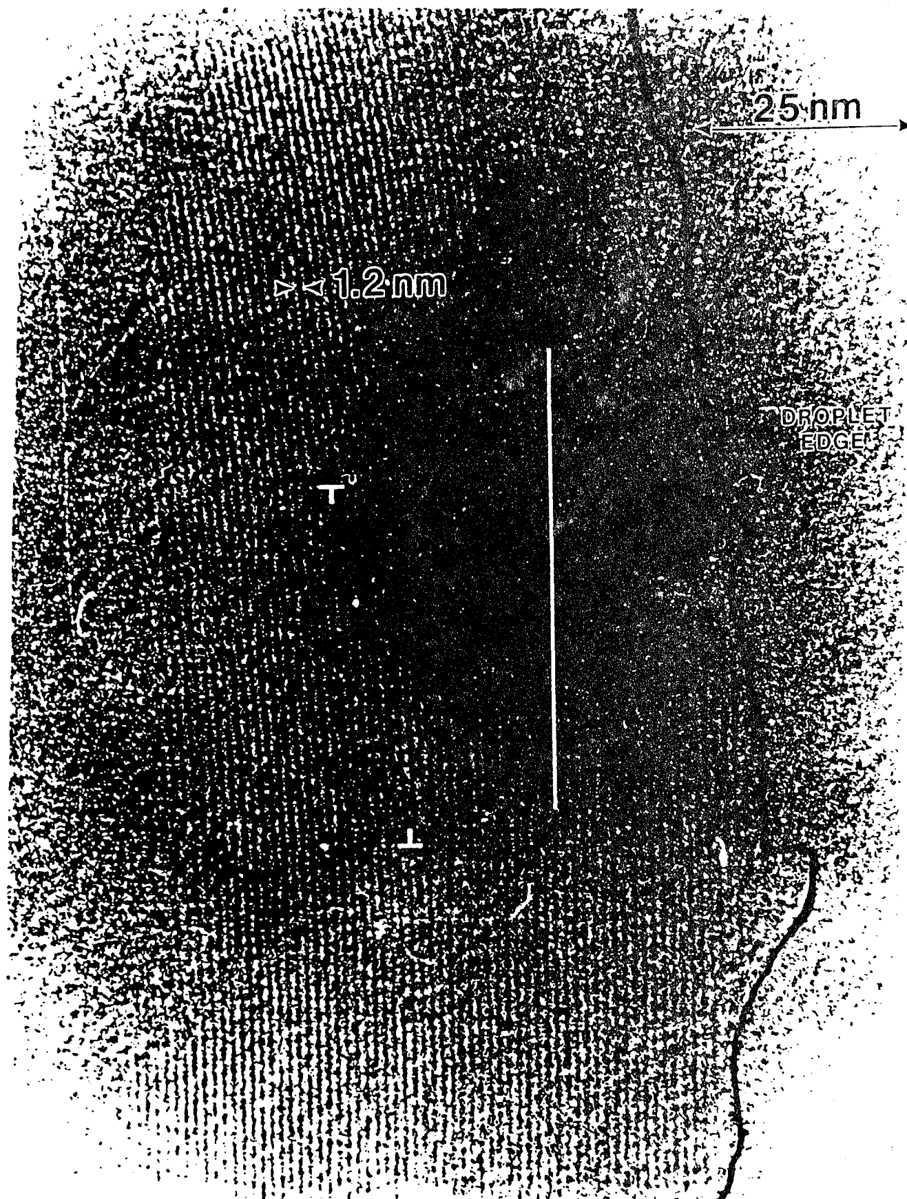
Figure 7: HREM image of DCHD droplet edge where the chain axis is parallel to the edge. The lattice fringes from the (010) plane can be seen to bend to conform to the droplet surface. Several edge dislocations with a Burgers vector in the [010] direction can be seen.
