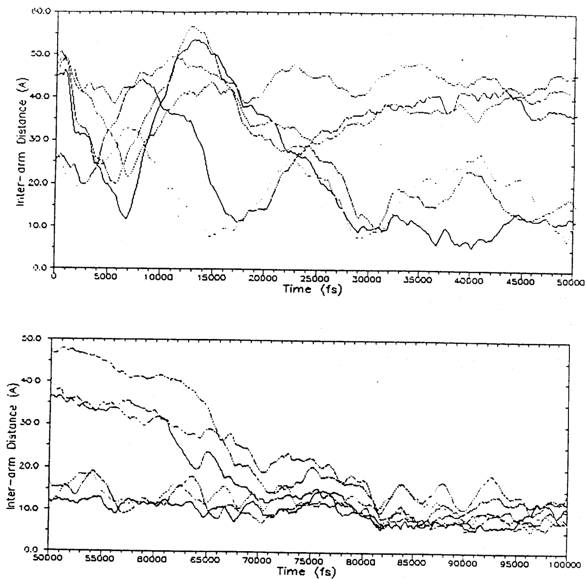
Figure 6. The distances between mesogens for the (4C) star as a function of time during the simulation: (top) from 0 to 50 ps and (bottom) from 50 to 100 ps.
