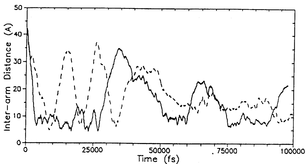
Figure 13. The distances between mesogens for the linear dimer (solid lines) and trimer (broken lines) containing two biphenyl mesogens (top) and one cholesteryl and one biphenyl mesogen (bottom).
