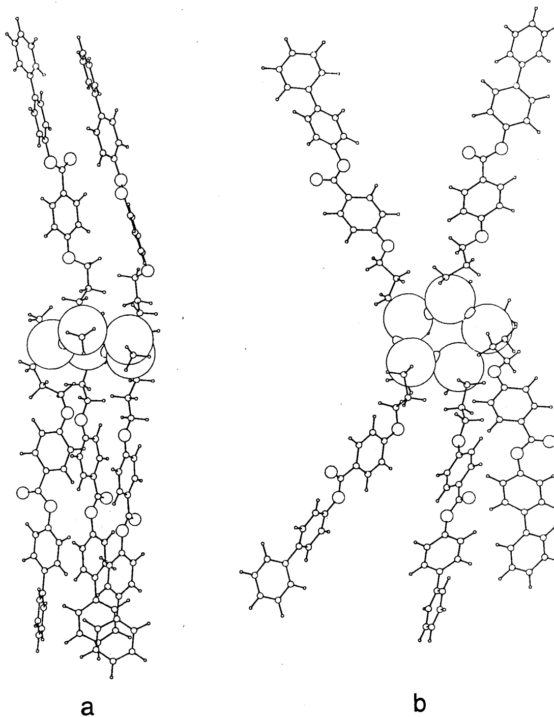
Figure 1: Ball and Stick Figure of Cylindrical Models. (a) - Model A, (b) - Model B.
