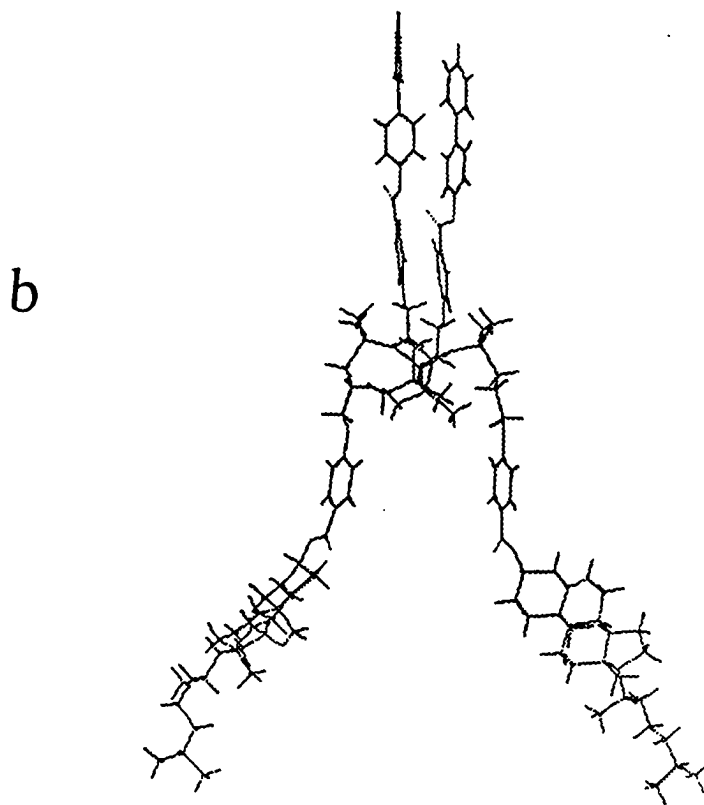
Figure 2. Starting geometries of the star siloxane (a) substituted with four biphenyl mesogens: (4B); and (b) substituted with two biphenyl and two cholesteryl mesogens: (2B2C);
