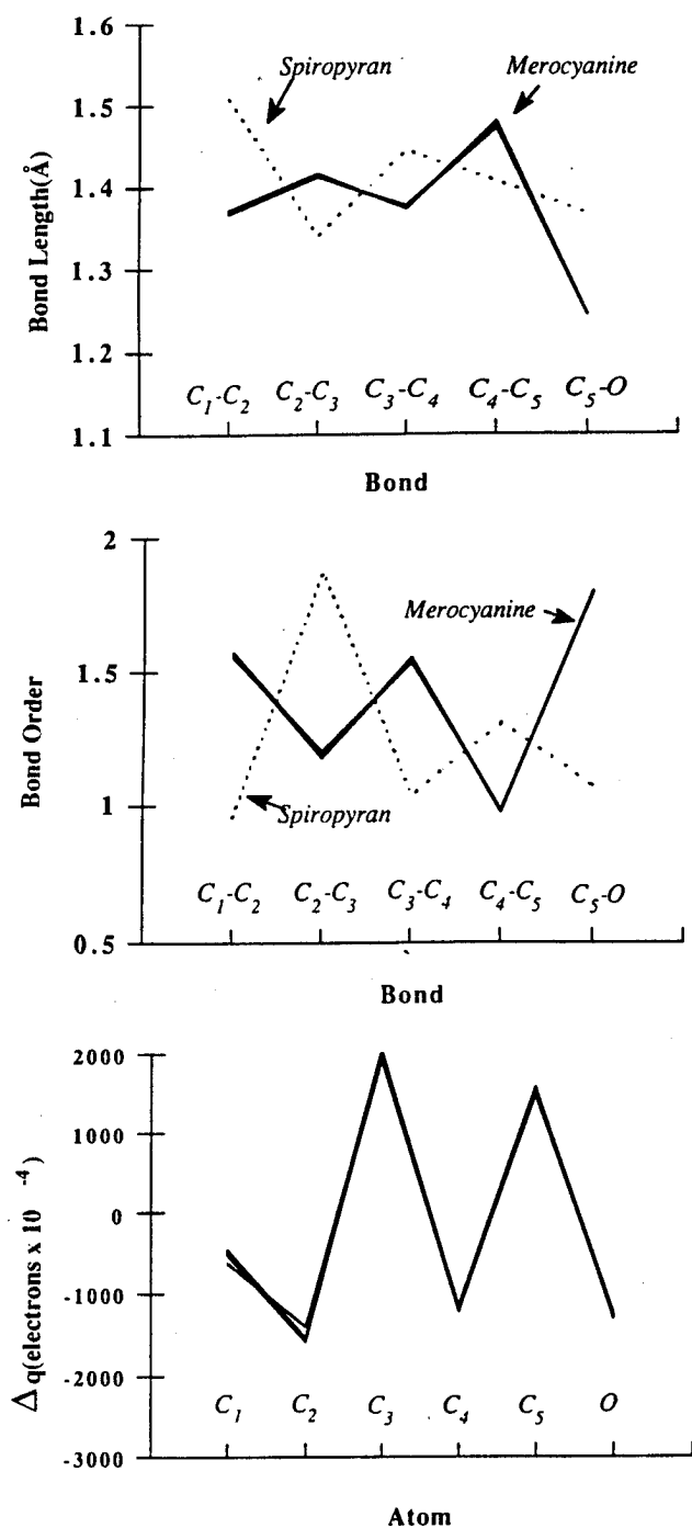
Figure 3. Calculated (a) bond lengths (Å), (b) bond orders, and (c) relative [\Delta q = q(\text{III}) - q(\text{II})] partial atomic charges (in electrons \cdot 10^{-4} ) for the merocyanine intermediate species considered in the ground state.
