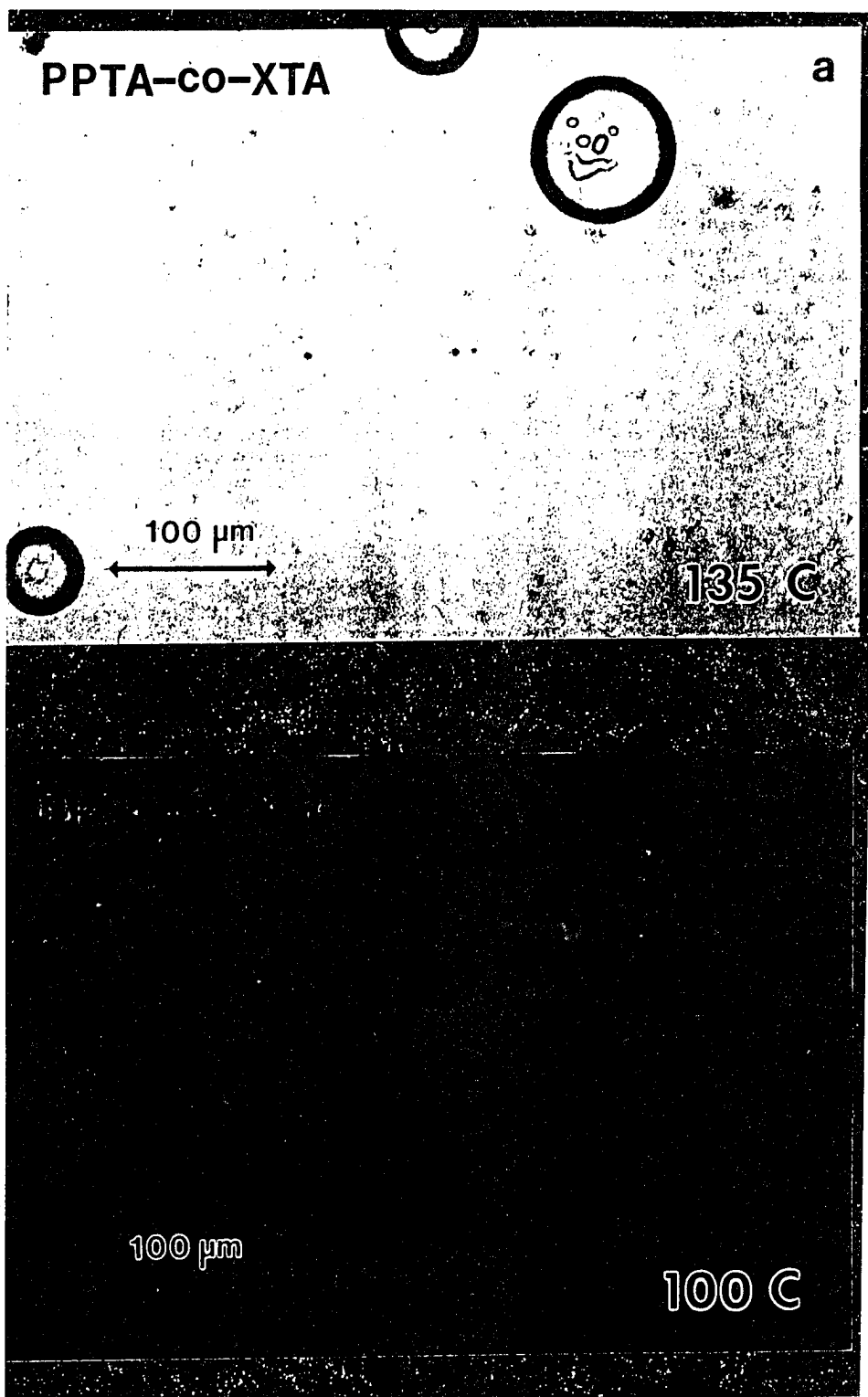
Hot Stage Optical Microscopy of PPTA-co-XTA copolymer (25% XTA) in H 2 SO 4 solution (20 weight %). Above 135 C the sample is optically isotropic. Upon cooling the solution becomes birefringent. This texture is consistent with the nematic lyotropic liquid crystalline phase found in neat PPTA solutions. Micrograph taken on an Olympus BH-2 Optical Microscope under crossed polarizers with full wave red filter.
