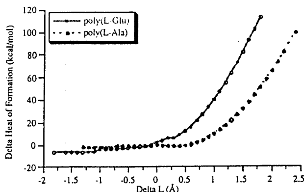
Figure 4: \Delta H_f vs. \Delta L dependence for the extended biopolymer chains: poly(L-Ala)-modulus of 160 GPa; A_{eq} \sim 20 \text{ Å}^2 , L_{eq} = 21.7 \text{ Å} , and K = 145 \text{ N/m} and poly(L-Glu)-modulus of 230 GPa; A_{eq} \sim 20 \text{ Å}^2 , L_{eq} = 14.3 \text{ Å} , and K = 320 \text{ N/m} .
