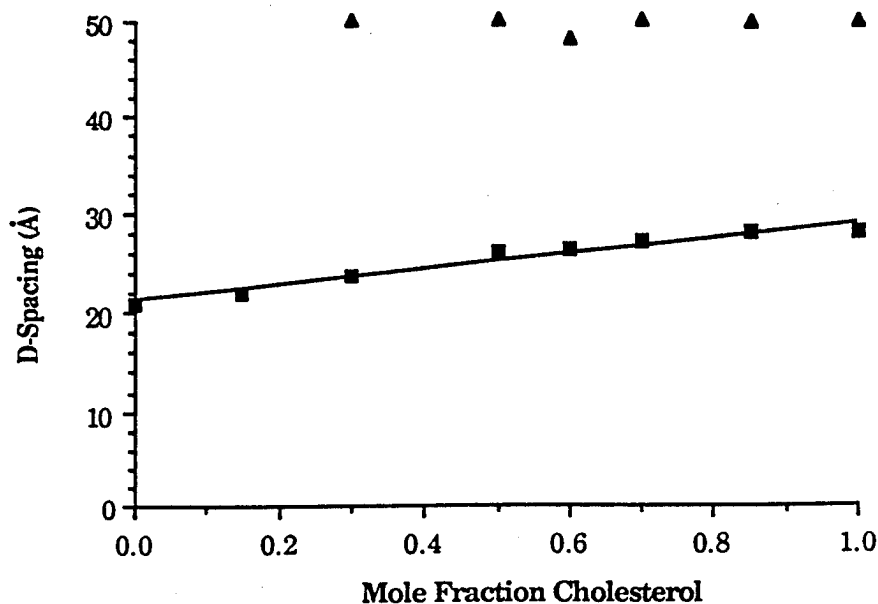
Figure 1.9: Measured primary (-o-) and low angle (-Δ-) d-spacings as a function of mole fraction cholesterol mesogen
