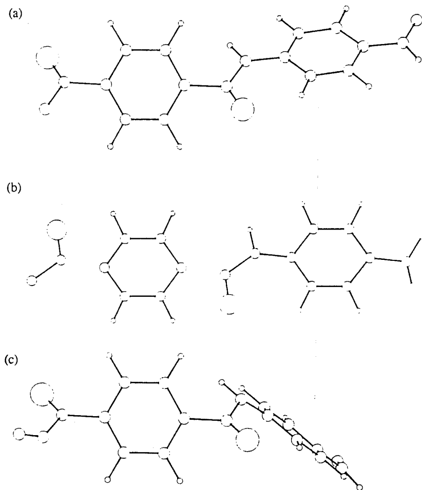
Figure 2: Equilibrium structure of PPTA(a), in tension (b), and in compression (c)
