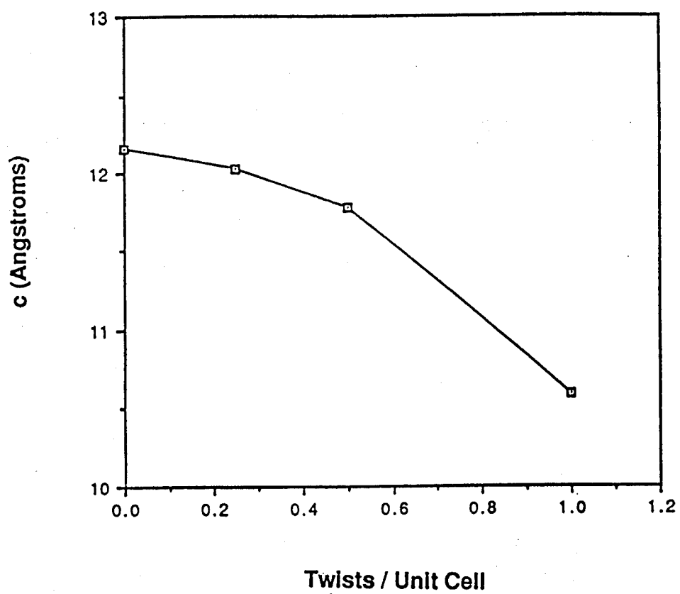
Axial Repeat Distance (c) vs. Twist Density
