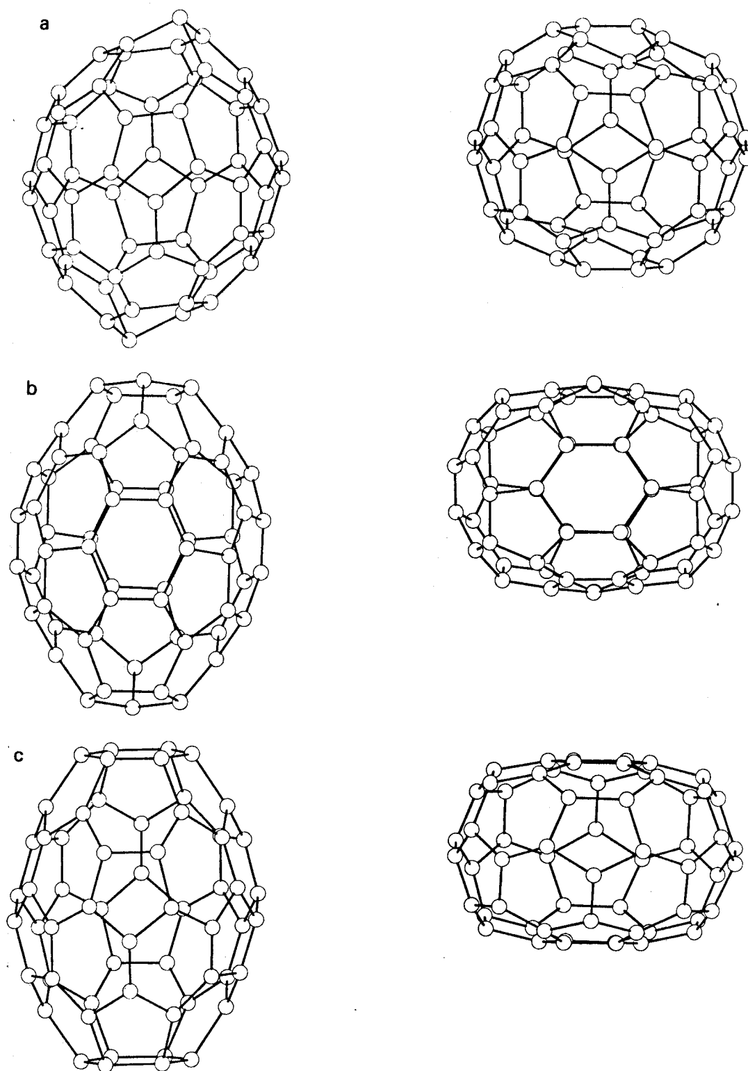
Fig. 1. Response of C 60 to anisotropic stresses applied to two opposing atoms which are colinear with the center (a), parallel to an S_{10} symmetry axis (b), and parallel to an S_6 axis (c). The virtual displacements in tension and compression are shown side by side with a vertical stress axis. The amplitude of the distortions has been adjusted separately for each stress axis.
