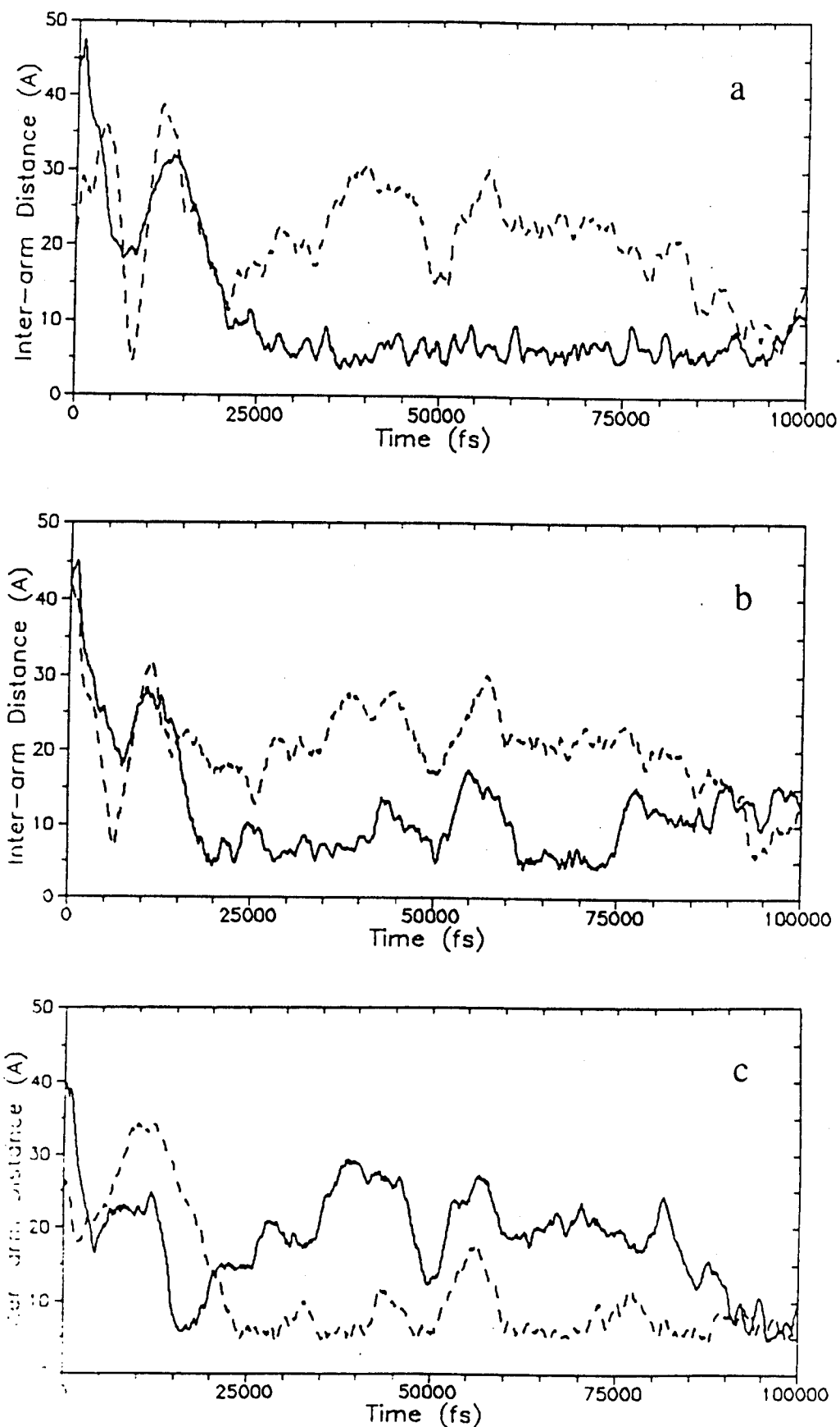
Figure 4. The distances between mesogens for the (2B2C) star as a function of time during the simulation: (a) Distances between the two cholesteryl mesogens (solid line) and the two biphenyl mesogens (broken line); (b) Distances between B1 and the two cholesteryl mesogens; (c) Distances between B2 and the two cholesteryl mesogens.
