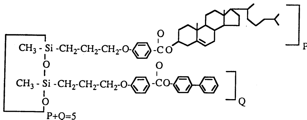
Figure 1.1: General Chemical Structure of the cyclic siloxane-based liquid crystal
