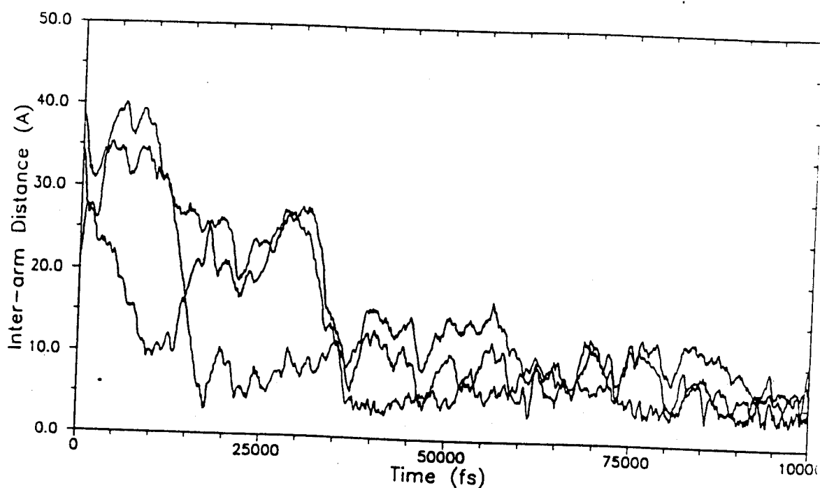
Figure 8. The three closest inter-arm distances between for the (4B) star as a function of time during the simulation, using a force field adjusted for the biphenyl torsion.
