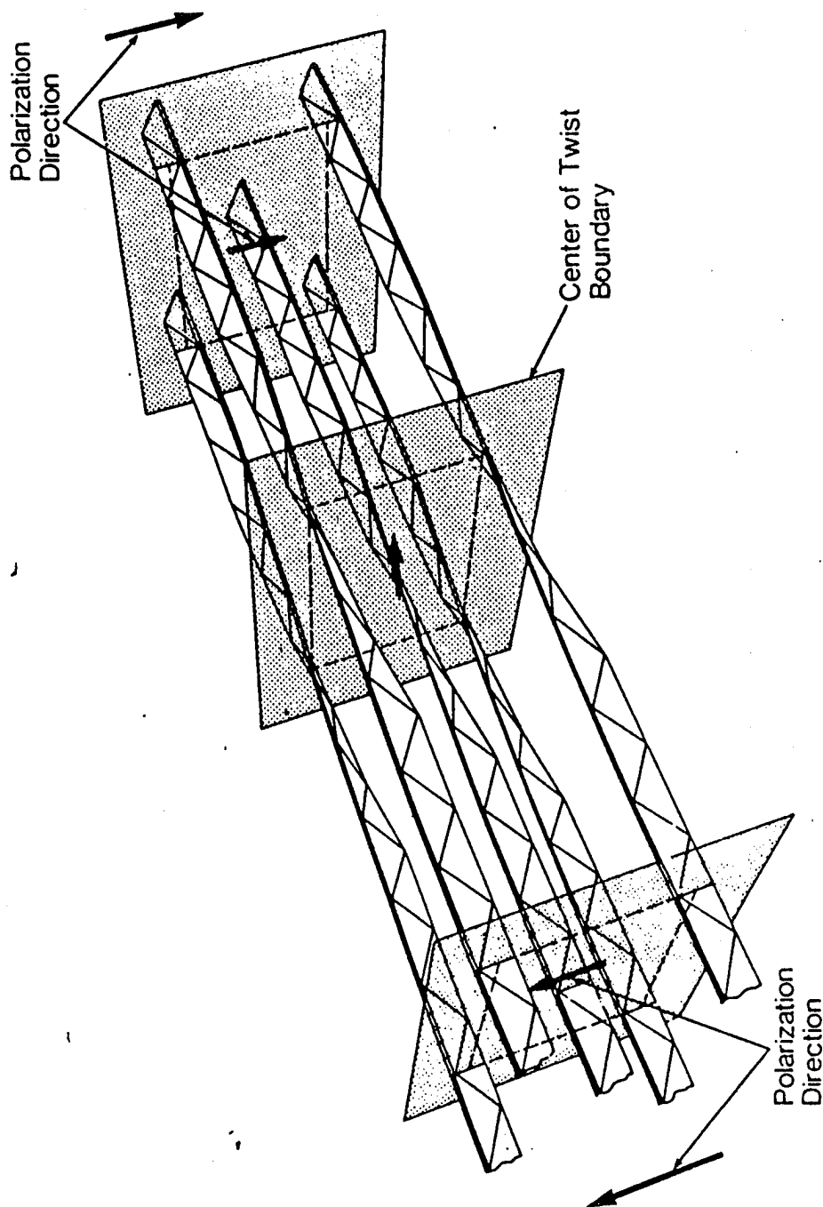
Figure 3. Twist boundaries in 5 chains are shown, with the calculated conformation. There are 21 carbon atoms between the hatched rectangles near the ends. The middle rectangle shows the location of the centre of the twist boundary. The polarization directions are shown by arrows. The direction of the dipole is reversed as the molecule passes through a twist boundary. When an external field is present, the total energy is lowered as the twist boundary moves in a direction that allows more of the dipoles attached to each molecule to align with the field.
