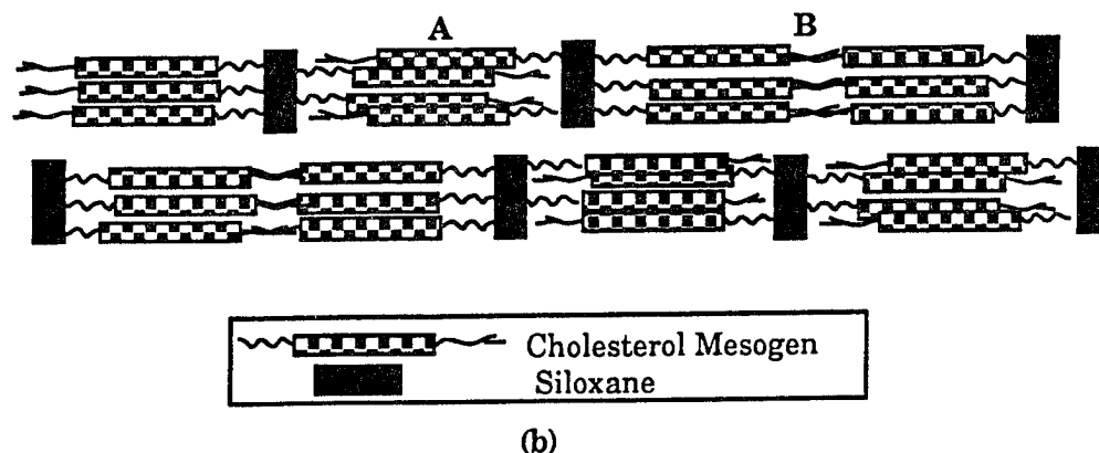
Figure 1.12: Schematic of packing in: {B} mesogen substituted siloxane molecules (a) and {C} mesogen substituted siloxane molecules (b)
