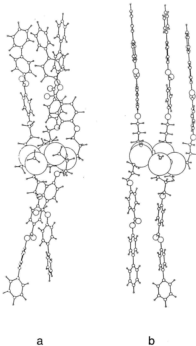
Figure 4: Molecular Structure After 50 picosecond Dynamics Simulation. (a) Without Boundary Condition; (b) With Boundary condition.
