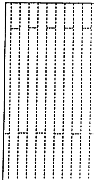
Chemical Crosslinks
