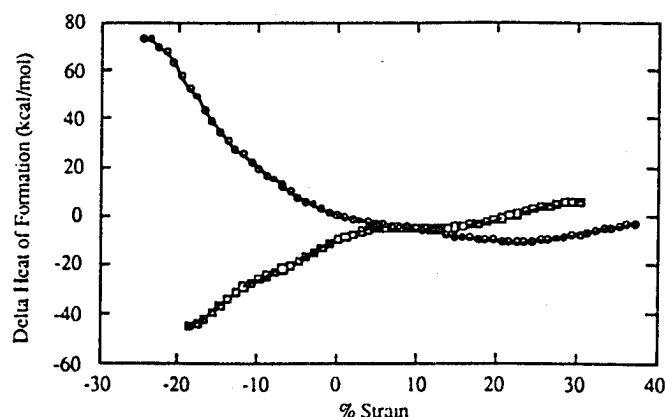
Figure 5: \Delta H_f vs. \Delta L dependence for the alpha-helical model of poly(L-Ala)-modulus of 60 GPa, where A_{eq} \sim 20 \text{ \AA}^2 , L_{eq} = 10.2 \text{ \AA} , and K = 107 \text{ N/m} . The force ( 10^{-10} \text{ N} ) curve (squares) shows that in distinct contrast to PPTA (Fig. 1), there is no evidence for 'kinking'.
