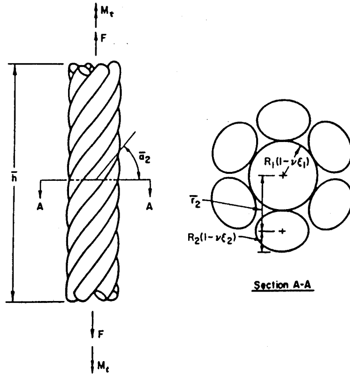
FIGURE 3.1. Loaded simple straight strand.
