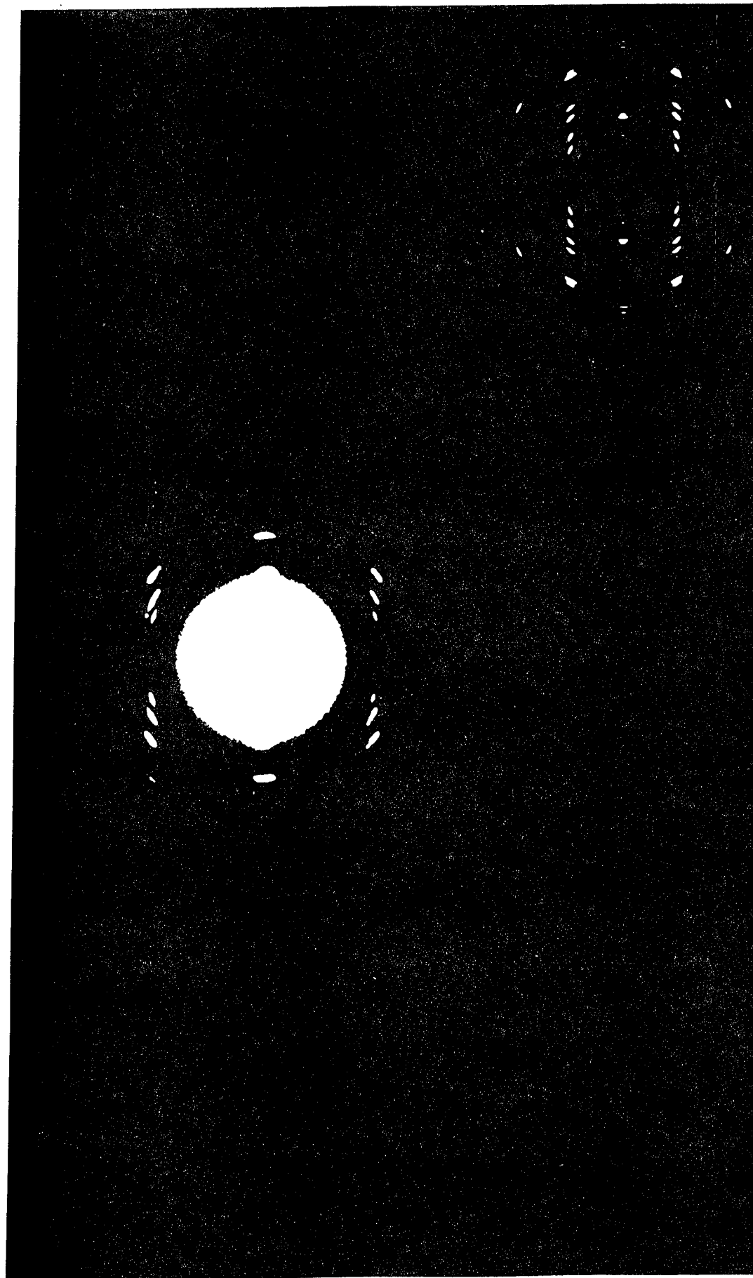
Figure 4: SAED of poly(DCHD) droplet. The mirror symmetry of the pattern suggests a fiber texture of the droplet. The inset shows a simulation of (CERIUS [17]) of the SAED pattern using a fiber texture geometry for the reported polymer crystal structure (Apgar and Yee [11]).
