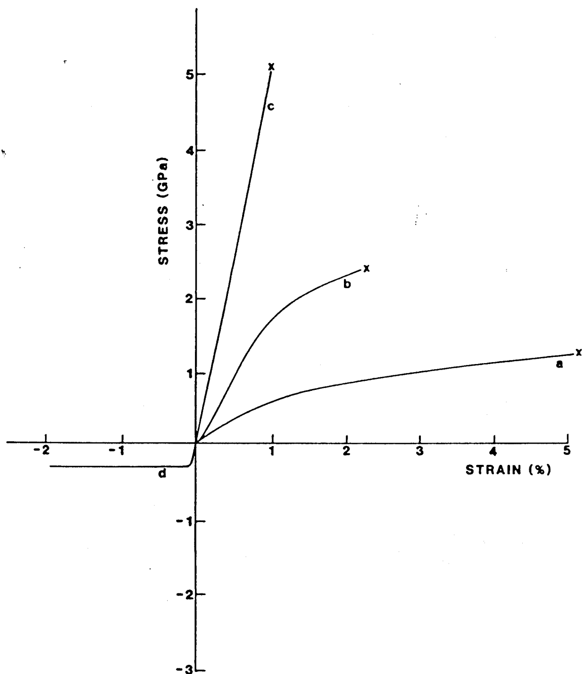
FIG. 13.31 Typical (a-c) tensile and (d) compressive stress-strain curves of PBO fibers: (a) as-coagulated (wet), (b) as-spun (dried), (c) and (d) heat-treated.
