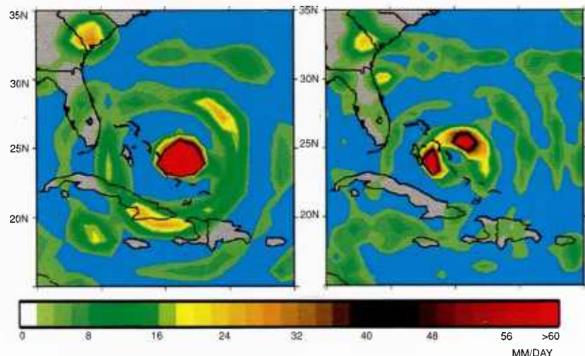
Mesoscale rainfall bands for Hurricane Andrew (24 Aug 1992) for model resolutions T106 (left) and T170 (right).
