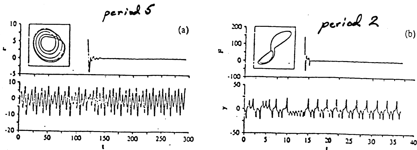
Figure 2: The output signal y(t) and the forcing term F(t) of the (a) Rosslor system : dx/dt = -y - z , dy/dt = x + 0.2y + F(t) , dz/dt = 0.2 + z(x - 5.7) , stabilized to a period-5 cycle and the Lorenz system : dx/dt = 10(x - y) , dy/dt = -xz + 28x - y + F(t) , dz/dt = xy - (8/3)z , stabilized to period-2 motion. The inset is an x-y portrait of the stabilized system. From Pyragas
