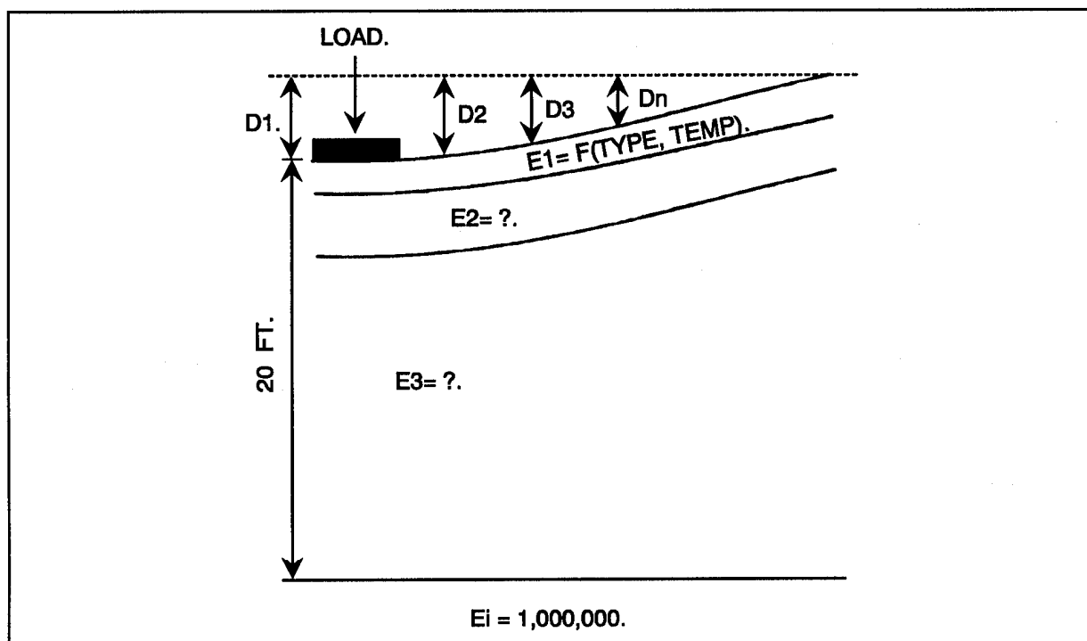
Figure E-3. Pavement structure modeled as a layered system with up to i layers ( \text{max}=5 ) and n measured deflections ( \text{max}=7 ).
