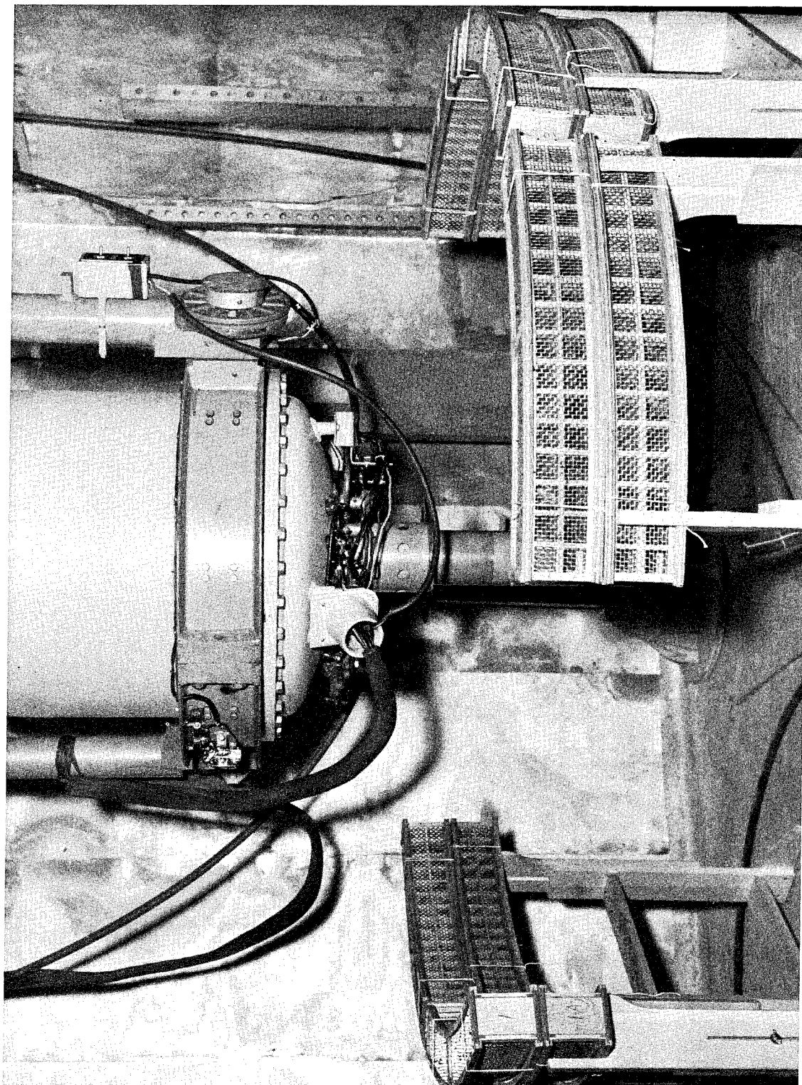
FIG. 4.18 Maxitron, 250-KVP X-ray Apparatus Installed on Japtan for Irradiation of Control Mice
