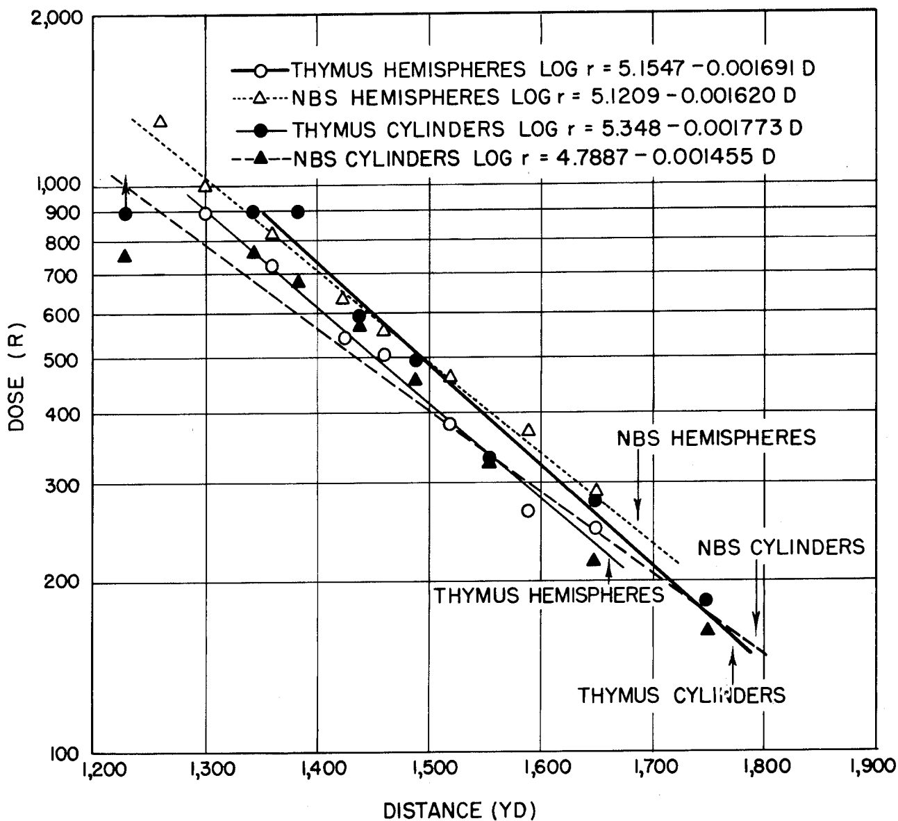
FIG. 3.4 Biological Effectiveness of Bomb Gamma Radiation in Terms of Equivalent Roentgens of 230-KVP X Rays, Measured inside the Hemispheres (open circles) and the Cylinders (closed circles) as a Function of Distance from Ground Zero, Easy Shot. Film-pack readings are represented by triangles. (Greenhouse Report, Annex 2.4, Part I, Sec. 1.)
