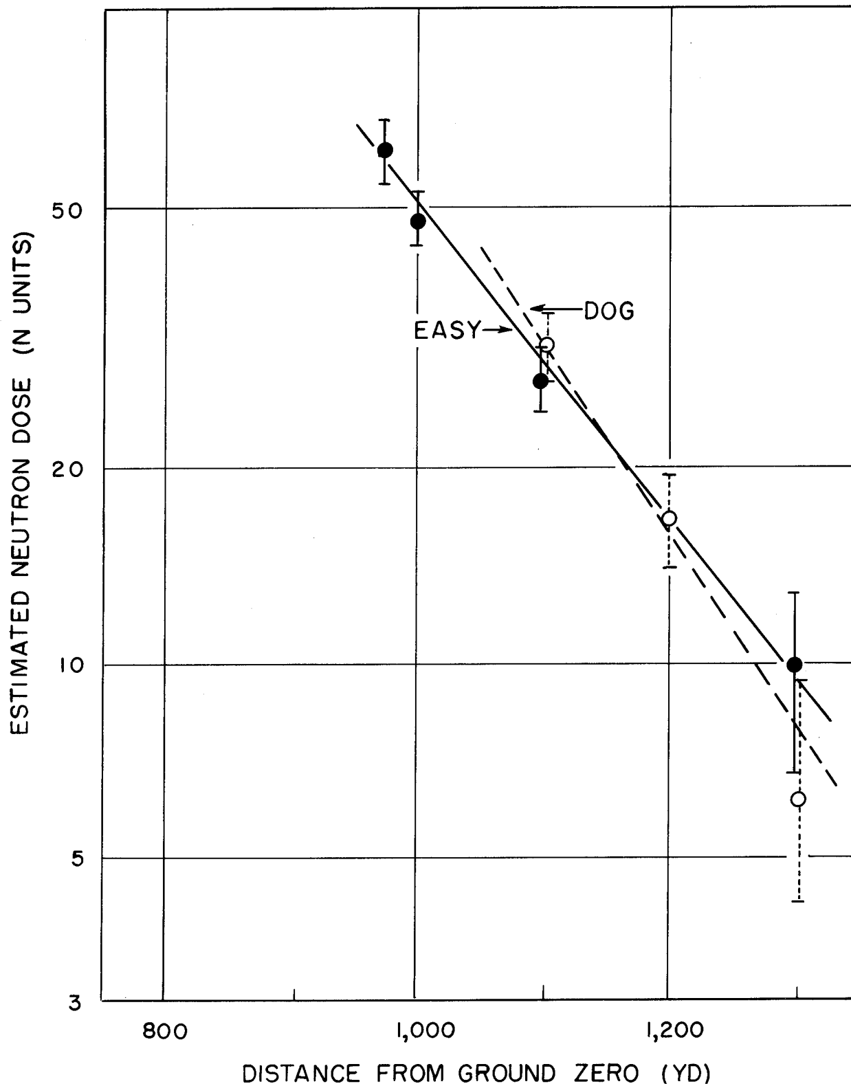
FIG. 3.10 Estimates of Neutron Dose, in n Units, as a Function of Distance, Using Tradescantia , Dog and Easy Shots. (Greenhouse Report, Annex 2.4, Part III.)
