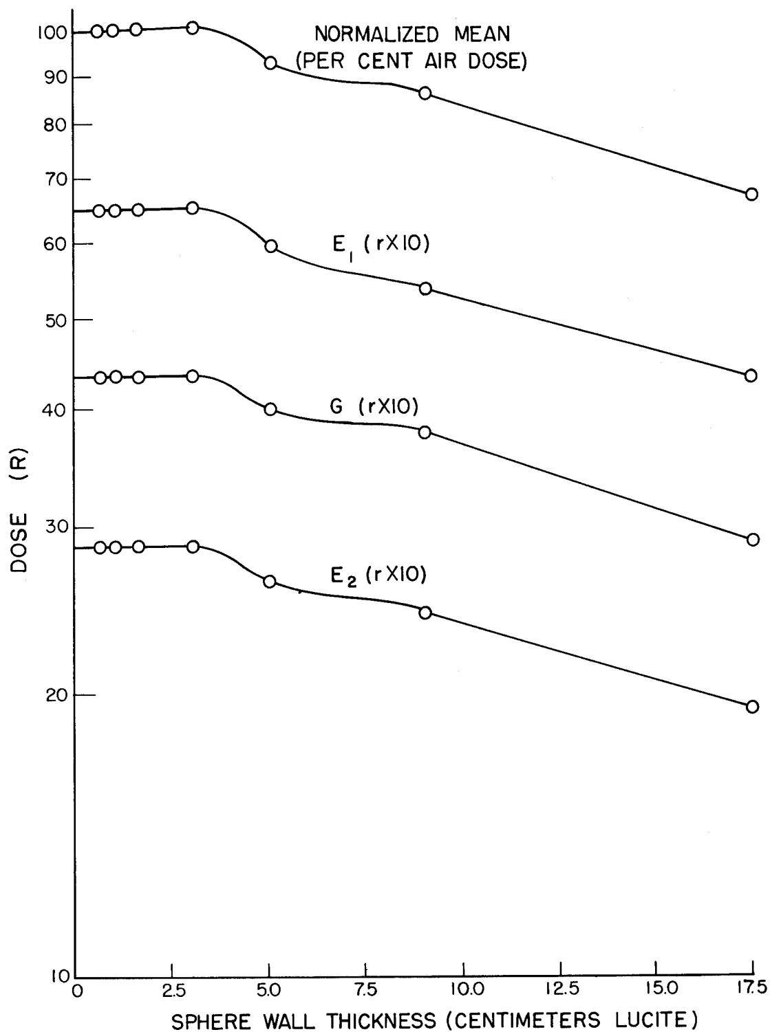
FIG. 4.2 Absorption of Bomb Gamma Radiation in Lucite Spherical Phantoms, Easy and George Shots. The dose was measured with Sievert ionization chambers. The top curve is a composite of the three lower ones, with the points normalized to per cent air dose. The readings in spheres with wall thickness 0.5 to 2.5 cm were taken as equal to the air dose. (Greenhouse Report, Annex 2.4, Part II.)
