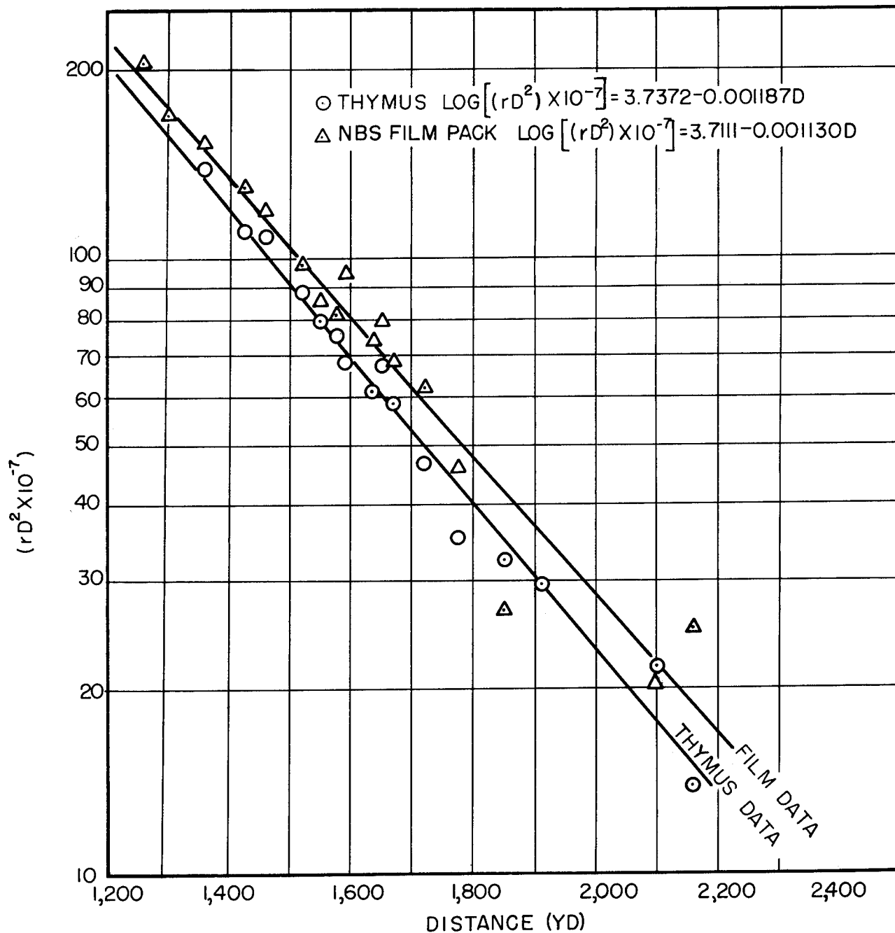
FIG. 3.6 Composite Curves of Biological Effectiveness of Bomb Gamma Radiation (expressed in roentgens equivalent of 230-KVP X rays) and NBS Film-pack Readings (calibrated with 600-KVP X rays) at Varying Distances from Ground Zero. The data from Dog, Easy, and George Shots have been combined and normalized to the yield of Easy Shot. (Greenhouse Report, Annex 2.4, Part I, Sec. 1.)
