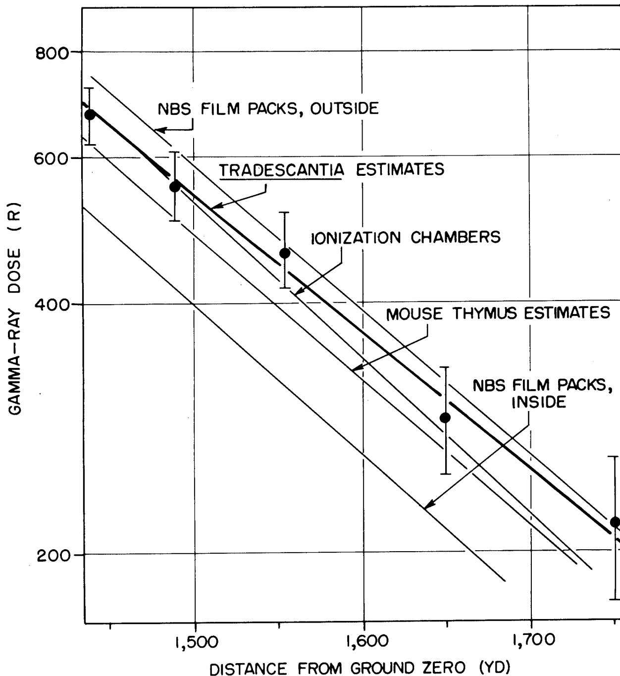
FIG. 3.9 Estimates of Bomb Gamma-ray Dose as a Function of Distance Using Tradescantia , Easy Shot. The Tradescantia , NBS film packs, and mice were inside cylinders of the 70, 71 series. The ionization chambers were in lucite spheres. (Greenhouse Report, Annex 2.4, Part III.)
