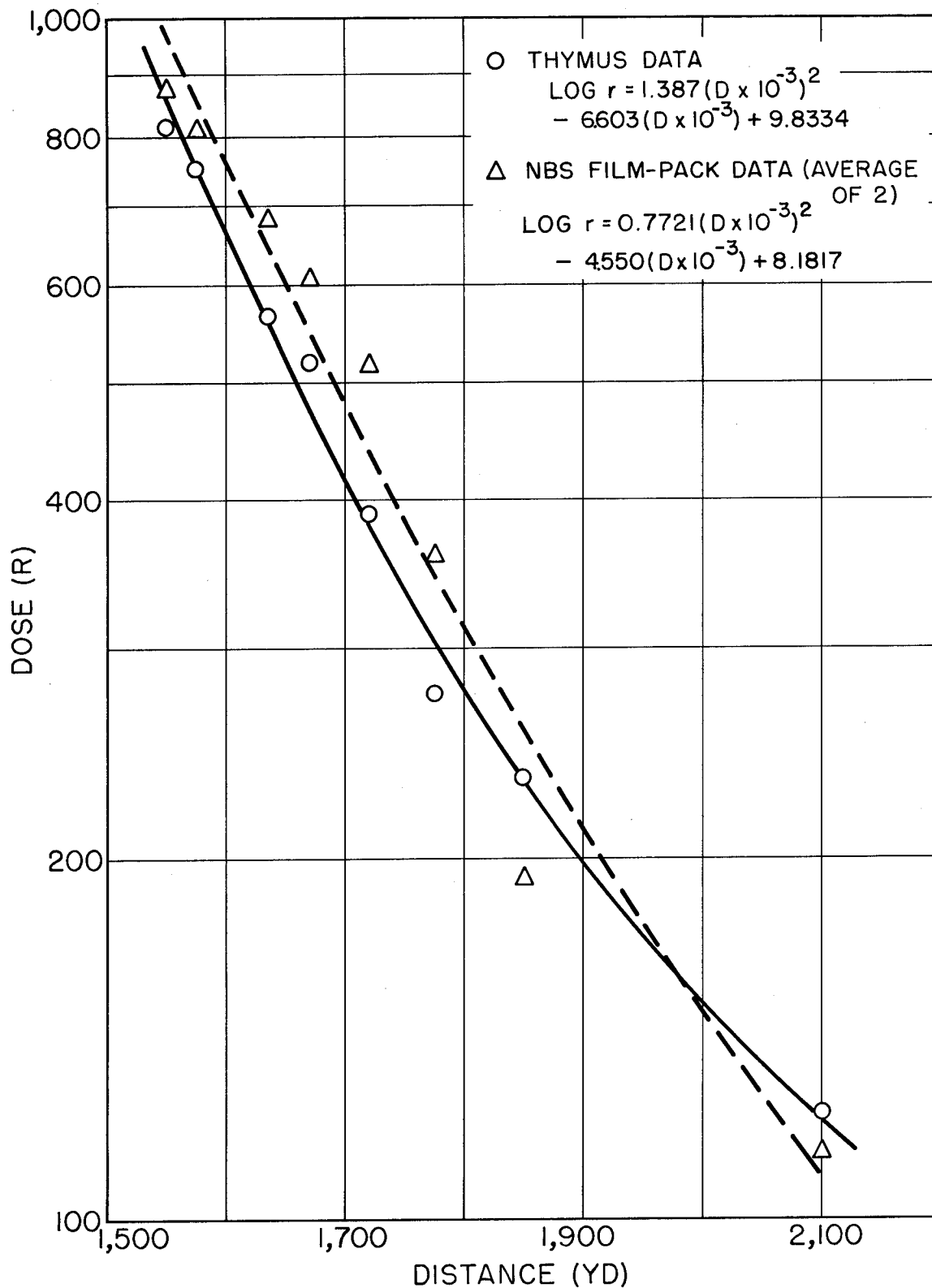
FIG. 3.2 Biological Effectiveness of Bomb Gamma Radiation in Terms of Equivalent Roentgens of 230-KVP X Rays as a Function of Distance from Ground Zero, Dog Shot. The NBS film was calibrated with 600-KVP X rays. (Greenhouse Report, Annex 2.4, Part I, Sec. 1.)
