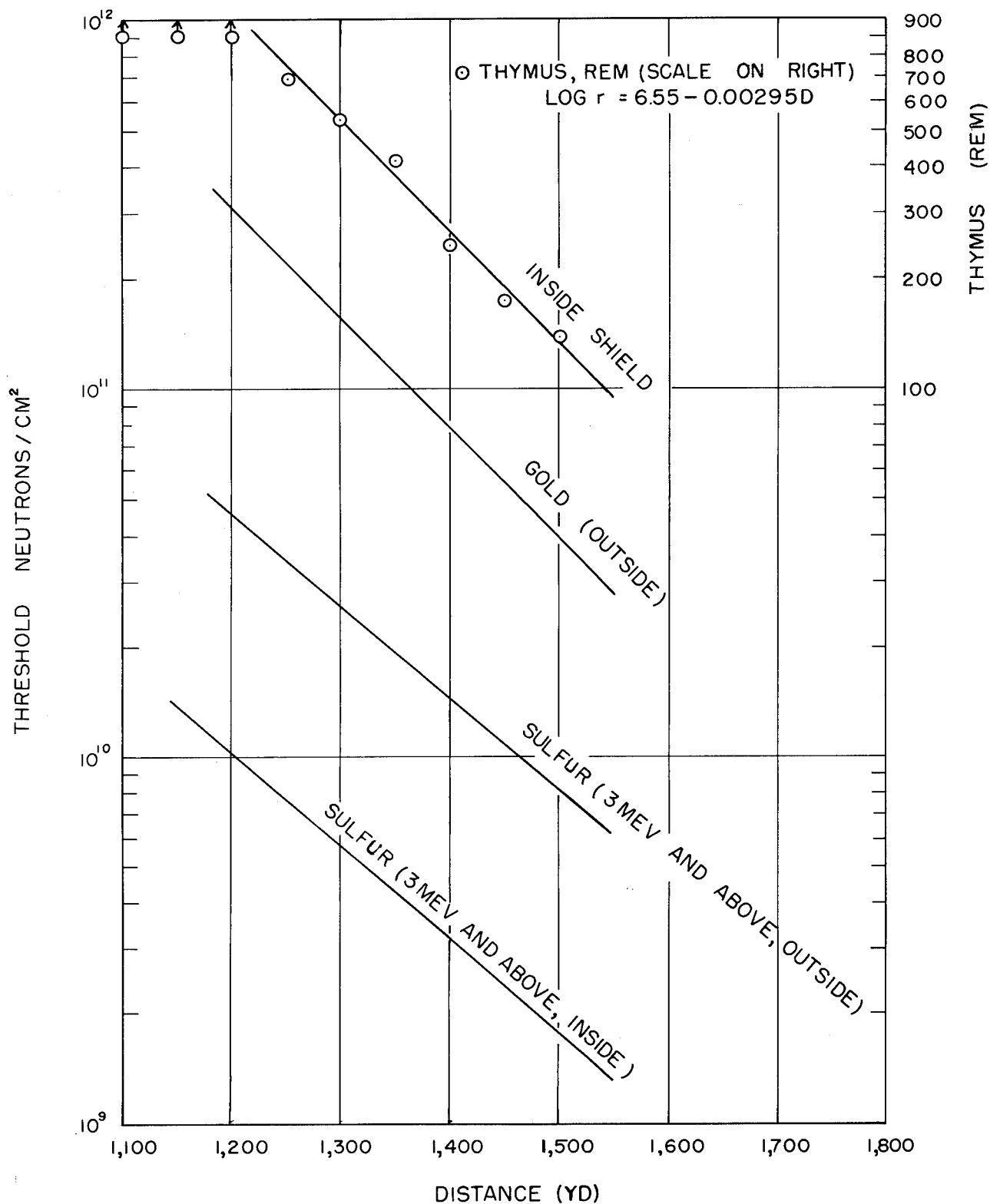
FIG. 3.5 Biological Effectiveness of Bomb Neutrons inside the 7-in.-thick Lead Hemispheres, Expressed in Roentgens Equivalent of 230-KVP X Rays, as a Function of Distance from Ground Zero, George Shot. The scale for thymus roentgens equivalent man is located arbitrarily and implies no relation to the neutron scale. (Greenhouse Report, Annex 2.4, Part I, Sec. 2.)
