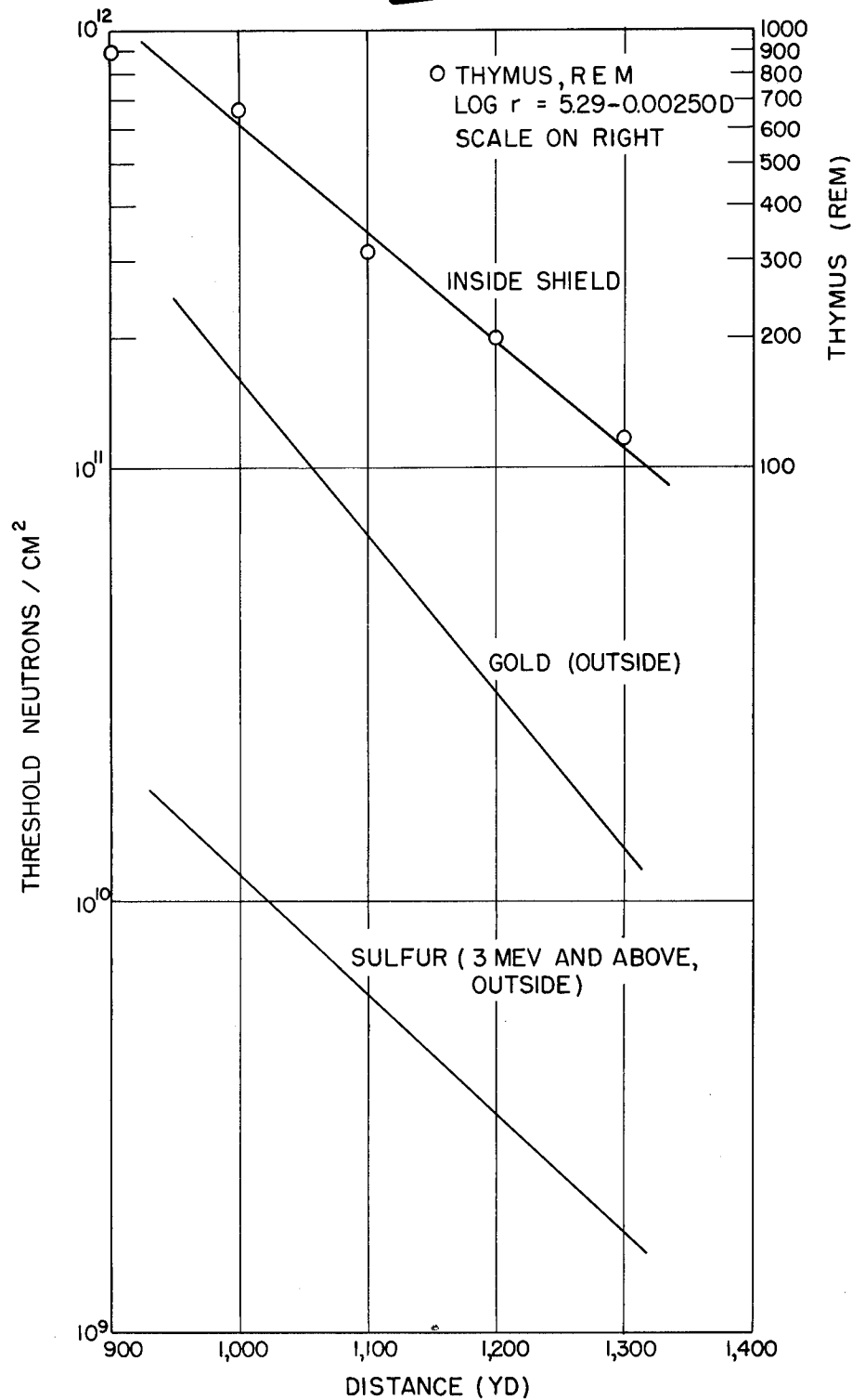
FIG. 3.3 Biological Effectiveness of Bomb Neutrons inside the 7-in.-thick Lead Hemispheres, Expressed in Roentgens Equivalent of 230-KVP X Rays, as a Function of Distance from Ground Zero, Dog Shot. The values for threshold neutrons were obtained outside the shield. The scale for thymus roentgens equivalent man is located arbitrarily and implies no relation to the neutron scale. (Greenhouse Report, Annex 2.4, Part I, Sec. 2.)
