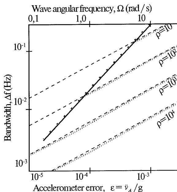
Fig. 7. Requirements to system bandwidth depending on wave frequency and accelerometer error.
