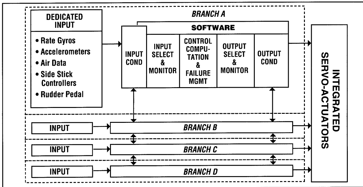
Figure 4 F-16 Digital Flight Control System
