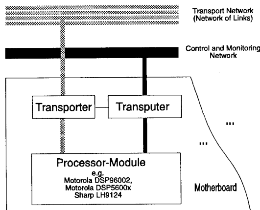
Figure 10: Communication structure for the processor
