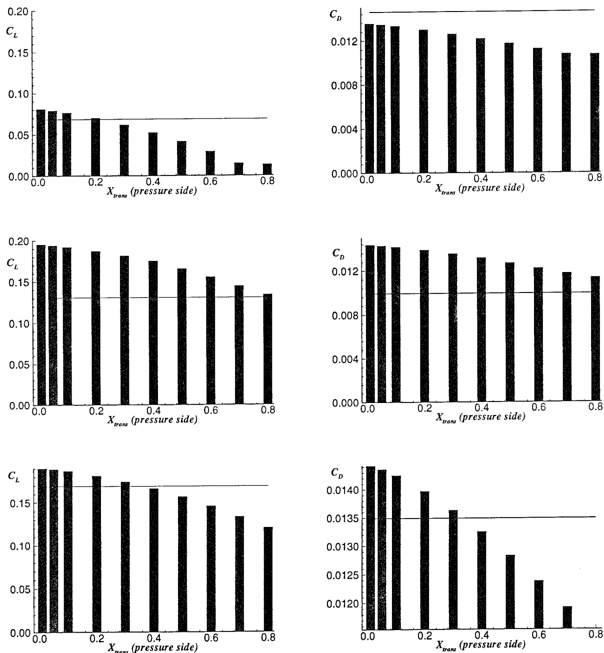
Figure D-8: Lift and drag coefficients as a function of transition location, on the pressure side of the foil. Cavity flow, \alpha = 1.66^\circ , l/c = 0.20 .
