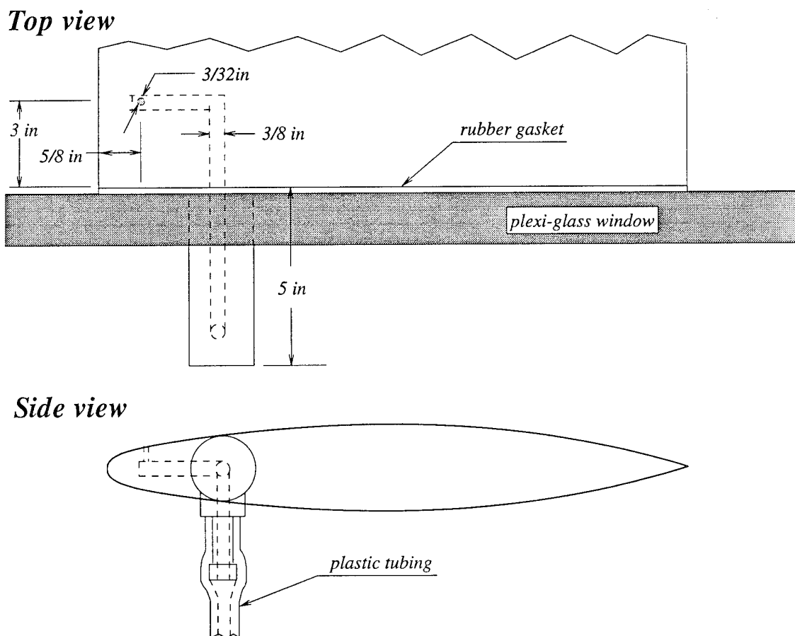
Figure 2-6: Top and side view of hydrofoil, in tunnel testing section, showing the location of the pressure tap.
