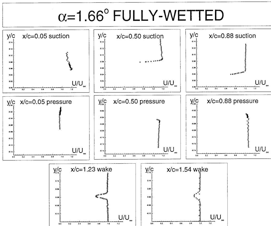
Figure C-1: Experimental velocity measurements in the boundary layer region. \alpha = 1.66^\circ , fully - wetted .
