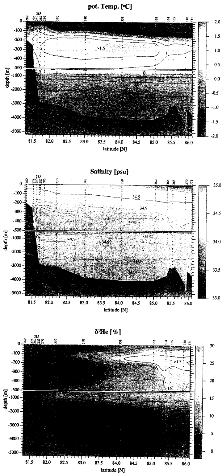
Fig. 3.25 Sections of potential temperature (°C), salinity and \delta^3\text{He} (%) in the Nansen Basin, nominally at 30E. Polarstern 1987 transect (by courtesy of Gerhard Bönisch).
