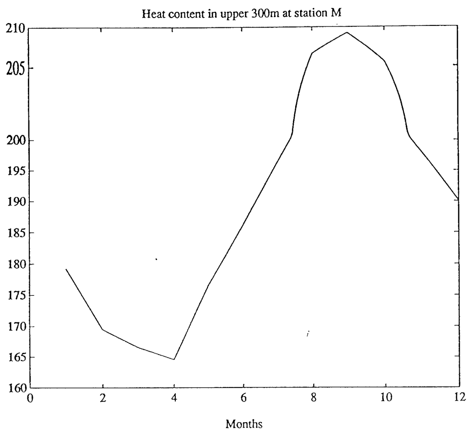
Fig. 5.3 Seasonal variations in heat content at Weather Station Mike.
