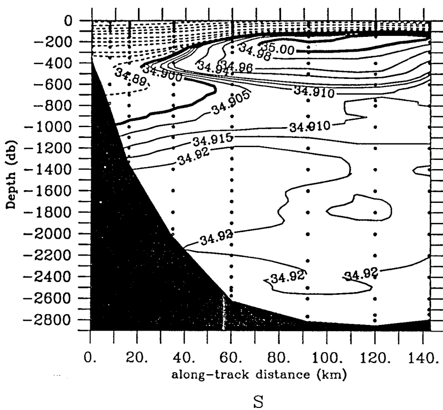
Fig. 3.22 Potential temperature and salinity in the western Fram Strait. Polarstern 1984 transect. Cruise track is shown in fig. 3.2b (P84-79).
