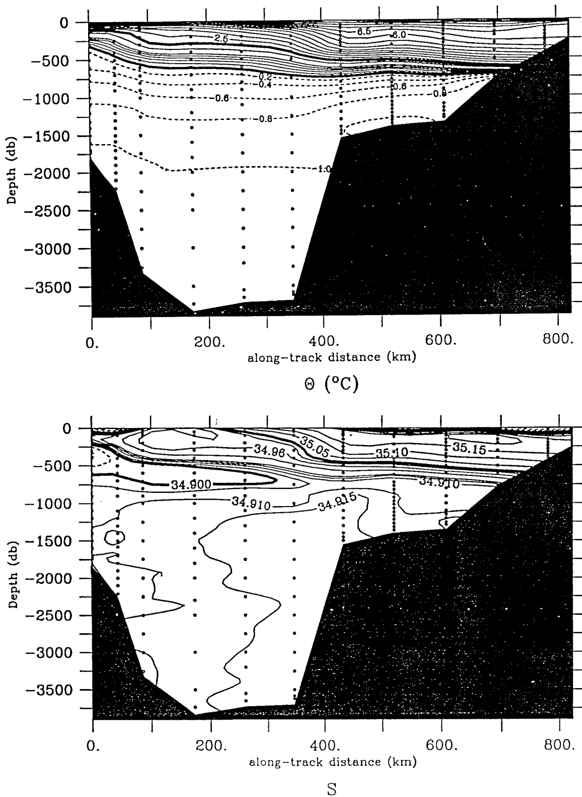
Fig. 3.5 Temperature and salinity section at 67 N. Meteor 1985 transect. Cruise track is shown in fig. 3.2b (M85-67).
