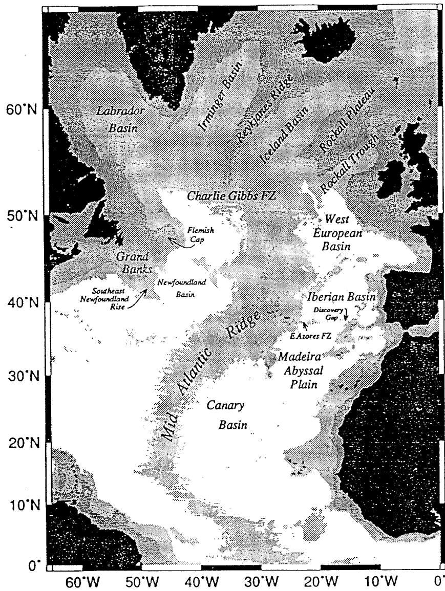
Fig. 2.5 Bathymetry and location of geographic features south of the Greenland-Scotland Ridge
