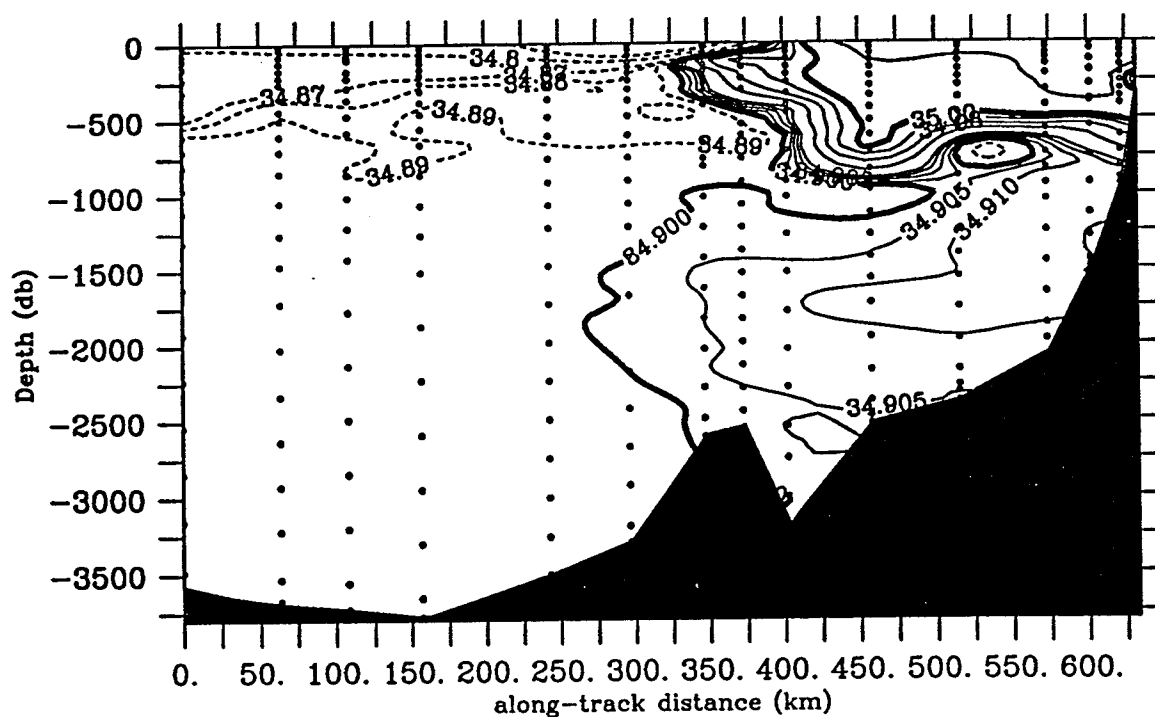
Fig. 3.33 Temperature and salinity crossing eastern Greenland Sea and northern Lofoten Basin at 75N. Hudson 1982 transect. Cruise track is shown in fig. 3.2b (H82-75).
