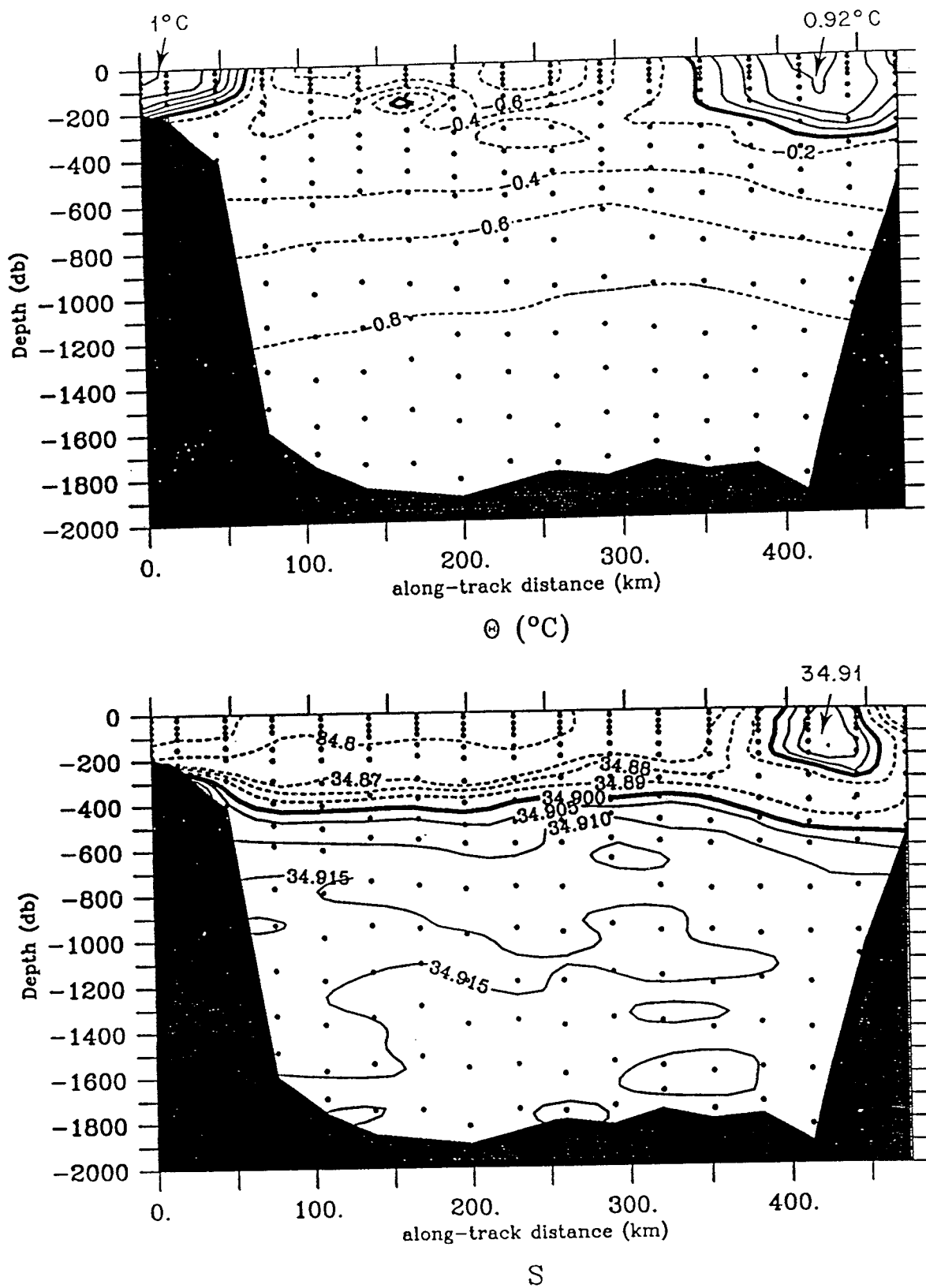
Fig. 3.16 Temperature and salinity crossing the Central Iceland Sea. Bjarni Sæmundsson 1982 transect. Cruise track is shown in fig. 3.2b (BS82).
