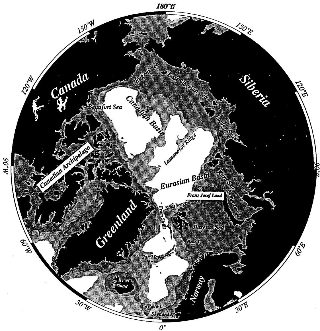
Fig. 2.4a Bathymetry and location of geographic features in the Nordic Seas and Arctic Ocean
