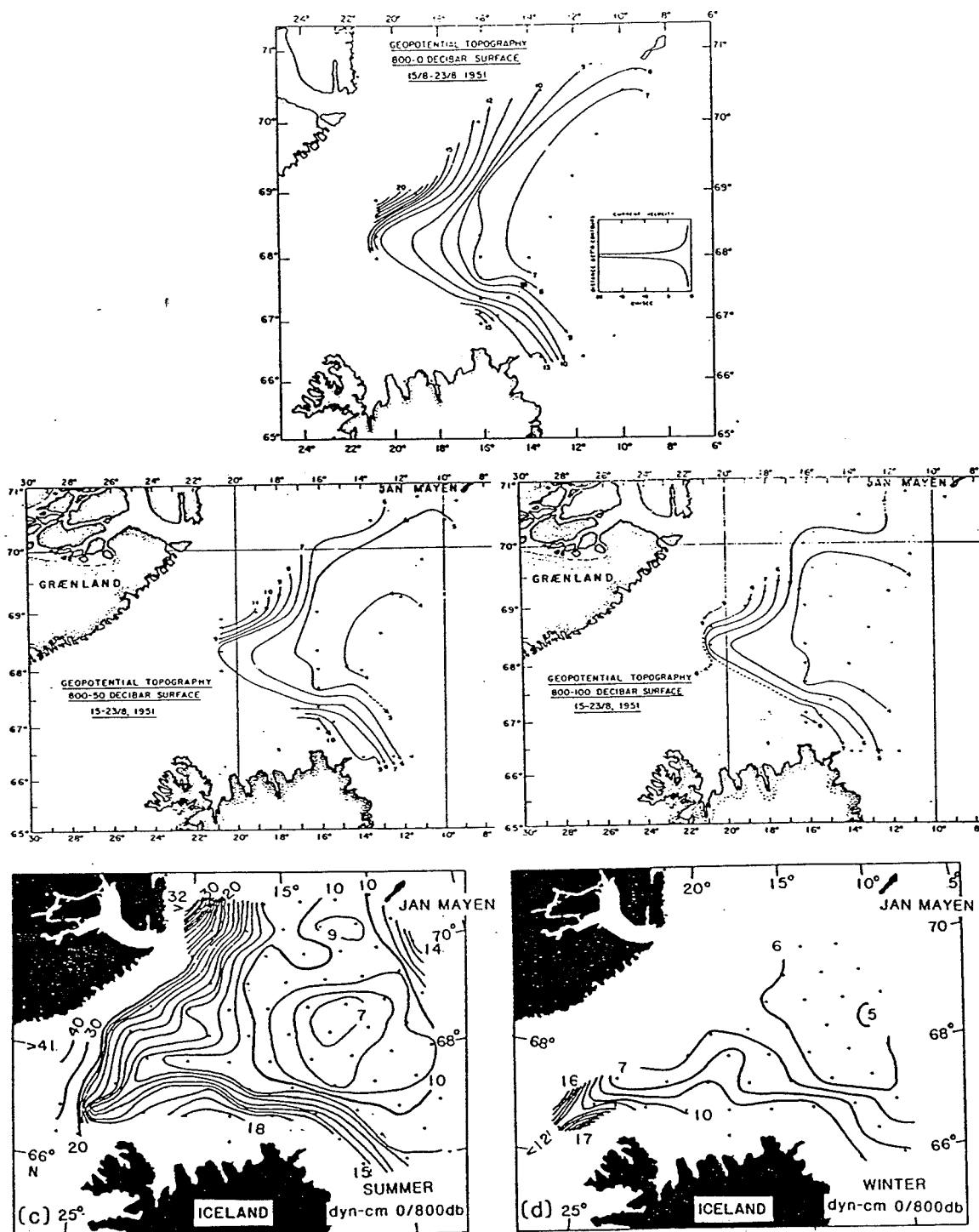
Fig. 3.27 Dynamic topography for Iceland Sea (Hopkins (1988) and Stefánsson (1962))
