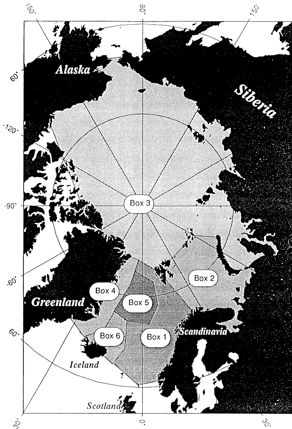
Fig. 4.1 The six areas of the box model.
