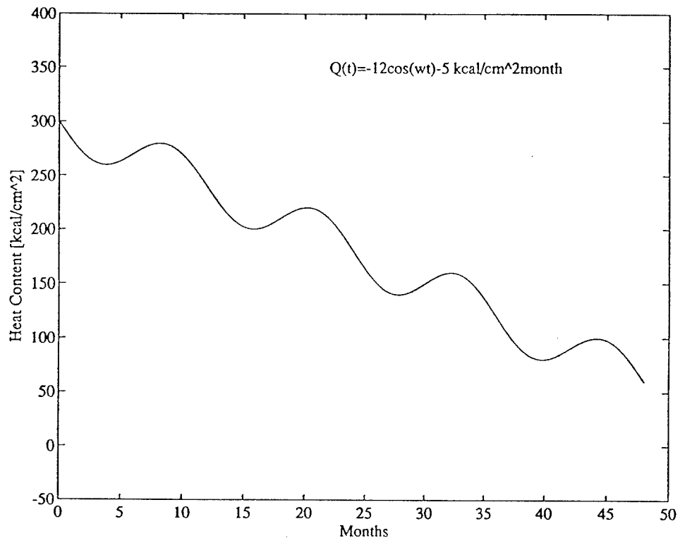
Fig. 5.6 Reduction of heat storage with a net cooling of 75 \text{ W/m}^2
