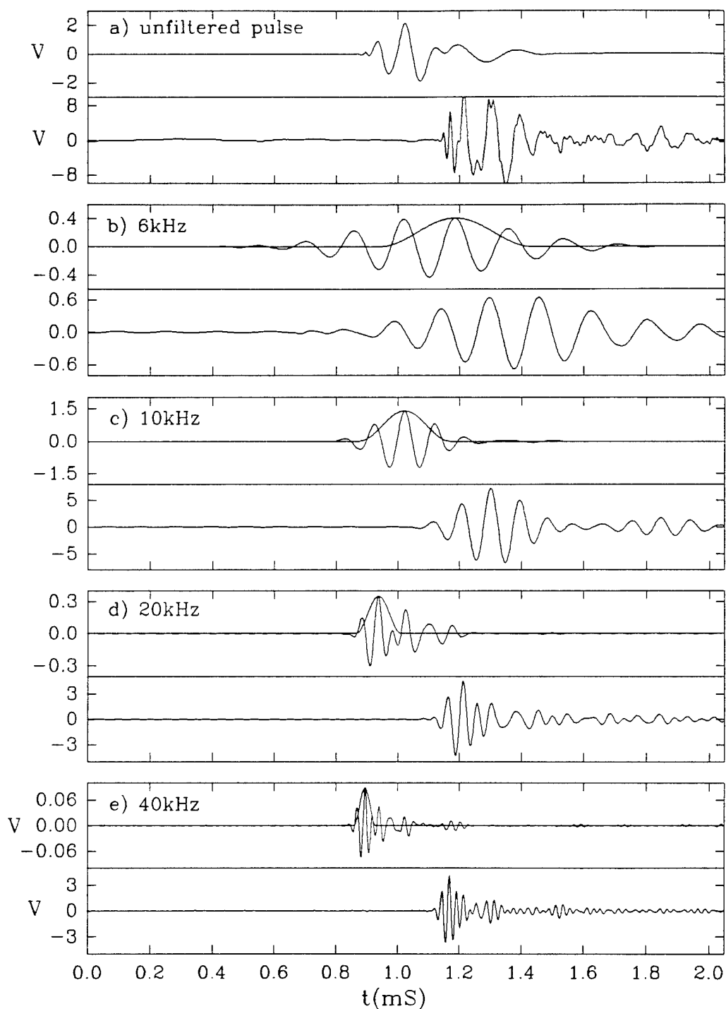
Figure 7.14: a) Transmit (above) and received (below) composite pulses. The filtered version of the composite pulse shown in a) with band-pass filter center frequencies b)6kHz, c)10kHz, d)20kHz and e)40kHz. The window function plotted with each transmit pulses was used to window the signal and thus eliminate the tail-end of the transmit pulses from biasing the cross-correlation function. Woods Hole data.
