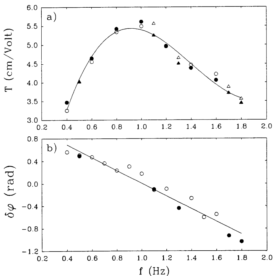
Figure C.2: a) Amplitude and b) phase transfer function for the MIT wavemaker system installed on the wave channel 25m \times 0.7m \times 0.6m. The hollow symbols are for an input amplitude of 0.1V and the filled symbols are for an input amplitude of 0.2V. Transfer function measured on 08-24-90.
