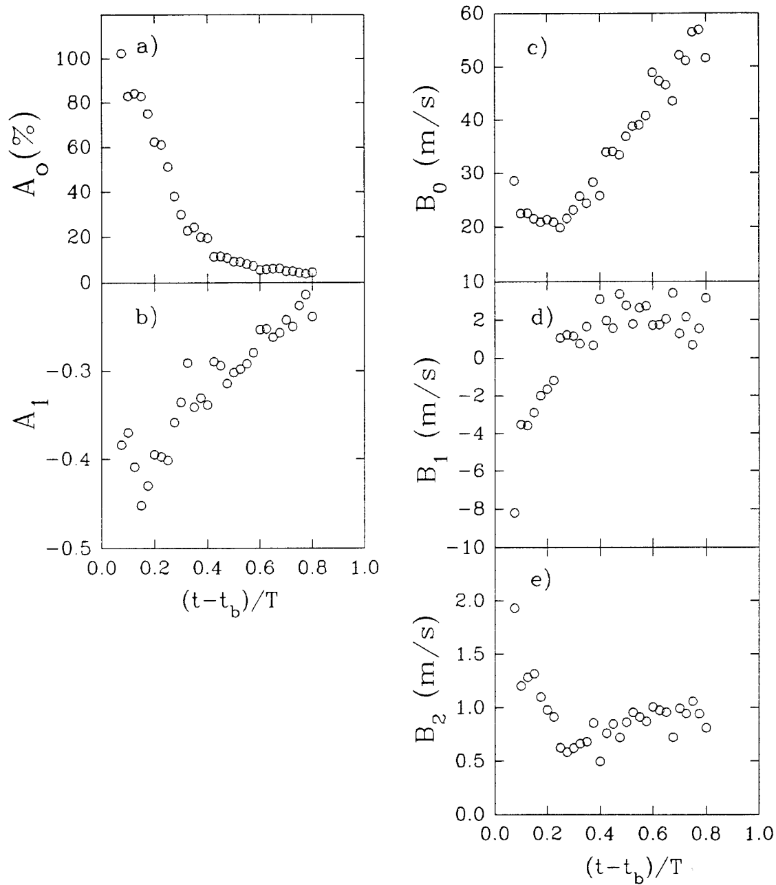
Figure 4.18: The fitting coefficients a) A_0(t) and b) A_1(t) for the exponential equation fitting the void-fraction profile as a function of radius (equation 4.8). Fitting coefficients c) Constant B_0 , d) linear coefficient B_1 and e) second order coefficient B_2 as a function of time for the sound-speed profile fitted by equation 4.9.
