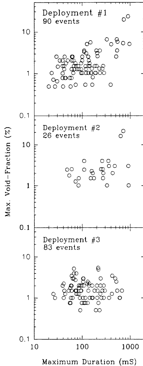
Figure 5.4: Scatter plots of event duration versus maximum void-fraction for a) deployment #1, b) deployment #2 and c) deployment #3. Each deployment has a duration of 155 minutes. The void-fraction is the maximum to occur for each event observed and the duration is the total time of the event above a threshold of 0.5% void-fraction. Note that one breaking wave may lead to multiple events (see figure 5.3c) so the duration should not be interpreted as the duration of a single breaking wave.
