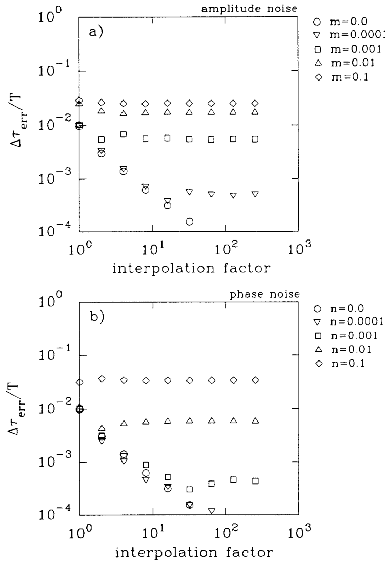
Figure E.3: Error \Delta\tau_{\text{err}}/T in the resolution of the location of the peak of the cross-correlation function versus the interpolation factor. T is the acoustic wave period. The number of samples per period is 100 and the number of points used in the spline is 5. a) effect of amplitude noise only, b) effect of phase noise only. The amplitude noise m and the phase noise n are shown on the graph
