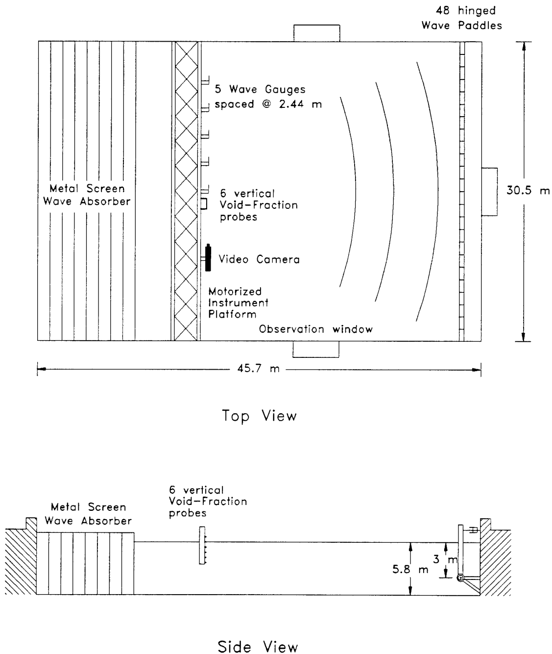
Figure 4.1: Top and side view of the multi-directional wave basin facility at the Offshore Technology Research Center (OTRC). The radial lines sketched in the top view represent the wave crests.
