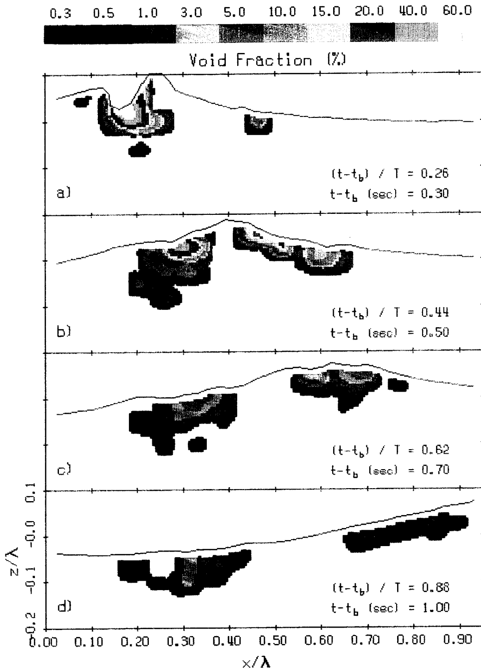
Figure 3.8: Contour maps of the void-fraction field for the most energetic breaker studied. Time evolves from a) through d). The wave moves from left to right. Each frame is constructed from approximately 170 ensemble averages of three runs. Note the distinct downstream cloud generated by the splash from the initial impact at breaking.
