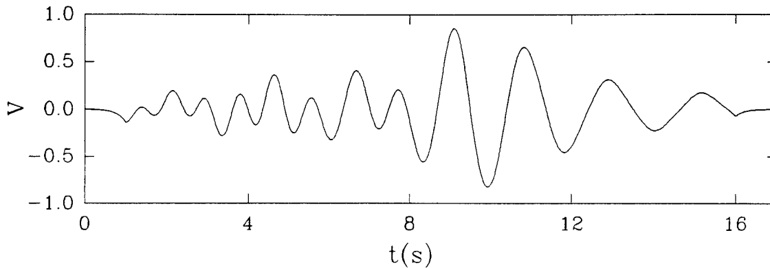
Figure C.1: Computed breaking wave packet used in the 2D experiment of §3. High frequency waves are generated first followed by lower frequency waves. Dispersion ensures superposition at a predetermined position x_b from the wave paddle. A PC equipped with a Metrabyte Das20 board performed the D/A at a conversion rate of 100Hz. The analog signal was fed to the input of the wavemaker system. Note that the packet shown has been corrected for the wavemaker transfer function.
