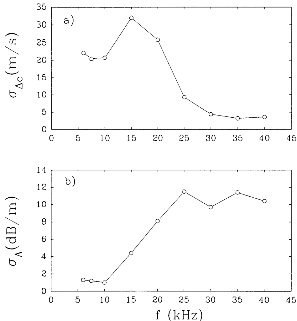
Figure 7.20: Standard deviation of a) the sound-speed anomaly \sigma_{\Delta c} and b) attenuation \sigma_A as a function of frequency. The standard deviations were computed over the 20min time-series shown in figure 7.17 and figure 7.18.
