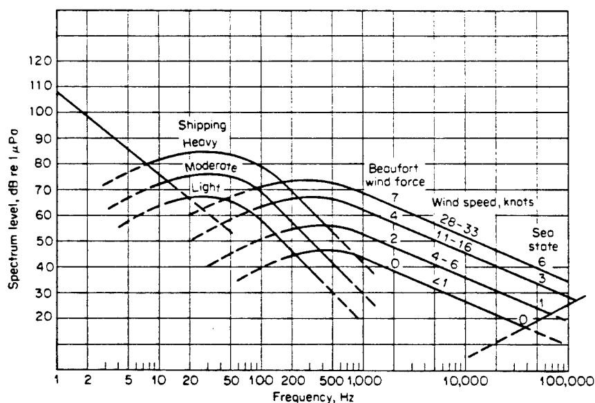
Figure 1.5: Average deep-water ambient-noise spectra. From Urlick [1975].
