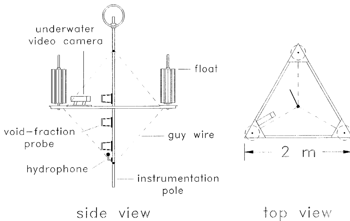
Figure 5.1: Line drawing of the buoy and associated instruments.
