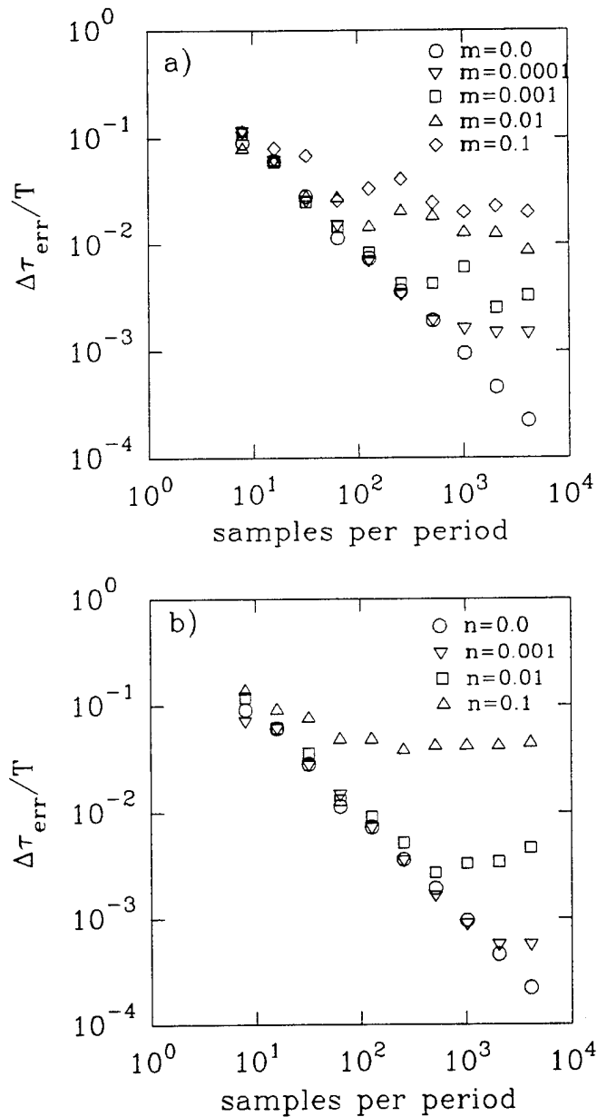
Figure D.2: Error \Delta\tau_{\text{err}} on the resolution of the location of the peak of the cross-correlation function normalized by the acoustic wave period T . The sampling rate is expressed as the number of data samples per period. a) Amplitude noise A_m and b) phase noise \phi_n . A 5 point spline interpolation was used in all simulations.
