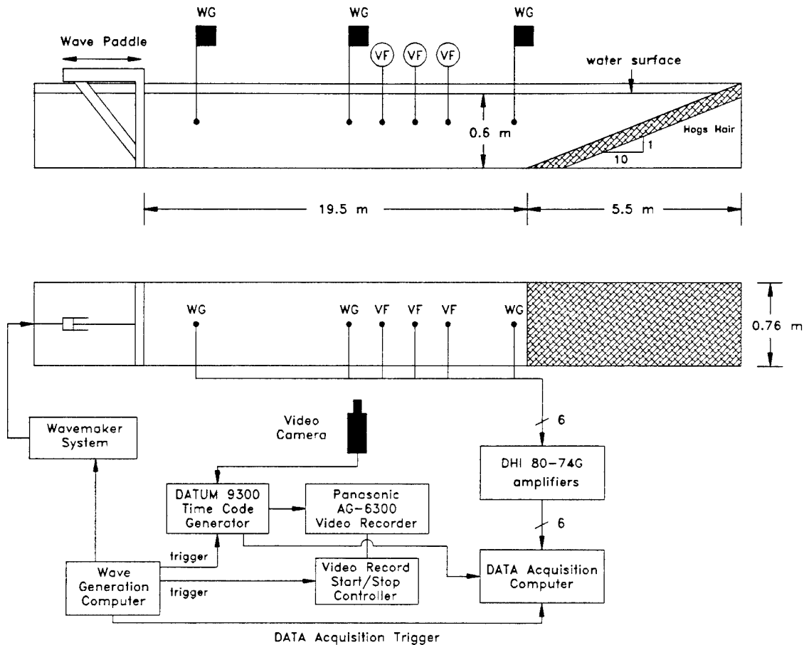
Figure 3.1: Sketch of the experimental facility and the instrumentation setup.
