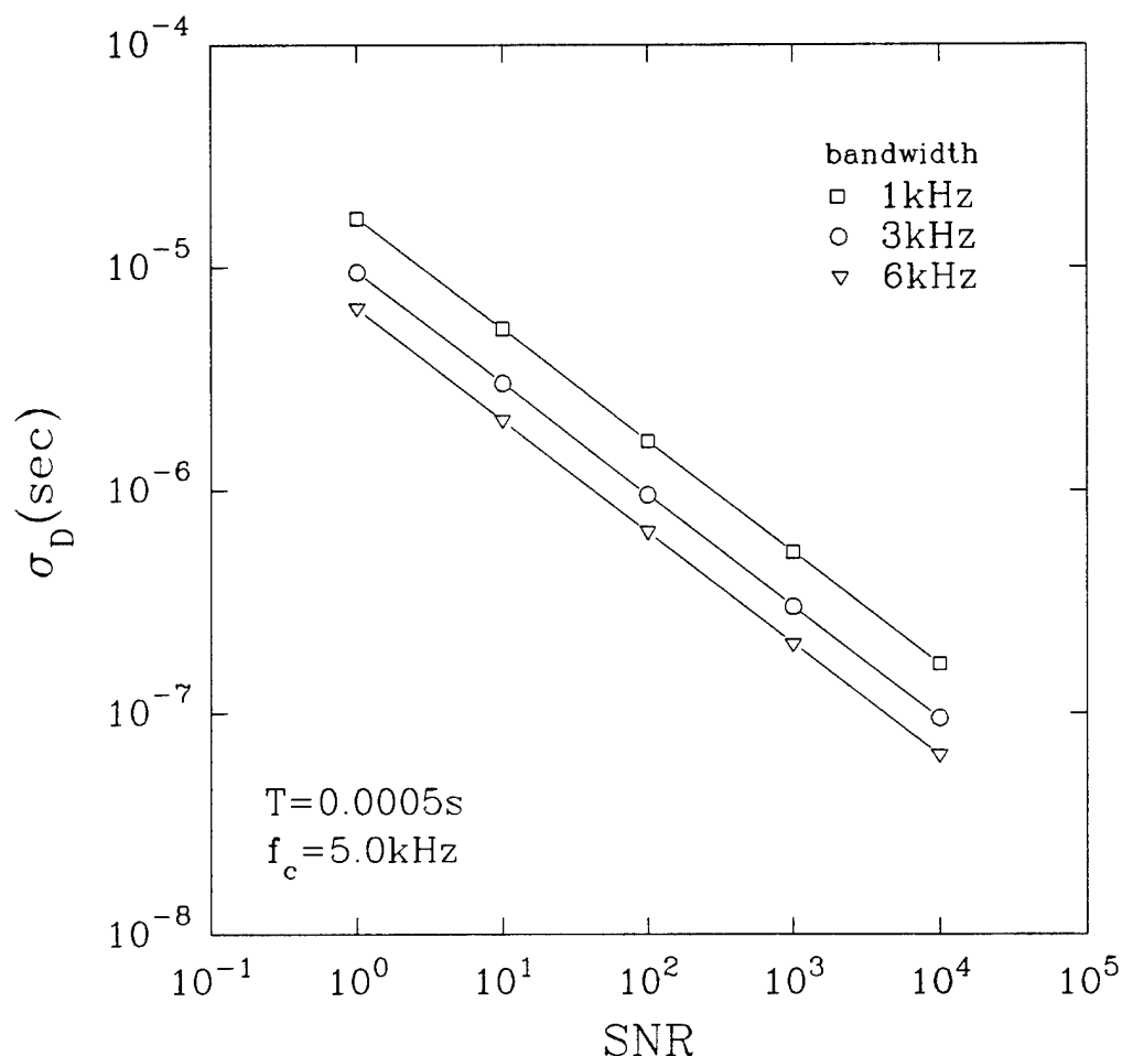
Figure 6.15: Cramer-Rao lower bound on the standard deviation of the time-delay estimate \sigma_b for an observation time T=0.0005s , a signal frequency f_c=(f_1+f_2)/2=5kHz and a signal bandwidth f_2-f_1=3kHz . Note that results are also shown for 1kHz and 6kHz bandwidths. For the laboratory, SNR \sim 1000 and in the field SNR \sim 100 .
