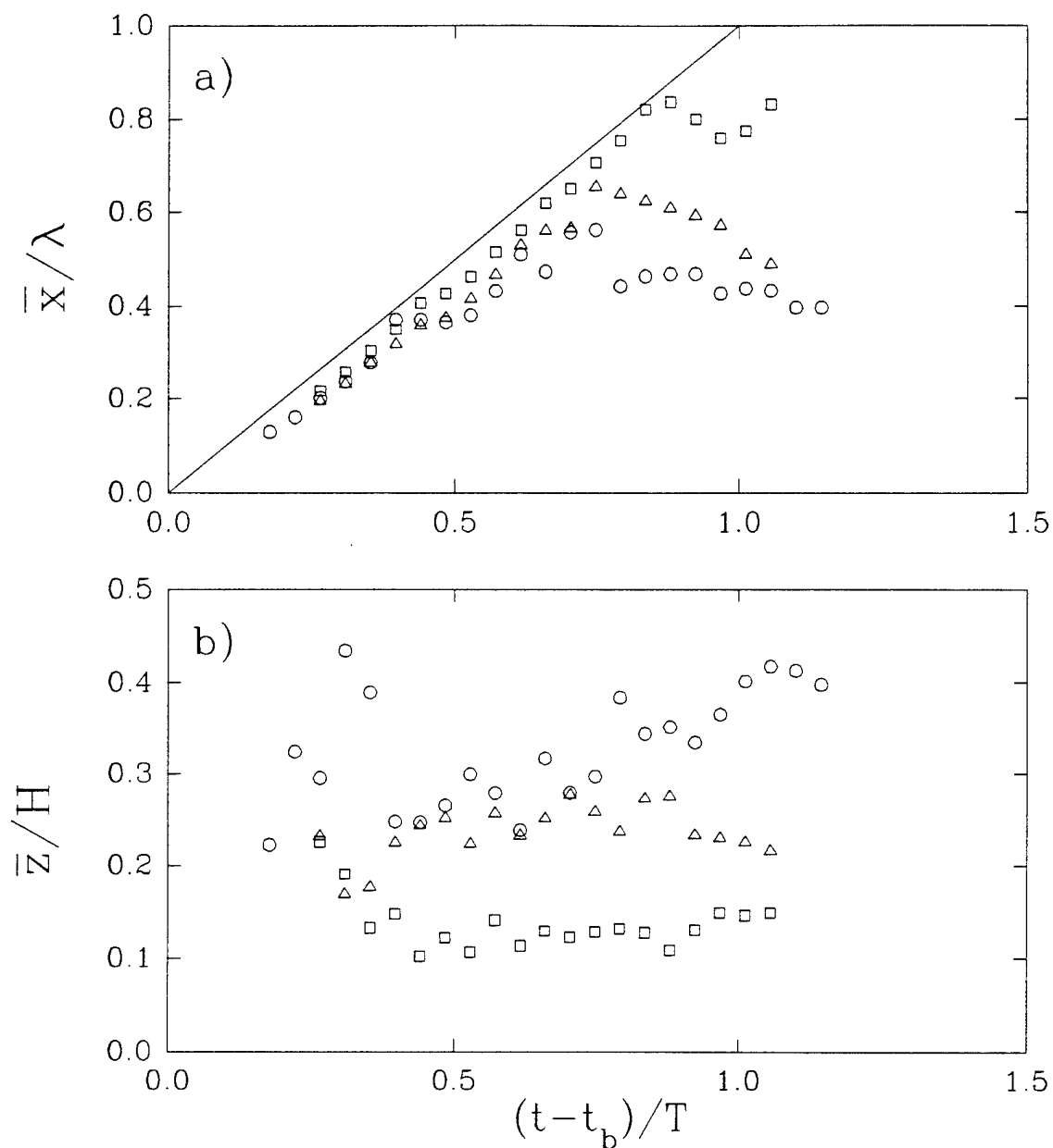
Figure 3.10: Centroids of the bubble plume. a) Horizontal centroid \bar{x} of the bubble plume normalized by \lambda=1.94\text{m} , the characteristic wavelength of the wave packet. b) Vertical centroid \bar{z} normalized by H the height of the wave at breaking (see table 3.1). Solid line is the phase speed of the wave C = \lambda/T . Symbols are S=0.54 (O), S=0.45 ( \square ) and S=0.38 ( \Delta ) where S is defined in table 3.1.
