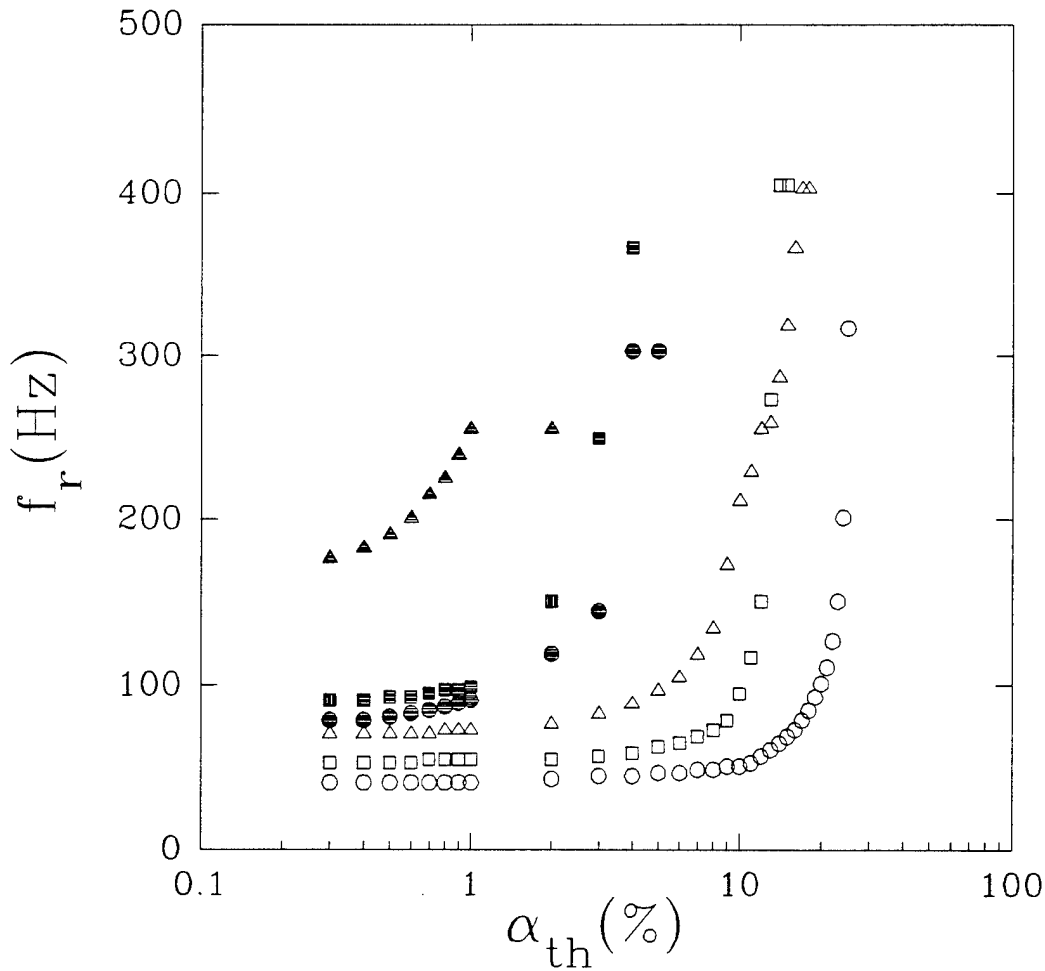
Figure 4.15: Frequency f_r of the collective oscillations of the bubble plume as a function of the void-fraction detection threshold \alpha_{th} for t-t_b = 0.3T (hollow symbols) and t-t_b = 0.8T (solid symbols). G=0.7 (O), G=0.55 ( \square ) and G=0.4 ( \Delta ).
