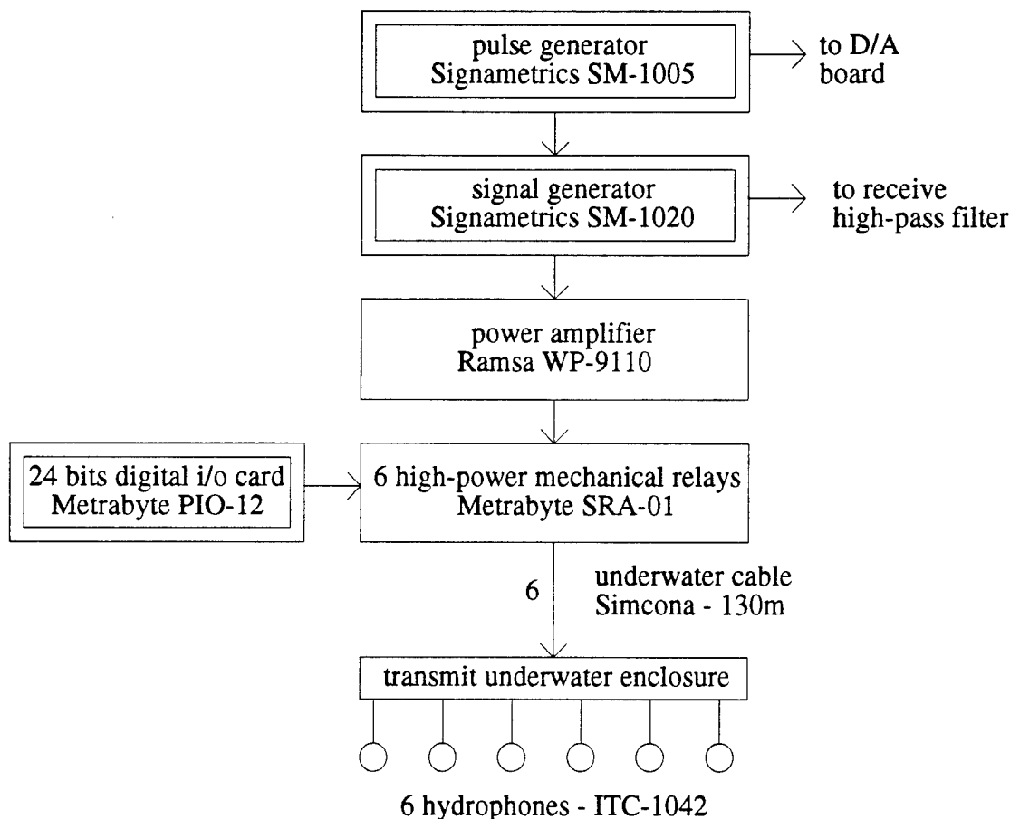
Figure 6.3: Bloc diagram of transmit acoustic system.
