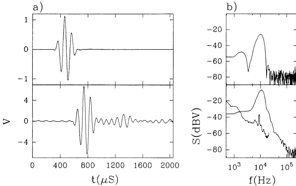
Figure 6.7: a) time-series of transmit (above) and receive (below) 10kHz acoustic pulses. b) Spectrum of time-series in a). Note that the receive time-series was windowed with a 250 point Bartlett window in order to eliminate the reflections from contributing to the spectrum. The second line on the lower spectra is the ambient sound for W_s = 8\text{m/s} .
