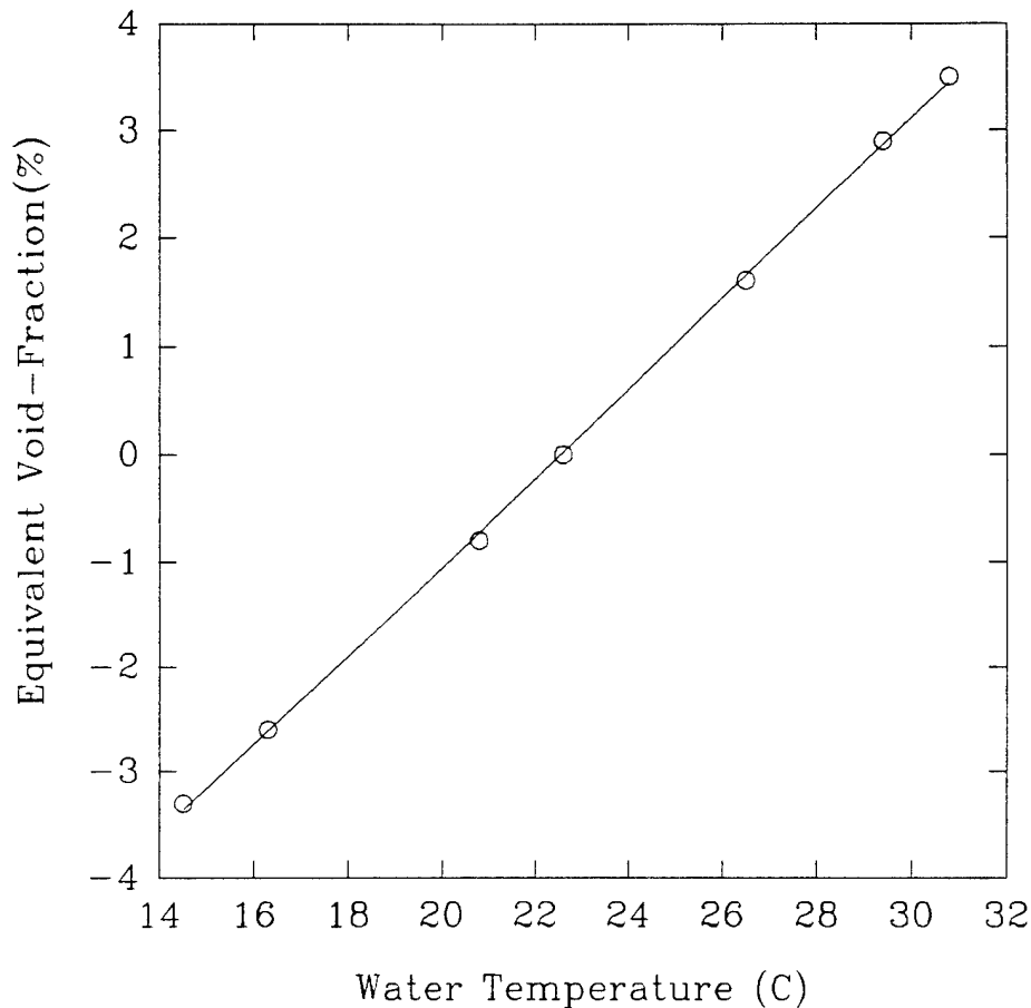
Figure 2.4: Dependence of void-fraction measurement on water temperature. The equivalent void-fraction output from the instrument is plotted as a function of the water temperature. The zero point has been arbitrarily set at 22.6°C.
