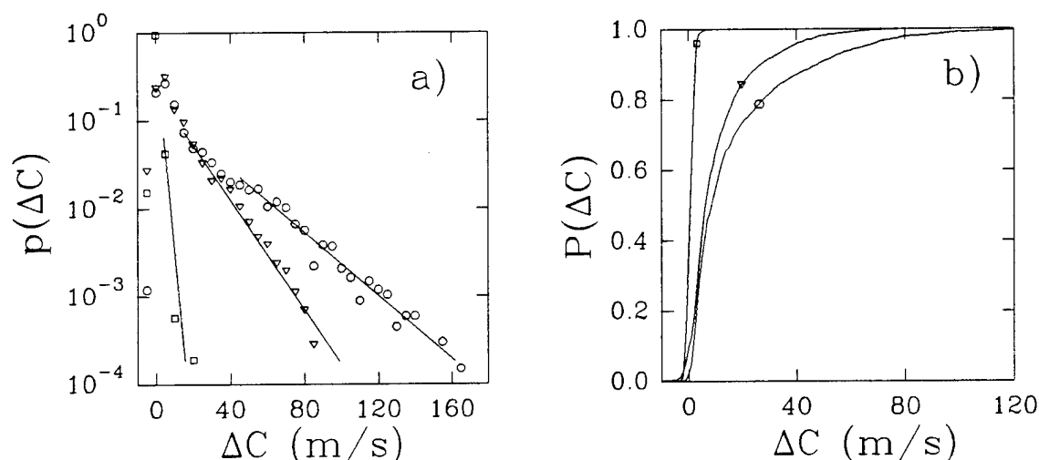
Figure 7.10: a) Probability distribution for three different wind conditions. Each distribution was obtained from three 20min time-series. (o) 7.5 to 8m/s (WH), (v) 5.5 to 6m/s (SD), (□) less than 3m/s (SD) (representative of the noise level). b) Cumulative probability distribution for the same data.
