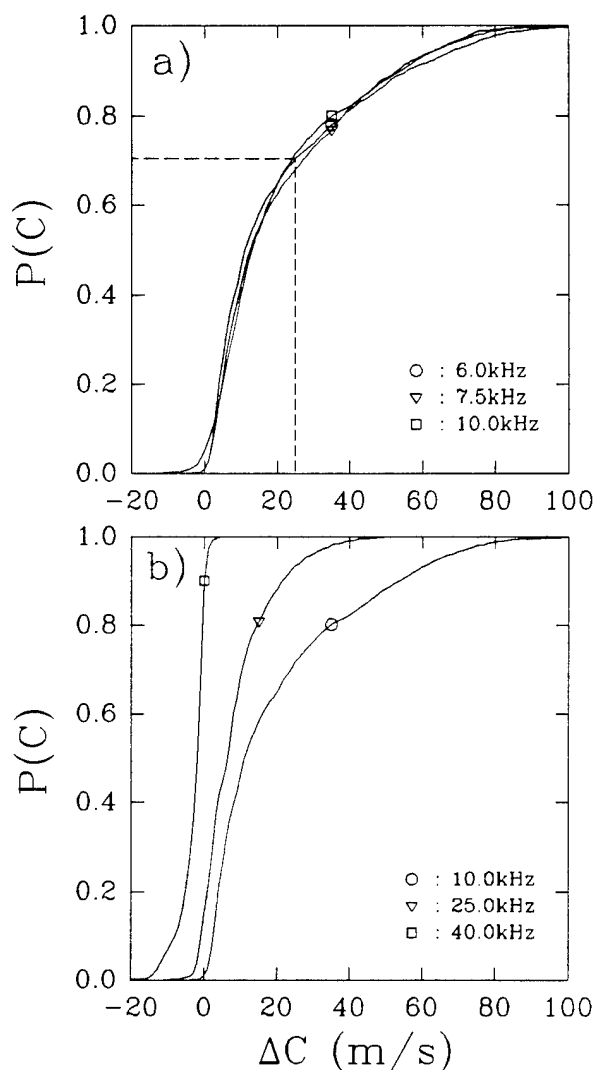
Figure 7.22: Cumulative probability distributions of the sound-speed anomaly at a depth of 0.5m for a) three low frequencies and b) three different frequencies spanning the range of the measurements. The dotted line shows that 30% of the time the signal was above 24m/s. Same data record as the one used in figure 7.17 and figure 7.18.
