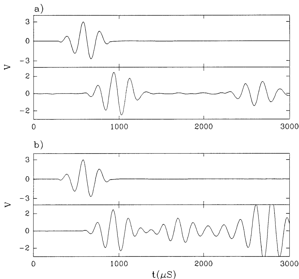
Figure 6.12: Test of acoustic interference by the support module at 5kHz. The experiments were conducted in a tank 3m in diameter and approximately 10m deep. a) The hydrophones were supported as in figure 6.10. b) The hydrophones were mounted on the support module of figure 6.2. The transmit and receive pulses are shown above and below respectively.
