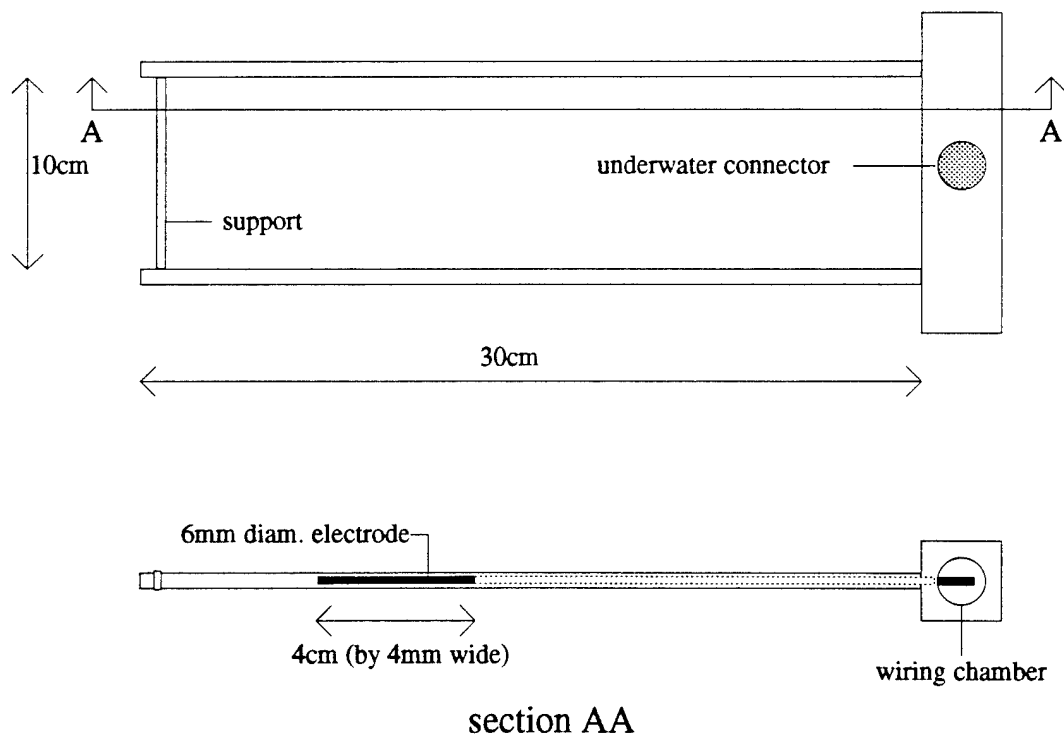
Figure 2.7: Sketch of the field probe used during the SWADE experiment.
