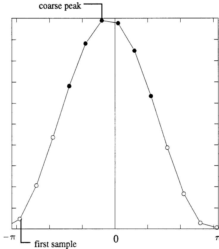
Figure D.1: Model used in the study of the effects of sampling rate and interpolation (discussed in appendix E). The peak of the cross-correlation function is modelled as a half cosine. The symbols represent the actual samples which define the cross-correlation peak. The solid symbols are the data selected for the spline fit (i.e. for interpolation)
