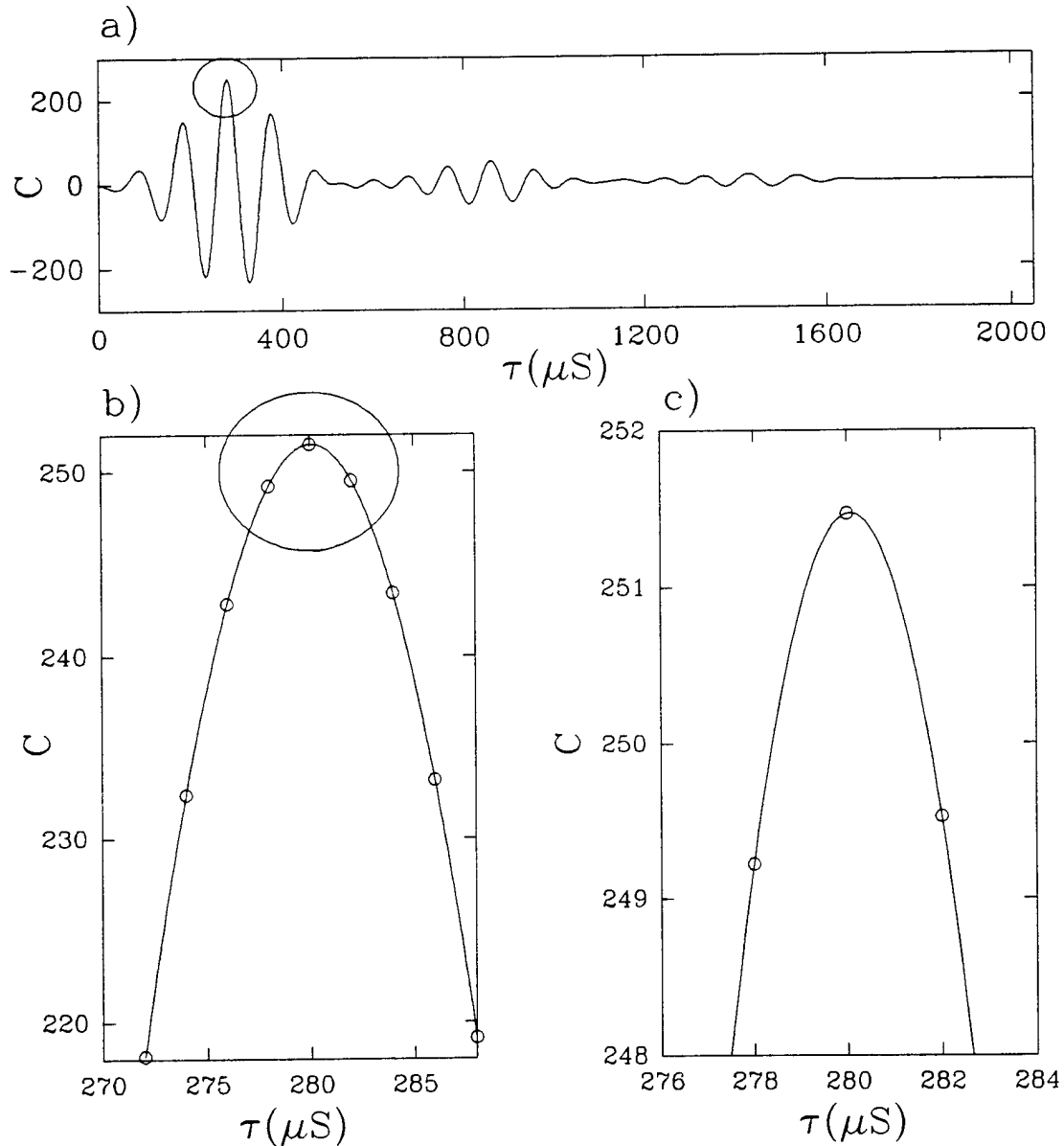
Figure 6.9: a) Cross-correlation function for the time-series in figure 6.7a (i.e. 10kHz pulses). b) Expanded section around the peak of a). c) Expanded section around the peak of b). The data from the cross-correlation are shown as (o) in b) and c). The solid line in b) and c) is the interpolation.
