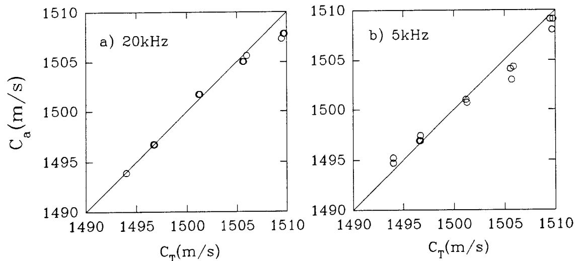
Figure 6.18: Changes in sound-speed caused by changes in temperature. C_T from temperature measurements and C_a from sound-speed measurements. a) 20\text{kHz} , b) 5\text{kHz} .
