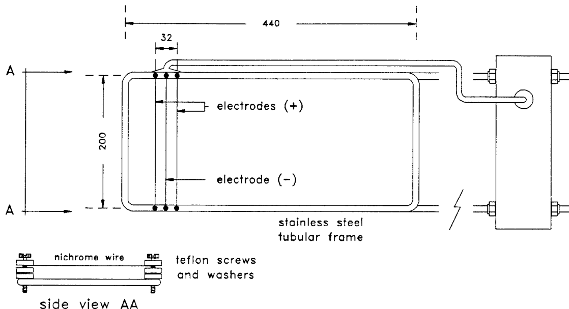
Figure 2.1: Void-fraction probe used in the laboratory experiments.
