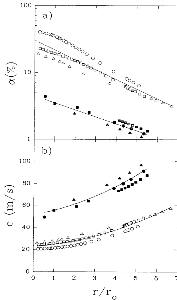
Figure 4.17: a) Void-fraction and b) sound-speed radial profiles for t-t_b = 0.3T (hollow symbols) and t-t_b = 0.8T (solid symbols). G=0.7 (O), G=0.55 (□) and G=0.4 (Δ). Solid lines are best fits based on a) equation 4.8 and b) equation 4.9. The radius is normalized by r_o = \sqrt{v_o/\pi} .
