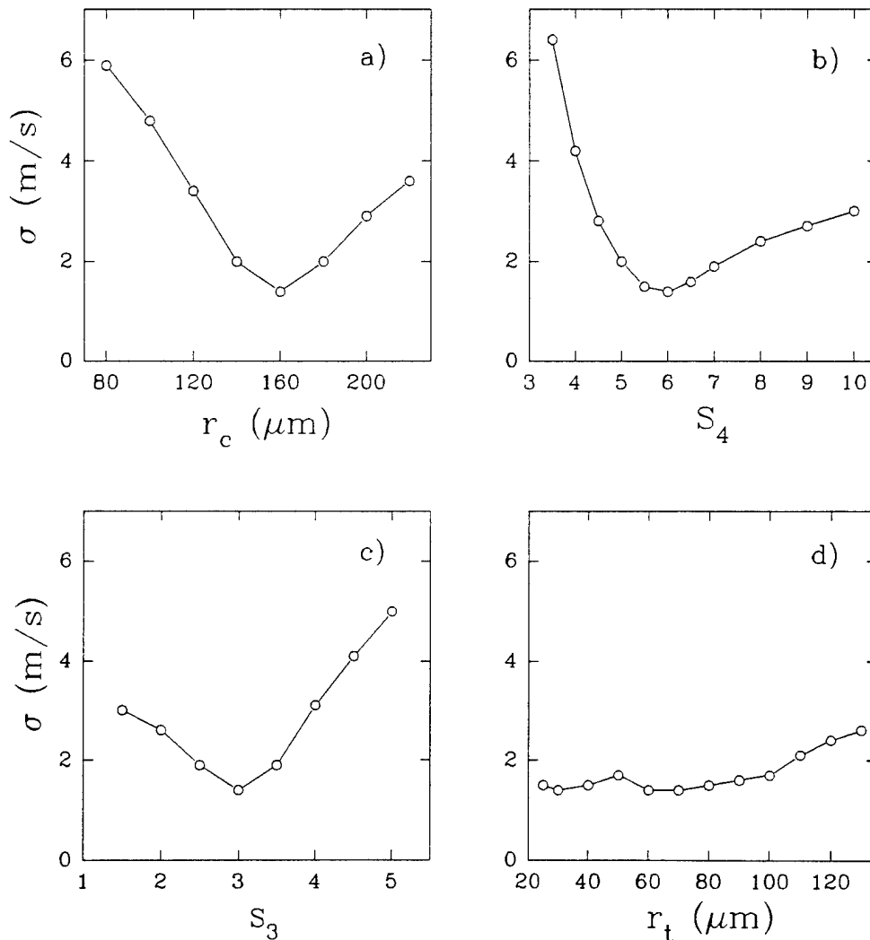
Figure 7.25: Sensitivity to variations in bubble population parameters for a) r_c , b) s_4 , c) s_3 and d) r_t . The standard deviation \sigma between the model and the measurements is given by equation 7.6. In each plot, the default bubble population used is given in table 7.4, and one of its parameters is varied.
