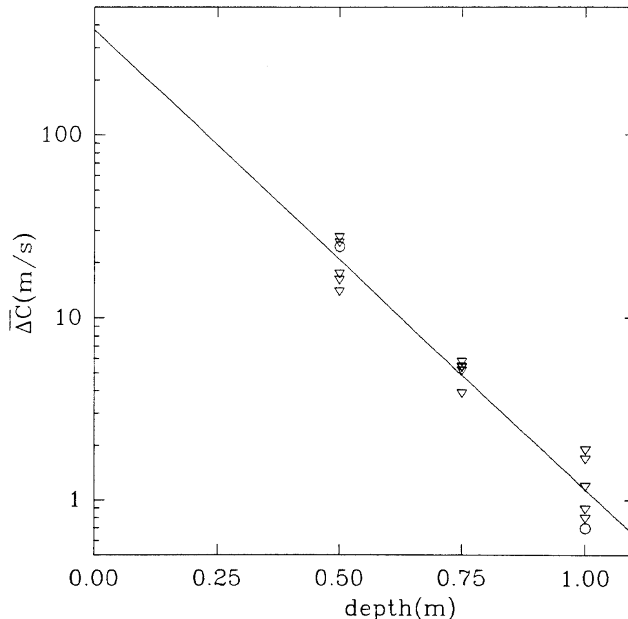
Figure 7.9: Average sound-speed anomaly \Delta\bar{C} as a function of depth. Each data symbol is a 20min average. ( \nabla ) Woods Hole experiment and (o) San Diego experiment. The solid line is the best exponential fit to the data. Wind speed of 7 to 8m/s. The frequency of the acoustic pulses was either 5kHz or 10kHz.
