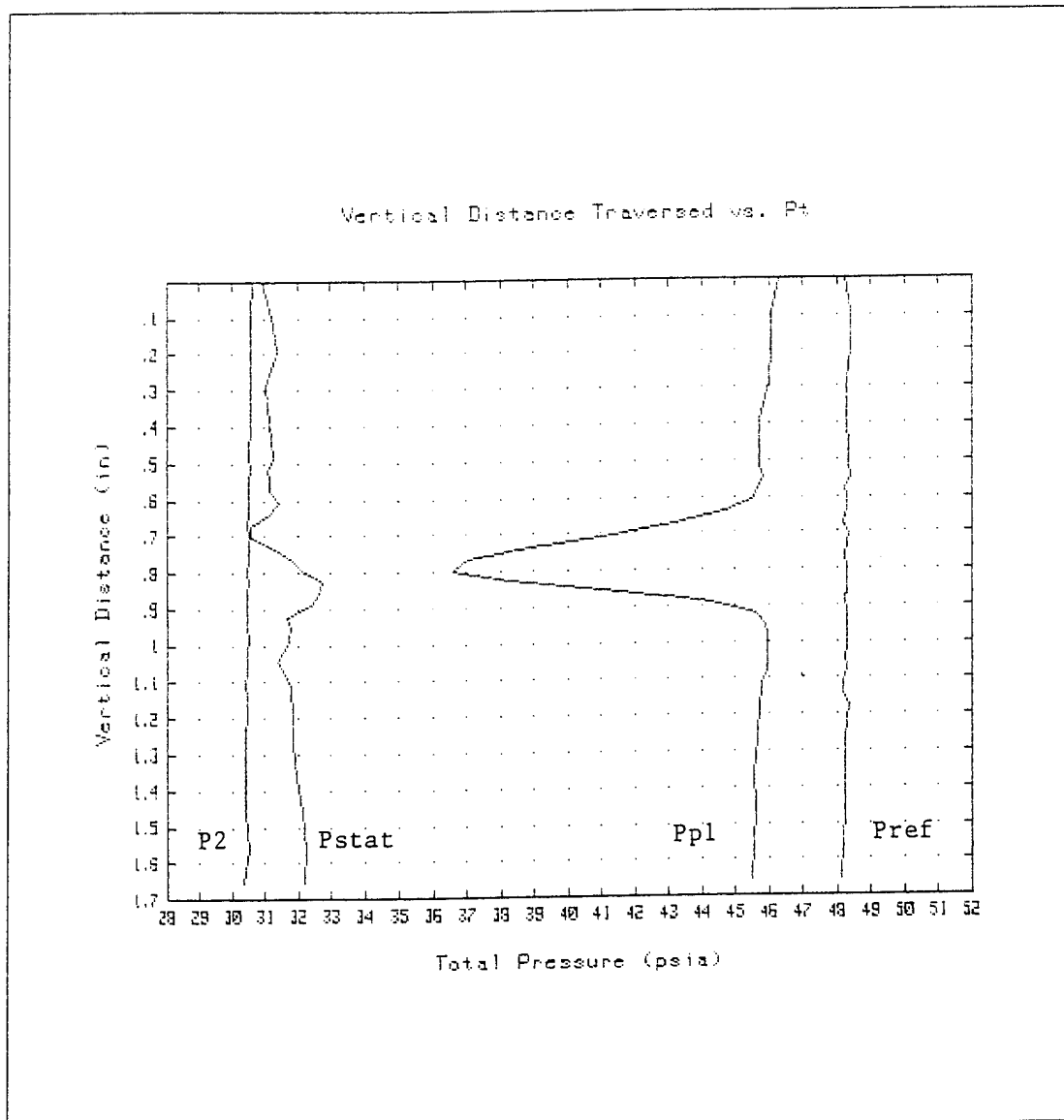
Figure 25. Example Pressure Distribution: Steel Blades Without VGs, Run 1, 2/24/95
