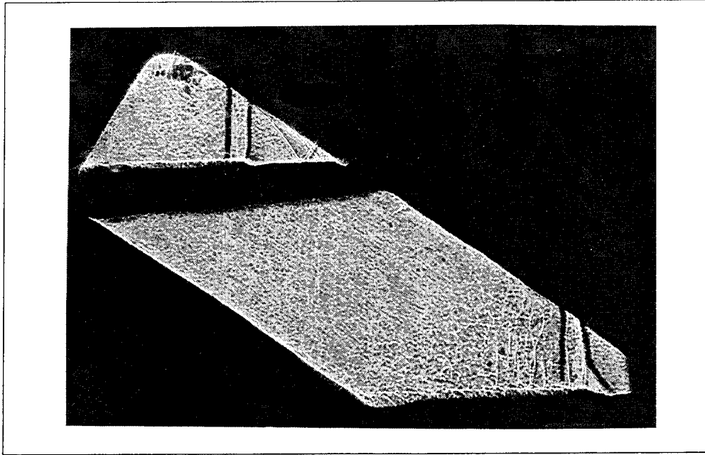
Figure 23. On-Design Shock Positions: Aluminum Blades Without VGs
