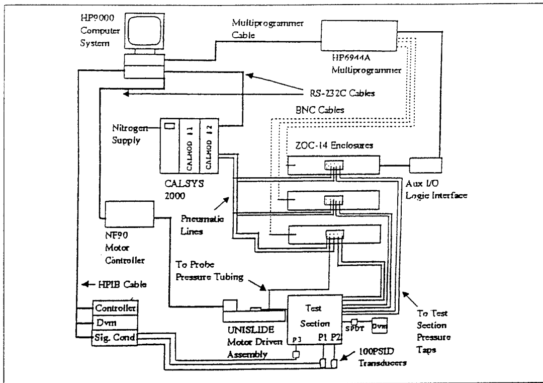
Figure 9. Data Acquisition System Schematic (from Reference 9)
