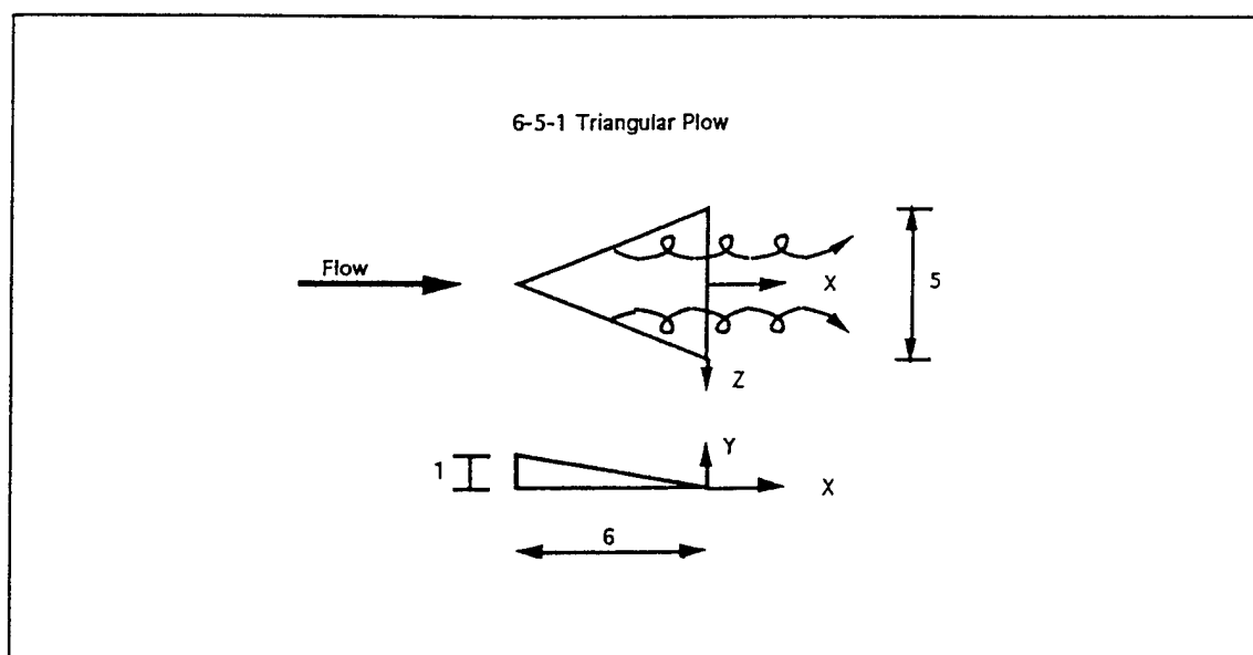
Figure 2. Low-Profile Vortex Generator (from Reference 10)
