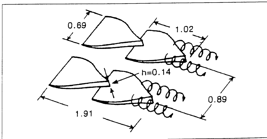
Figure 15. Wheeler-Doublets used by McCormick (from Reference 3)
