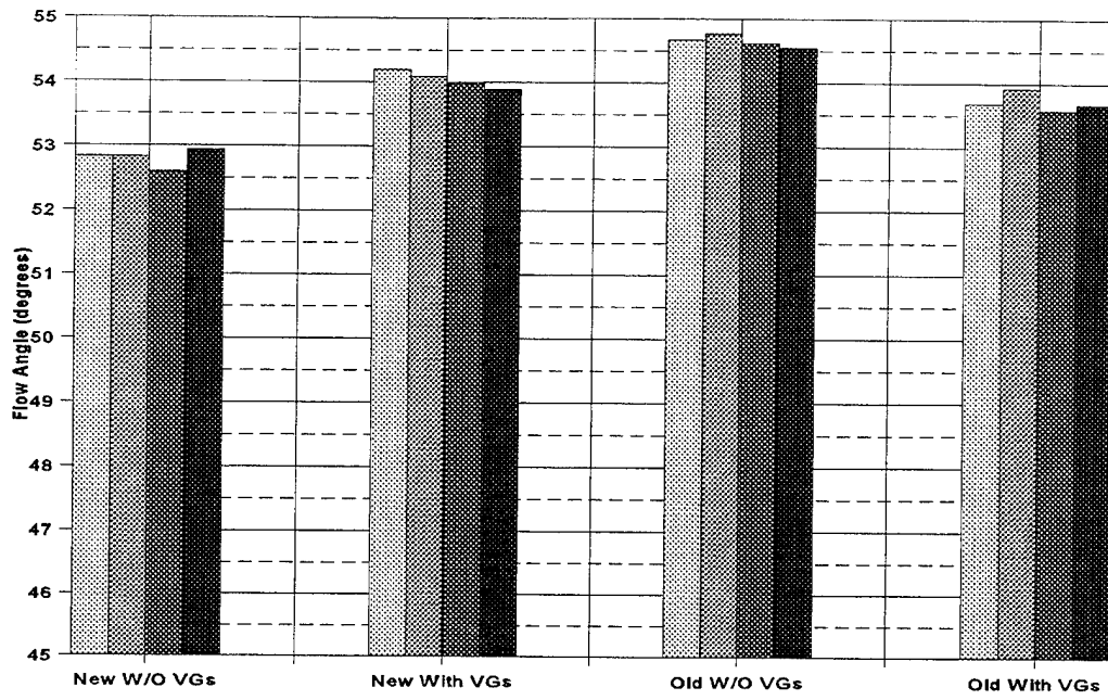
Figure 28. Fully-Mixed-Out Flow Angle ( \beta_3 )
