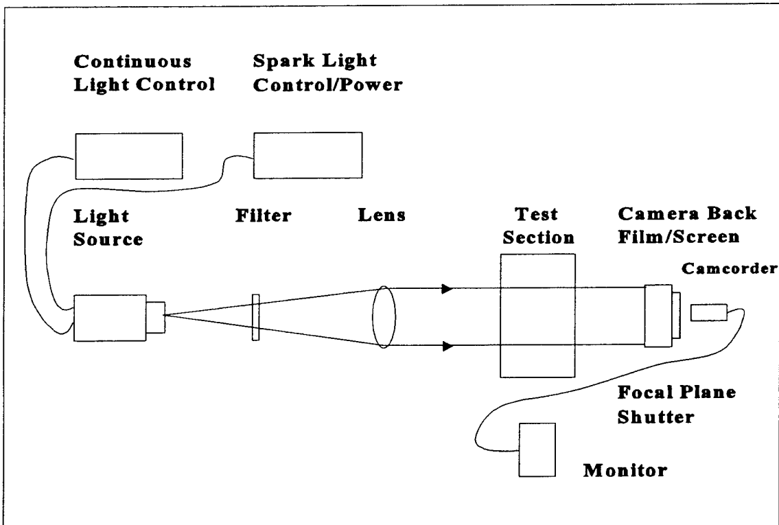
Figure 12. Shadowgraph Visualization System
