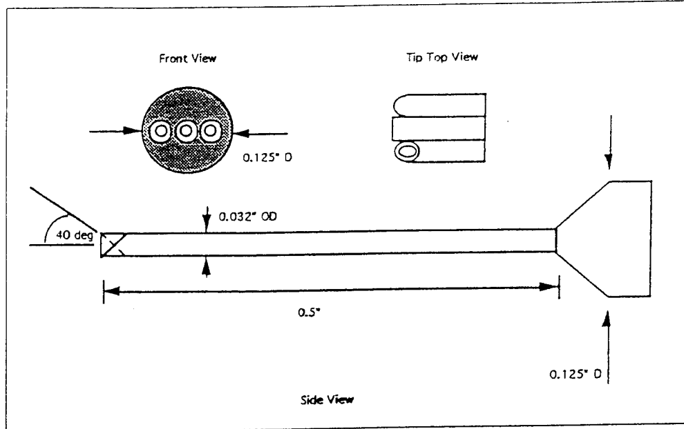
Figure 8. Probe Tip (from Reference 10)
