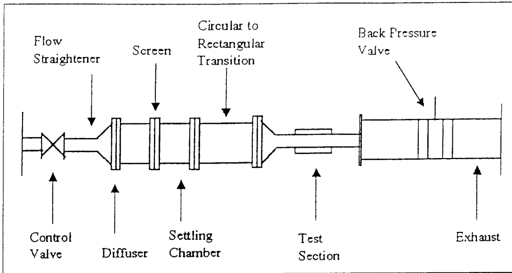
Figure 4. Transonic Wind Tunnel Schematic (from Reference 8)
