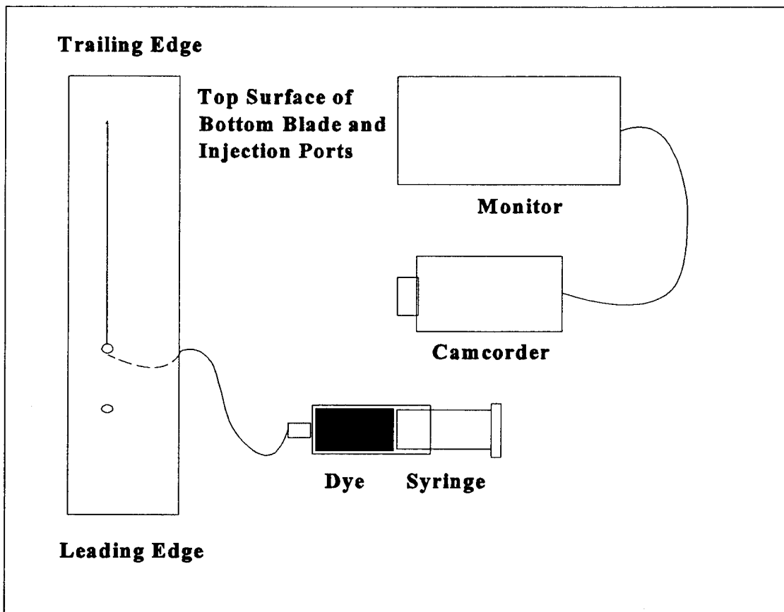
Figure 13. Dye Injection Visualization System
