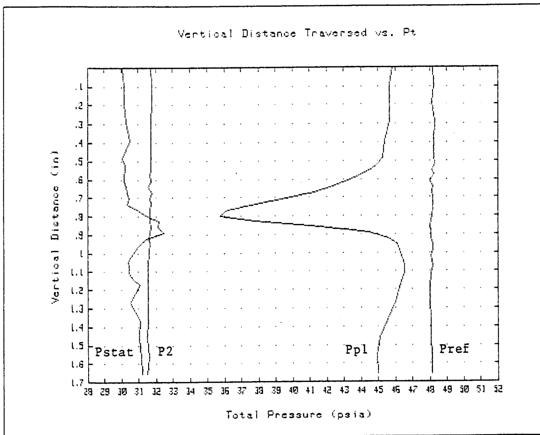
Figure 27. Example Pressure Distribution: Steel Blades With VGs, Run 1, 3/14/95
