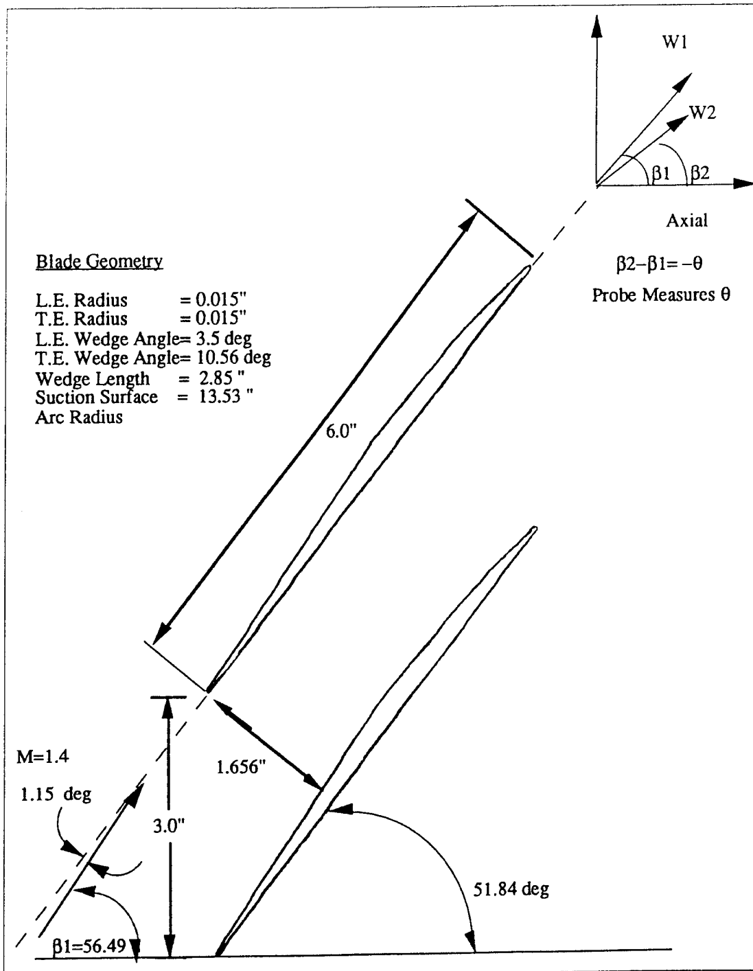
Figure 6. Cascade Blading Geometry (from Reference 10)
