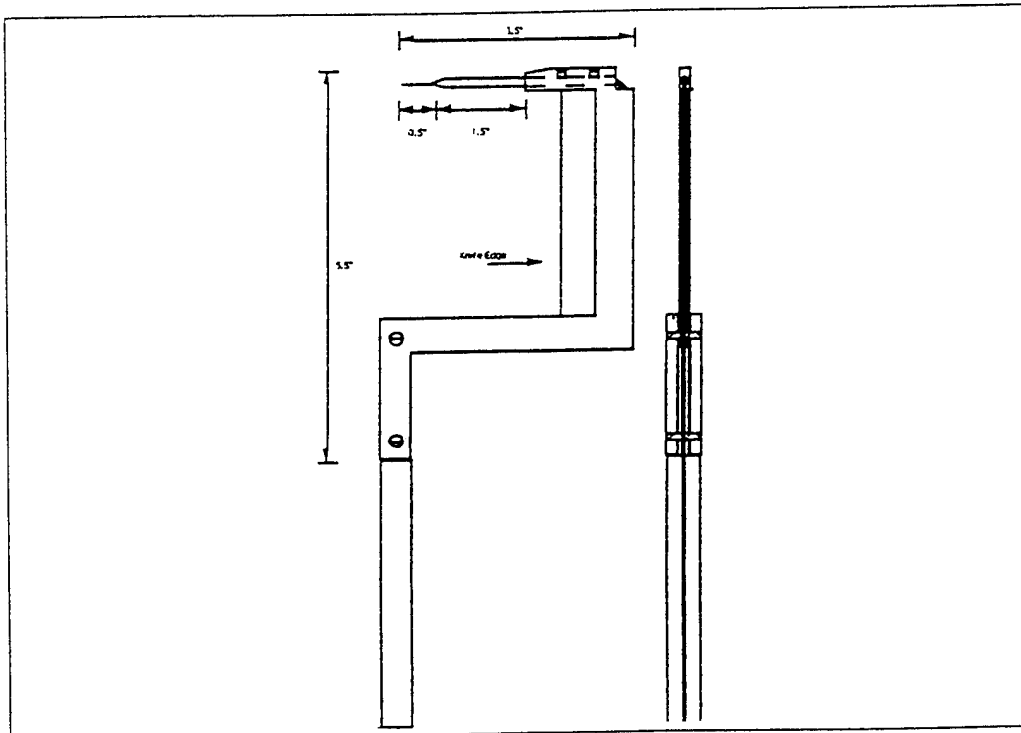
Figure 7. Probe Holder Assembly (from Reference 10)
