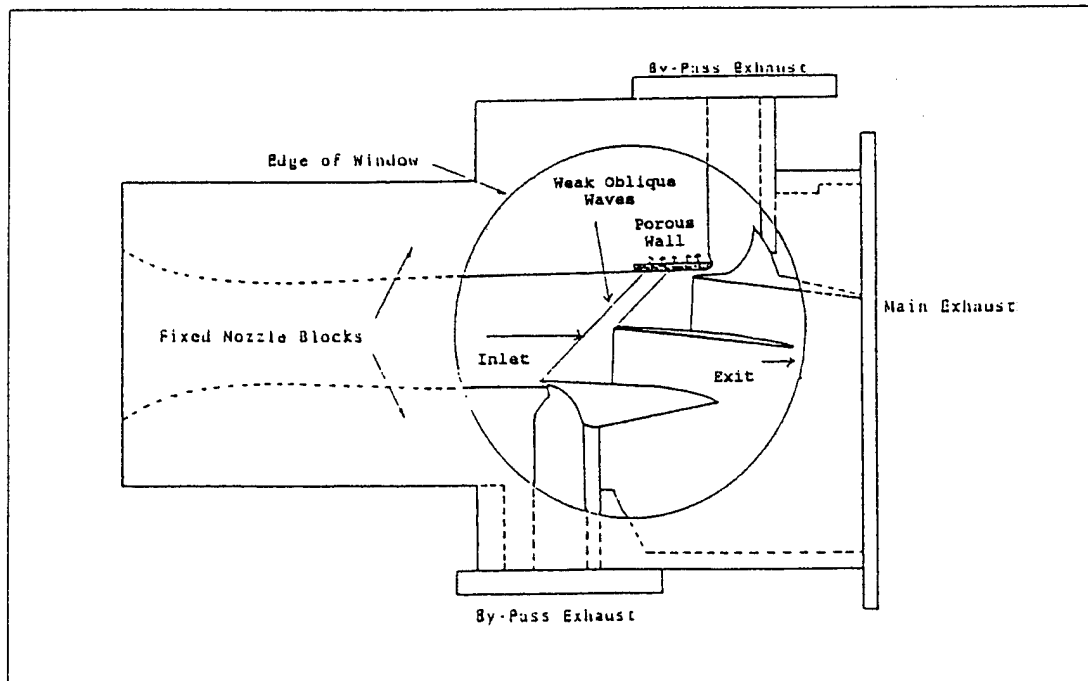
Figure 5. Test Section Schematic (from Reference 7)
