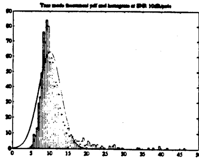
Figure 2: True mode theoretical pdf and histogram for two equal energy undamped modes.
