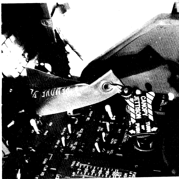
Figure 21. AH-64 pilot emergency egress handle.
