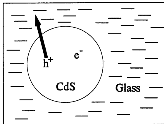
Figure 3. Schematic representation of the mechanism of the photodarkening effect indicating the tunneling of the photogenerated charged carriers out the quantum dot into traps in the glass surrounding the dots, which changes the overall static Coulomb field around the quantum dot.
