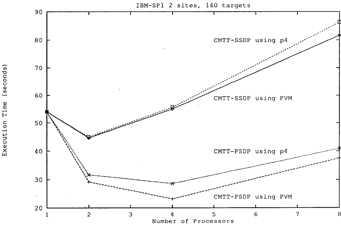
Figure 3: Performance Result of CMTT on IBM-SP1 implemented with p4 and PVM
