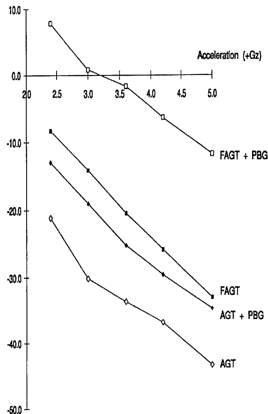
Figure 9. Eye level arterial blood pressure changes under G comparing the use of full coverage anti-G trousers (FAGT) or an in-service garment (AGT) with, and without, the addition of PBG at 30mmHg pressure. From Prior (1991).
