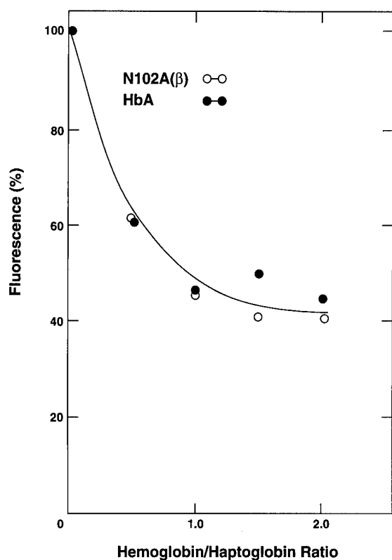
Fig. 6. Quenching of haptoglobin fluorescence by Hb dimers. The quenching of haptoglobin fluorescence as described in the text for various ratios of Hb to haptoglobin shown in the figure.
