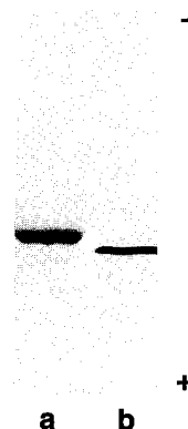
Fig. 2. Isoelectric focusing of N102A( \beta ) mutant Hb. A gel (pH 6–8) (Isolab) was electrophoresed at 10 W for 40 min and stained with 0.2% bromophenol blue. Lane a: N102A( \beta ) mutant Hb; lane b: a natural Hb.
