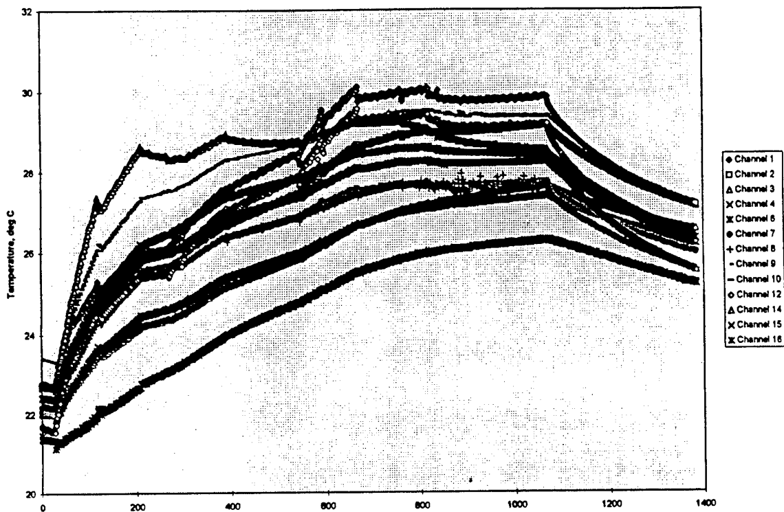
Figure 49. Temperature-time record for pig muscle heating experiment. The pig muscle contained significant amount of fatty tissue. Power was turned on at 33 seconds and pseudo steady-state condition was reached at 1030 seconds. The power was turned off at 1130 seconds.
