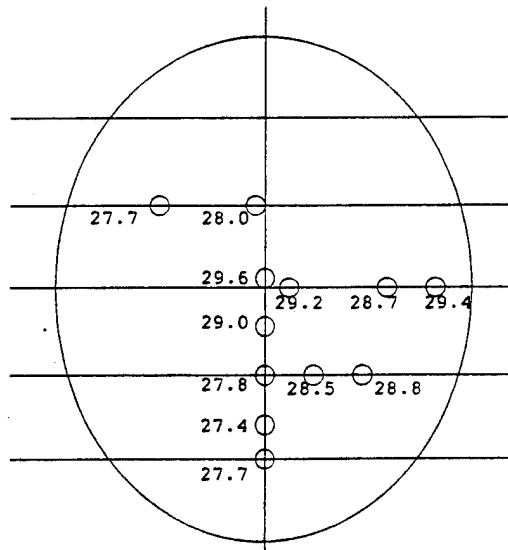
Figure 50. Cross-section of the elliptical pig muscle phantom shown with the probes and measurement points. Both low and high frequencies were used. The temperatures ranged from 27.4°C to 29.6°C.
