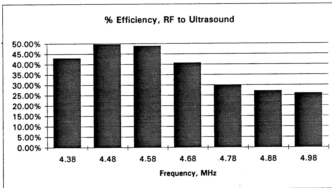
Figure 5. Acoustic efficiency as a function of frequency for a typical 4.5 MHz transducer used in the cylindrical array. Similar data exists for each of the 384 transducers.
