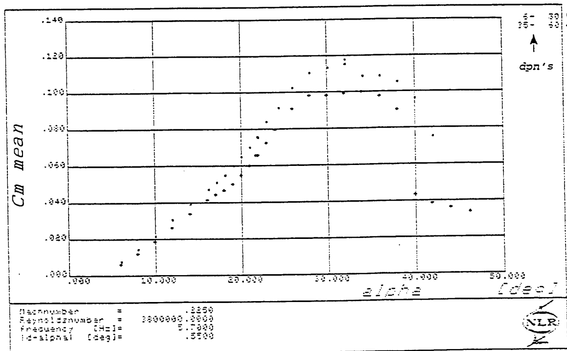
Figure B.2 Cm mean versus incidence with (■) and without (◆) filler plate
