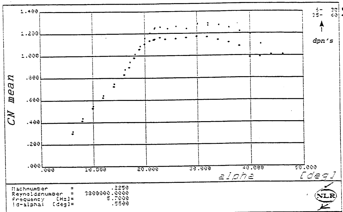
Figure B.1 CN mean versus incidence with (■) and without (◆) filler plate
