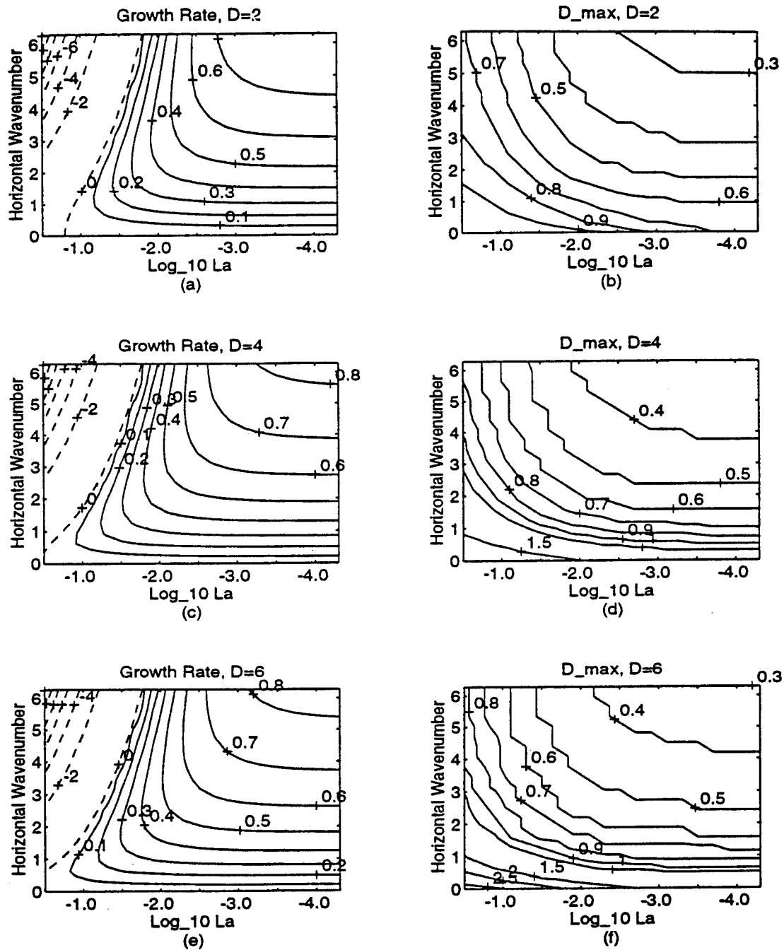
Figure 2.2: Growth rate and depth of maximum vertical velocity D_{\max} as a function of horizontal wavenumber and Langmuir number given monochromatic waves, no Coriolis force, and a surface Eulerian shear =1. Waves, wind and cell axis are assumed collinear. (a) Growth rate, Layer depth D=2 . (b) D_{\max} , D=2 . (c) Growth rate, D=4 . (d) D_{\max} , D=4 . (e) Growth rate, D=6 . (f) D_{\max} , D=6 .
