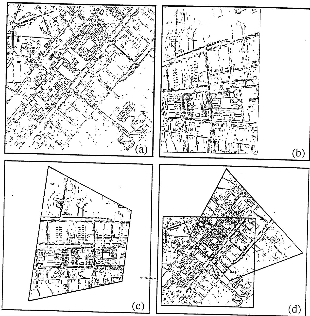
Figure 13: Image-to-image matching example on an aerial image: (a) image lines from nadir view, (b) image lines from oblique view, (c) rectified oblique view, (d) registration of nadir view with rectified oblique view.
