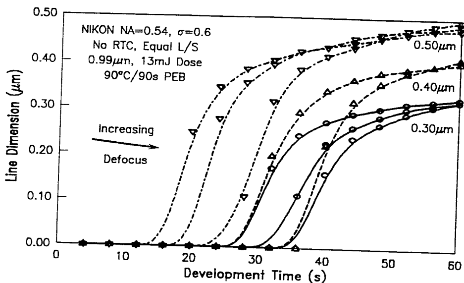
Figure 8. MCP Simulated Line Width Time Evolution of APEX-E on Si. Line width as a function of time and focus at 13\text{mJ}/\text{cm}^2 for APEX-E on Si.
