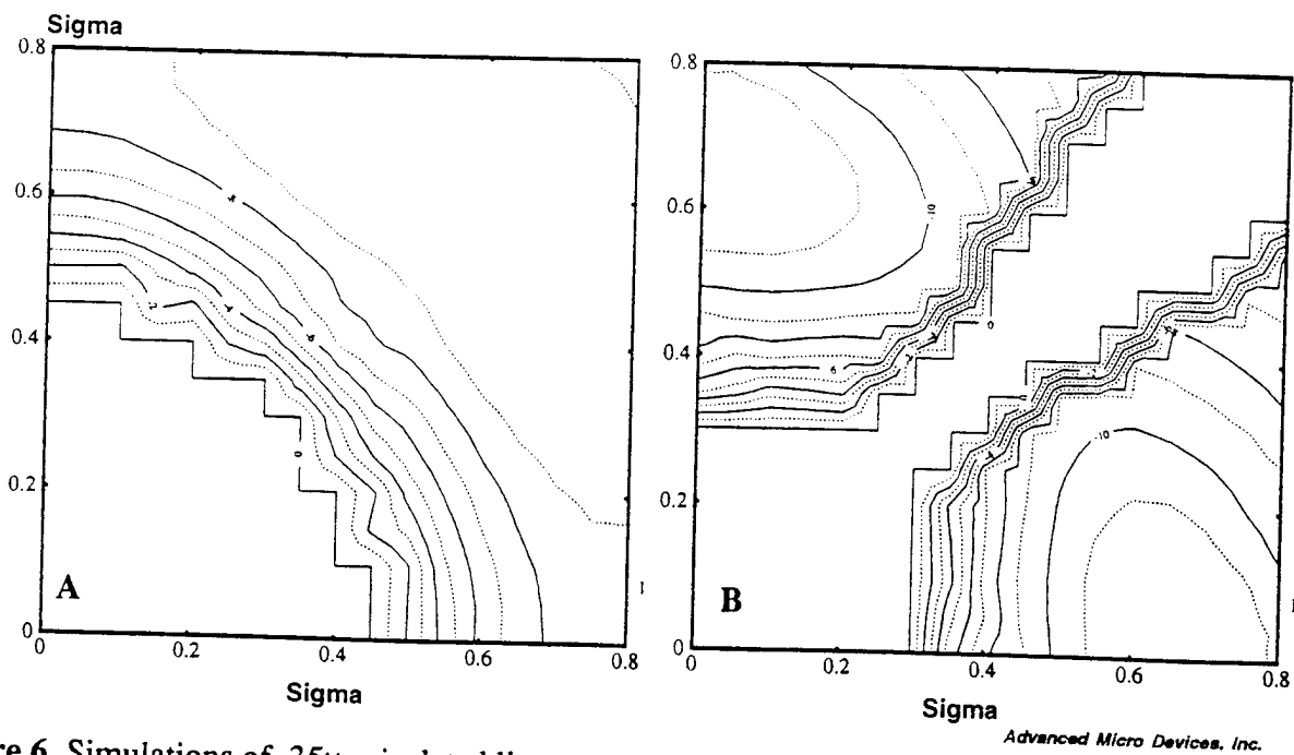
Figure 6. Simulations of .35μm isolated line exposure latitude at .9μm defocus for i-line systems with fixed NA of .48 and various illuminator configurations: (A) annular illumination; and (B) quadrupole illumination.
