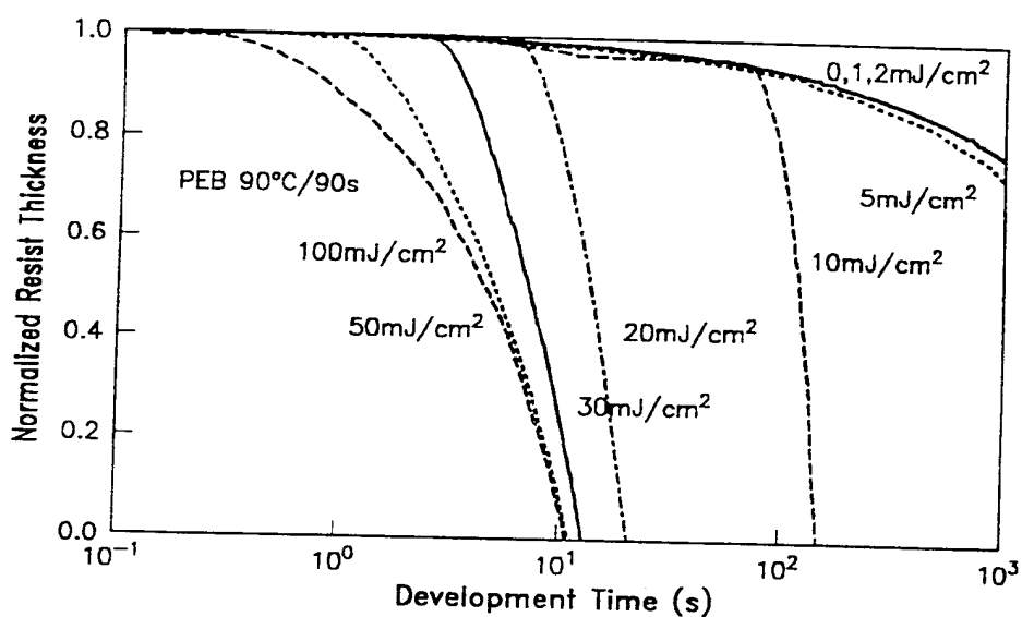
Figure 1. DRM Thickness Curve of APEX-E. Normalized APEX-E resist thickness as a function of development time and dose for a 90°C/90s PEB. Initial thickness was 0.99µm on Si exposed on a Canon FPA 4500.
