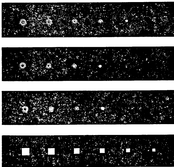
FIG. 6. The aerial image of contact holes of varying sizes, at 0.5- \mu\text{m} defocus, obtained with three exposure systems (from top to bottom): 193 nm, 0.5 NA, \sigma=0.6 ; 248 nm, 0.5 NA, \sigma=0.6 ; 248 nm, 0.5 NA, annular illumination with normalized inner and outer radii of 0.4 and 0.6; the ideal image (the reticle pattern, scaled down by 4 \times ). The nominal hole sizes are (from left-to-right): 0.4, 0.35, 0.3, 0.25, 0.2, and 0.15 \mu\text{m} . Note that only the 193-nm system can print 0.25- \mu\text{m} contacts, and that annular illumination has little effect on the aerial image of these features.
