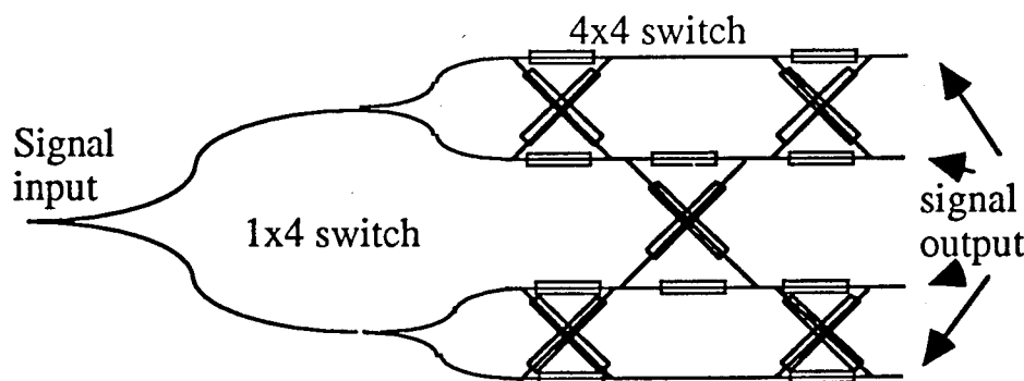
Figure 5.26. Diagram of signal distribution for the test of 1×4 and 4×4 switches.
