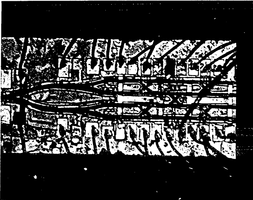
Figure 5.28. Wire bonded 1x4 and 4x4 switches.
