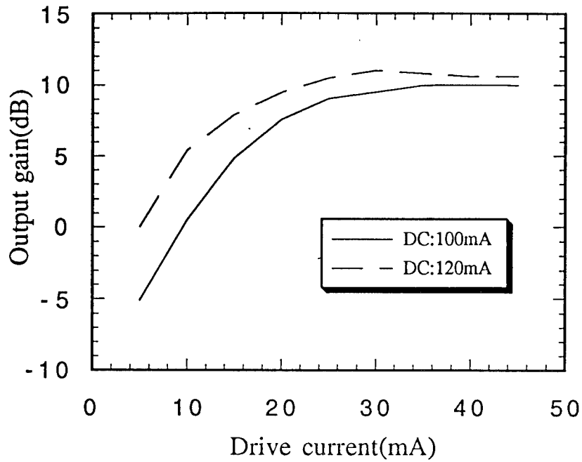
Figure 5.17. Output gain of the 1×2 switch with DC arm pulsed-biased (1KHz and 10% duty cycle) vs. the (CW) current through one of the switch arms. The solid line is for I = 100 mA, and dashed line is for I = 120 mA.
