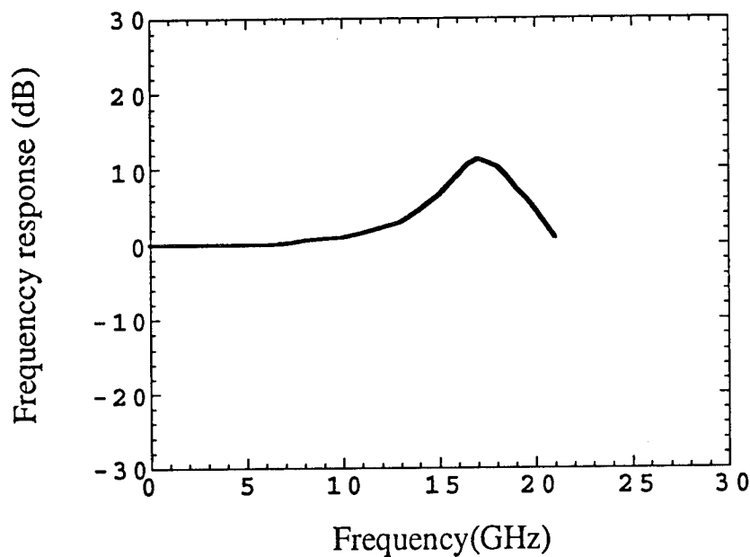
Figure 5.15. Small signal frequency response of a 1x1 switch/modulator biased at 60 mA.
