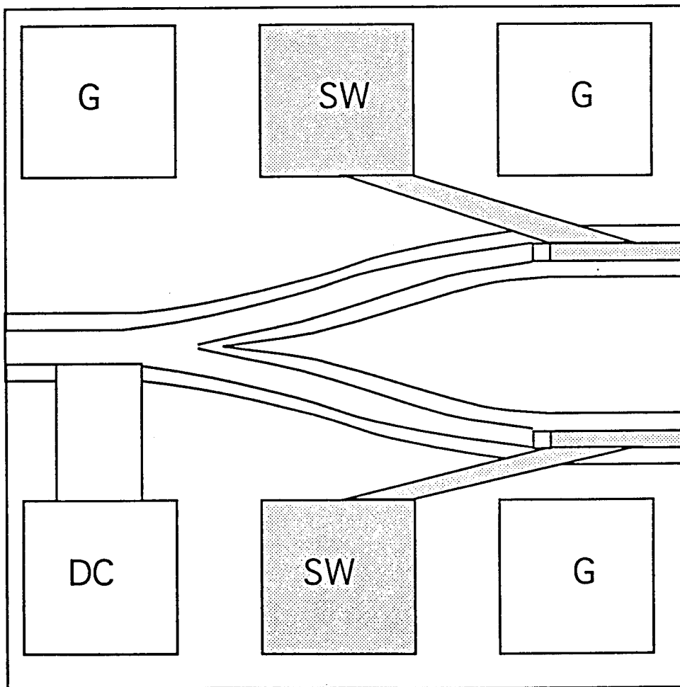
Figure 2.12. The structure of an 1 \times 2 switch.
