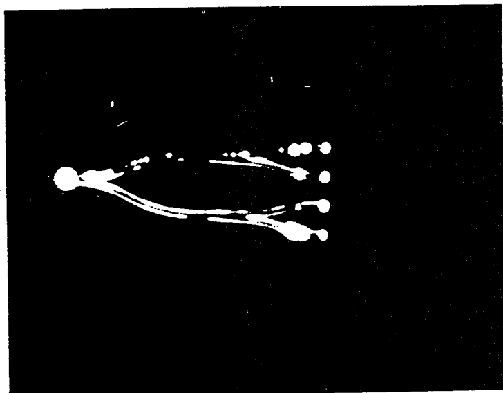
Figure 5.29. Top view of the 1×4 switch with a proper bias.
