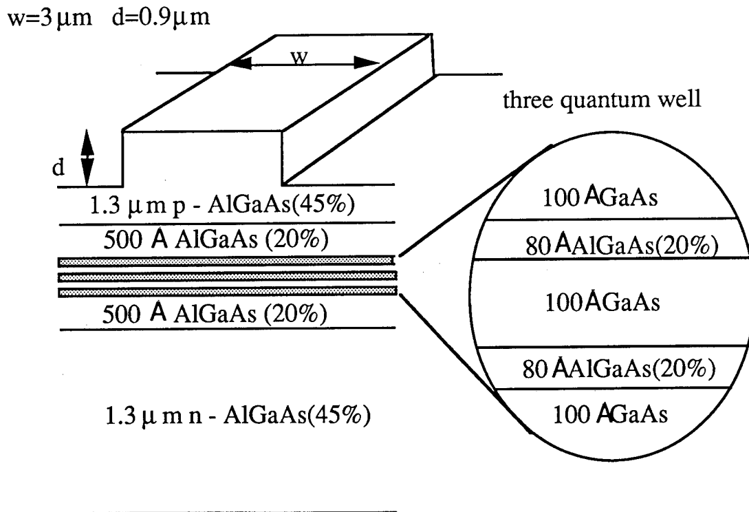
Figure 2.5. The ridge waveguide structure
