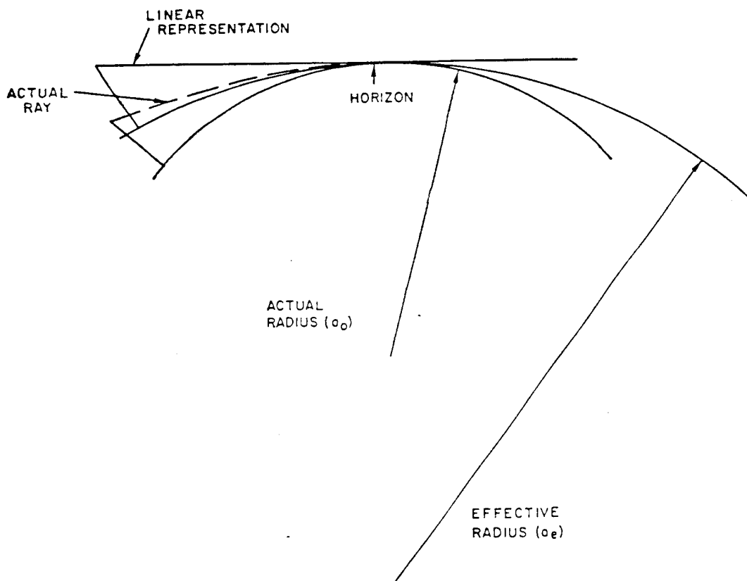
Figure 2-1. Effective Earth Radius, a_e
