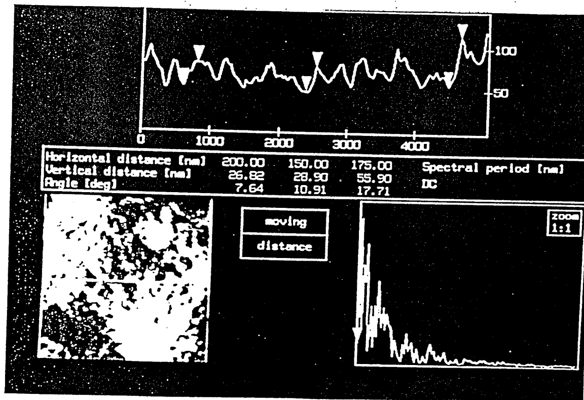
Figure 16 AFM surface roughness measurement of untreated ( above ) and treated (bottom) PE film
