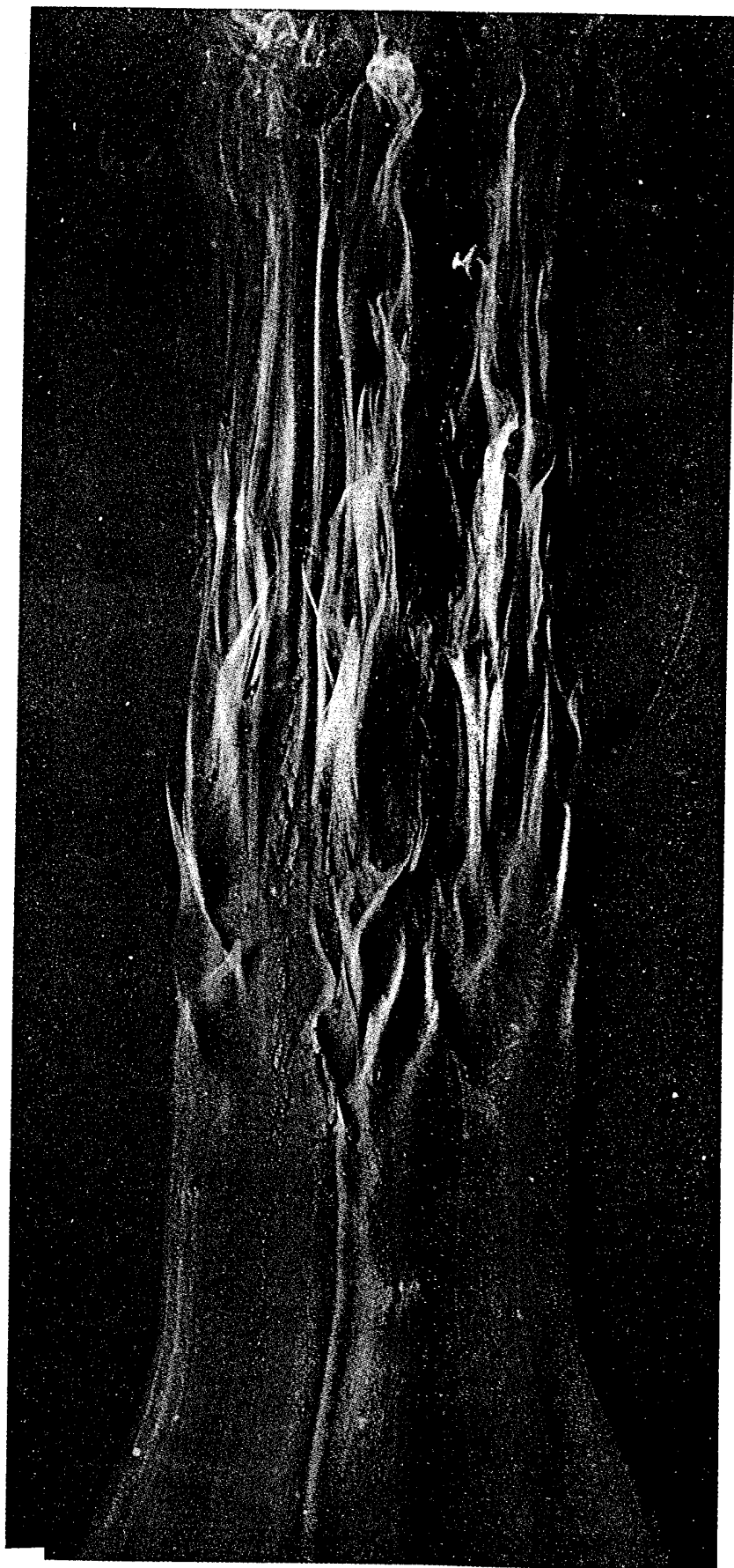
105. Natural transition on a slightly inclined plate. At the same Reynolds number of 100,000 but 1^\circ angle of at-
