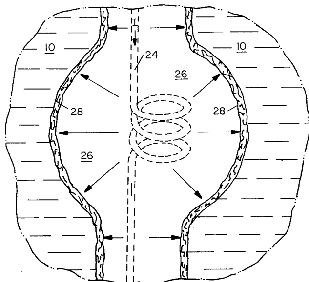
Fig. 12. Torus formation in the Koloc model. (Taken from Koloc. 19 )
