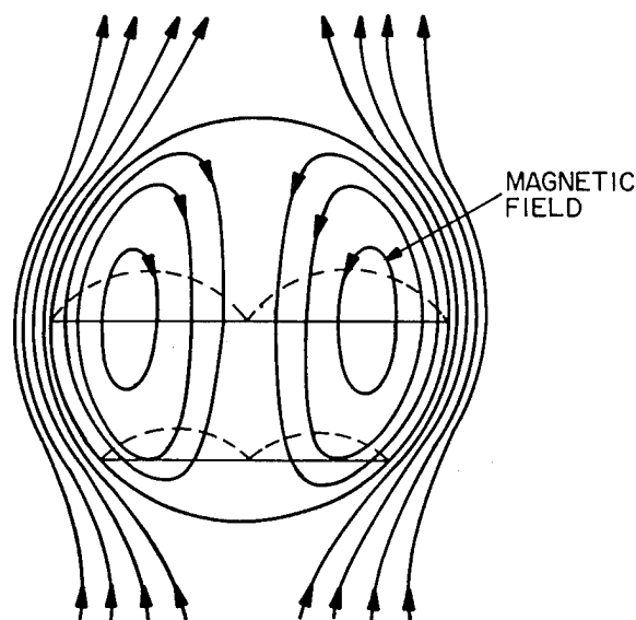
Fig. 5. The vortex plasmoid model for ball lightning. (Taken from Singer. 3 )
