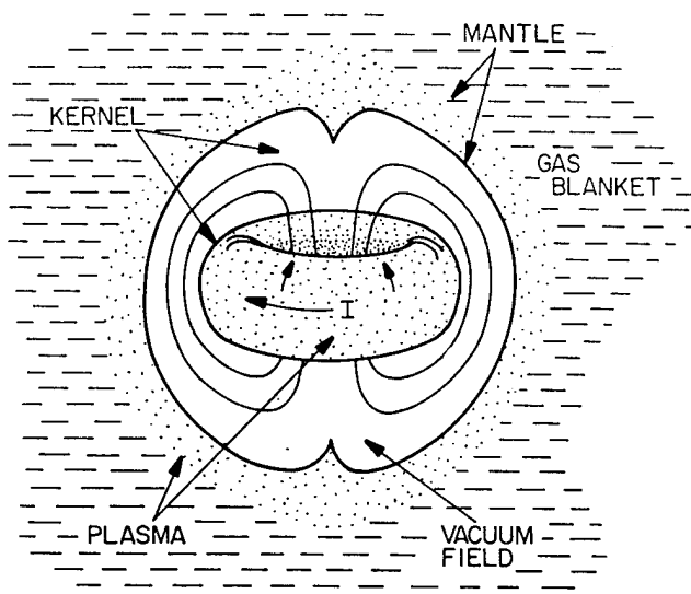
Fig. 14. The end point of the Koloc model, showing a toroidal plasma insulated from the surrounding neutral gas by a high-energy electron shell. The "kernel" forms a plasmalike bubble, which is maintained by a combination of magnetic and plasma pressure against the pressure of the surrounding atmosphere.
