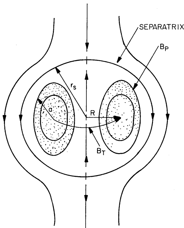
Fig. 8. The spheromak configuration. A weak vertical magnetic field stabilizes a toroidal current-carrying plasma. (Taken from Roth. 12 )
