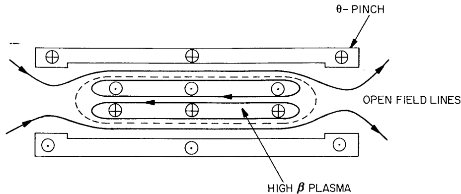
Fig. 7. The field-reversed theta pinch. (Taken from Roth. 12 )
