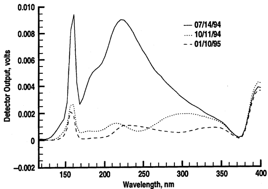
Figure 2. Deuterium lamp spectra.
