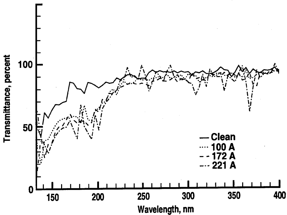
Figure 7. Transmittance as function of RTV-566 film thickness.
