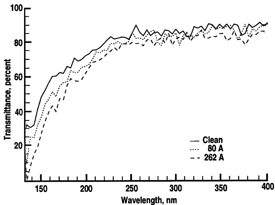
Figure 5. Transmittance as function of RTV-142 film thickness.
