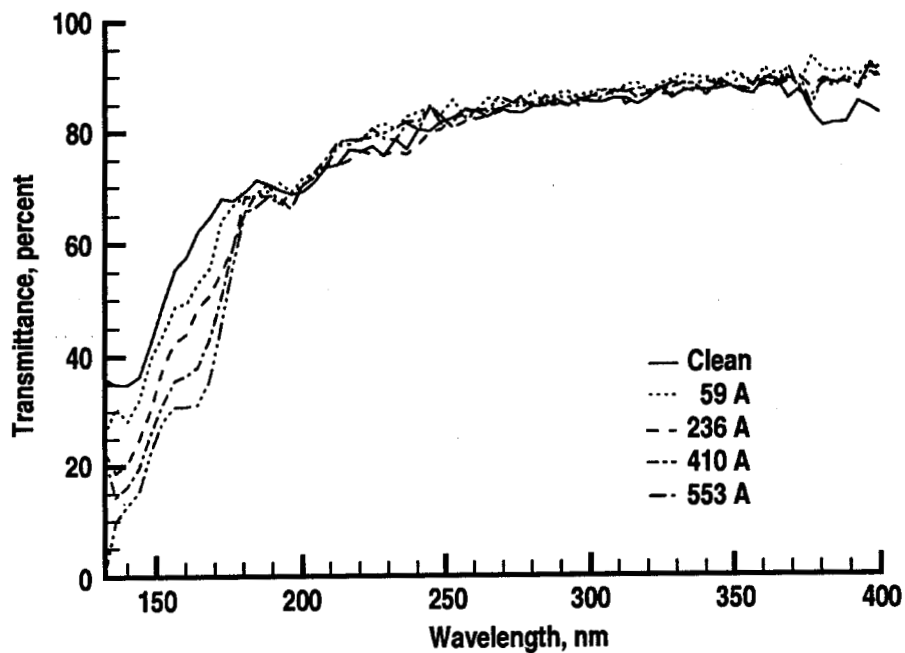
Figure 3. Transmittance as function of DC6-1104 film thickness.
