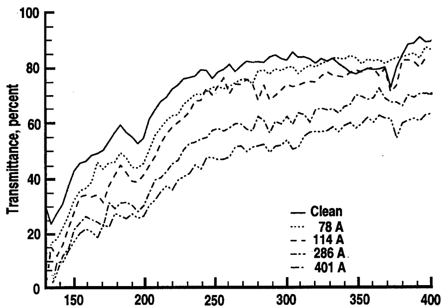
Figure 4. Transmittance as function of Solithane film thickness.
