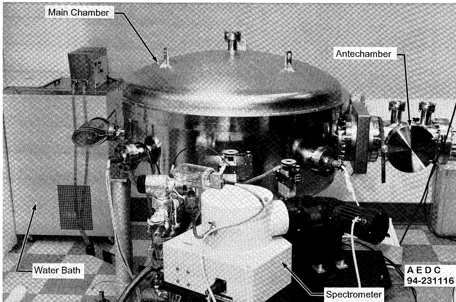
Figure 1. Vacuum Ultraviolet Measurements Chamber.
