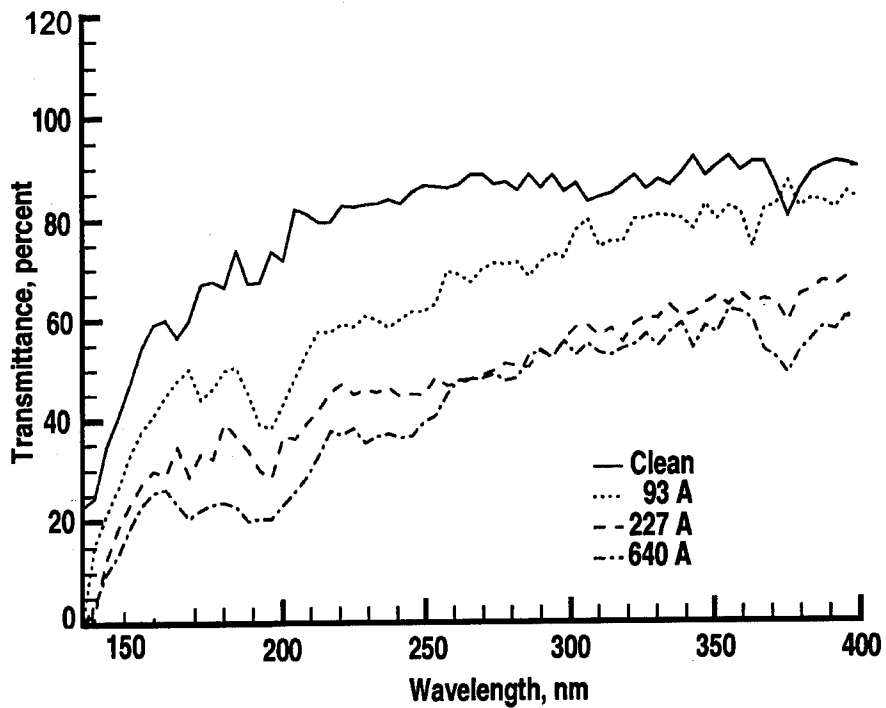
Figure 6. Transmittance as function of Uralane® film thickness.
