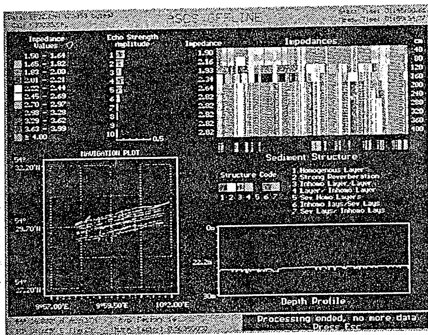
Figure 3: Color display of the ASCS sediment characterization program showing the impedance (upper right) measured along track lines (lower left) in the CBBL/JOBEX test.
