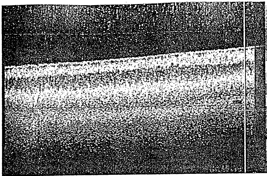
Figure 2: ASCS subbottom seismic profile of sediments in the CBBL/JOBEX experiment area, Eckernförde Bay, SW Baltic Sea. A biogenic gas horizon is shown at about 1 m below the sediment water interface.
