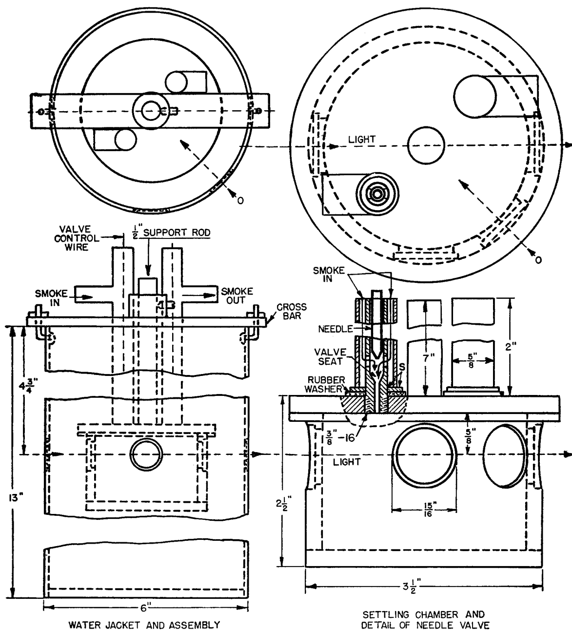
FIGURE 4. Differential settler.
