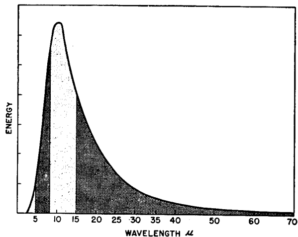
FIGURE 4. Energy distribution in black-body radiation at 300 K. Shaded portions are regions of water-vapor absorption.
