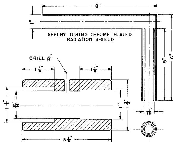
FIGURE 16. Diagram of radiation shield.
