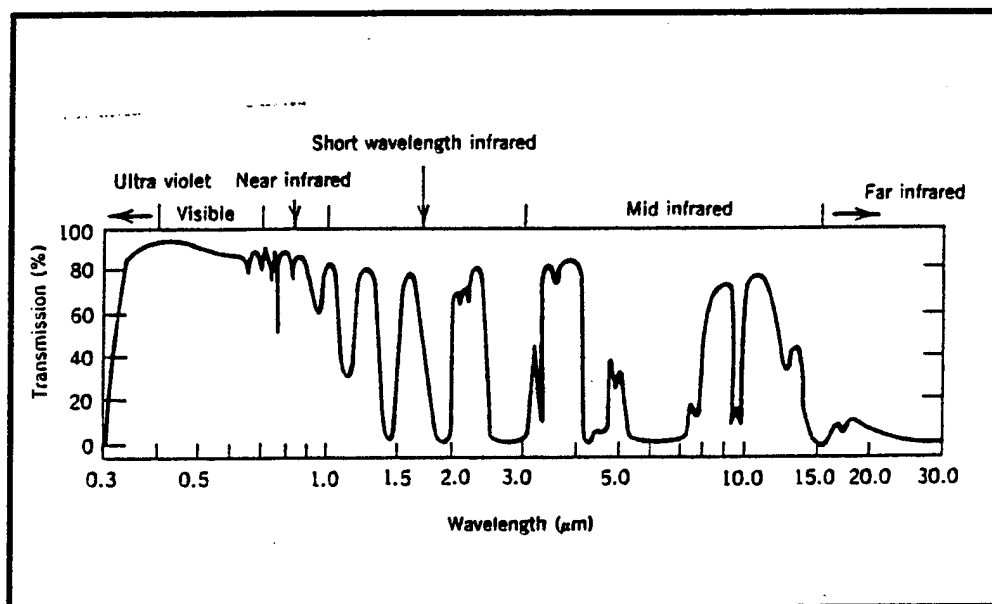
Figure 5. Atmospheric Transmission Windows "From Ref 16"
