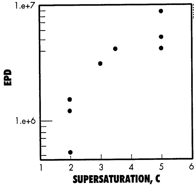
Figure 29 The average dislocation etch pit density.
