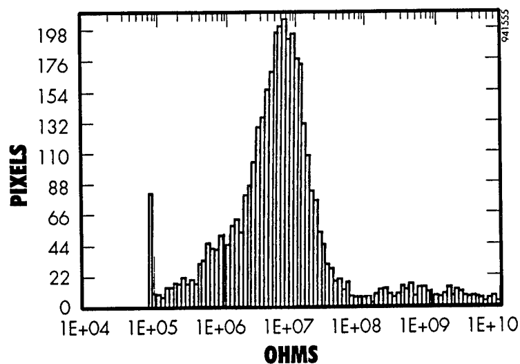
Figure 31 A histogram of differential resistance at a bias of -20\text{mV} at 87\text{K} .
