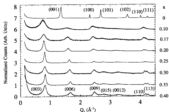
Fig. 2. The composition, x , dependence of the room-temperature, Cu K \alpha powder X-ray diffraction patterns of [(\text{CO}_3)_{x/2} \cdot y(\text{H}_2\text{O})]_{-x}[\text{Ni}_{1-x}\text{Al}_x(\text{OH})_2] . These patterns were acquired with an instrument resolution of 0.006 \text{ \AA}^{-1} .
