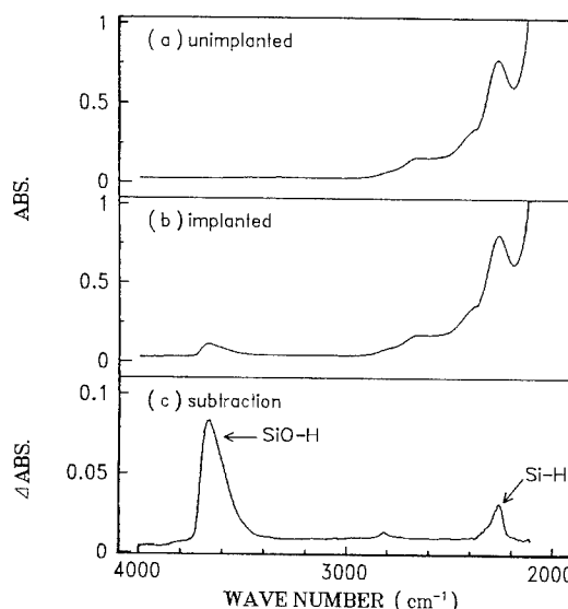
Fig. 3. Changes in infrared absorption spectra of \text{SiO}_2 glass (type IV) upon implantation of \text{H}^+ ions (150 keV, 1 \times 10^{18} \text{ cm}^{-2} ). Two induced bands peaking at \sim 3670 and 2230 \text{ cm}^{-1} are due to stretching vibrations of Si–OH and Si–H bonds.
