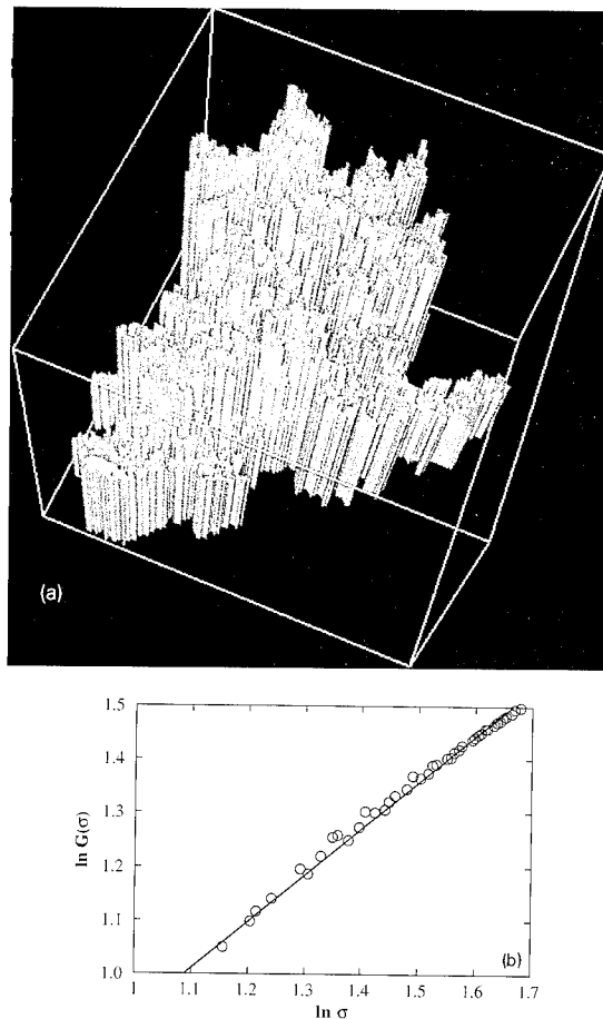
Fig. 5. (a) Snapshot of an internally fractured surface resulting from a percolating pore in silica glass at a mass density of 1.4 \text{ g/cm}^3 . (b) Height–height correlation function ( \circ ) versus the in-plane distance, \sigma , for the fracture surface of a 1.12 million particle silica system computed on IBM SP-1. The solid curve is the best fit, G(\sigma) \propto \sigma^\alpha , with \alpha = 0.87 \pm 0.02 for \sigma < 100 Å.
