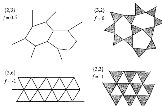
Fig. 2. Four two-dimensional networks constructed using one-dimensional rod and two-dimensional triangular polytopes, with the corresponding connectivities and structural freedoms indicated.
