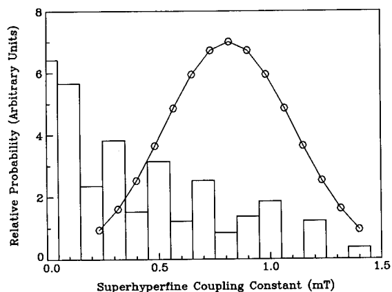
Fig. 9. Histogram (bar graph) of E'_1 -center ^{29}\text{Si} superhyperfine coupling constants developed from Fig. 5 by assuming a totally random (flat) distribution in dihedral angle, \alpha_1 , and the MW distribution in Si–O–Si angles. In principle, this distribution would independently apply to ^{29}\text{Si} s occupying each of the three near-neighbor silicon positions, Si(2), Si(3), and Si(4) in Fig. 4(a). The circles represent a Gaussian SHFS distribution discussed in the text.
