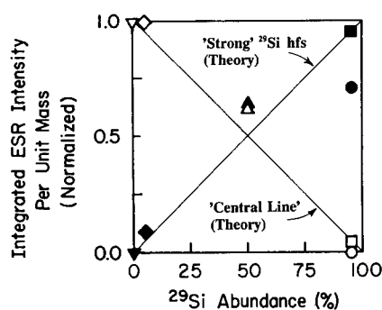
Fig. 6. ESR intensity per unit sample mass versus isotopic abundance for the E'-center 'central line' (open symbols) and 'strong' ^{29}\text{Si} hyperfine structure (filled symbols) in the silica glasses of the present study. Deviations from the predicted behavior (diagonal straight lines) are tentatively ascribed to experimental error and/or slight differences in glass structure. (After Ref. [23].)
