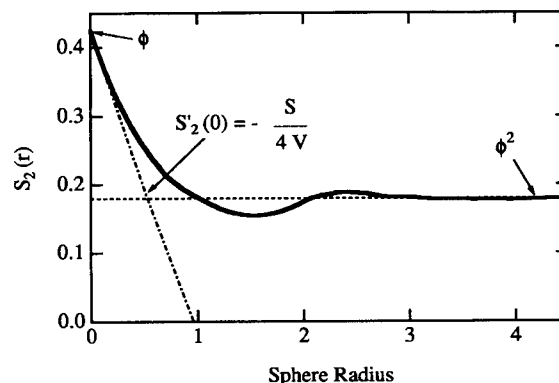
Fig. 1. Structure factors, S_2(r) , for model materials composed of impenetrable spheres.
