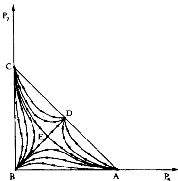
Fig. 2. The phase diagram of the differential system (6).
