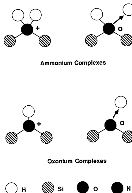
Fig. 2. Local atomic arrangements in positive and neutral charged and neutral ammonium and oxonium clusters. The positively-charged clusters (a) and (c) are stable. The neutral clusters are unstable with respect to the loss of a single H atom (indicated by the arrow).
