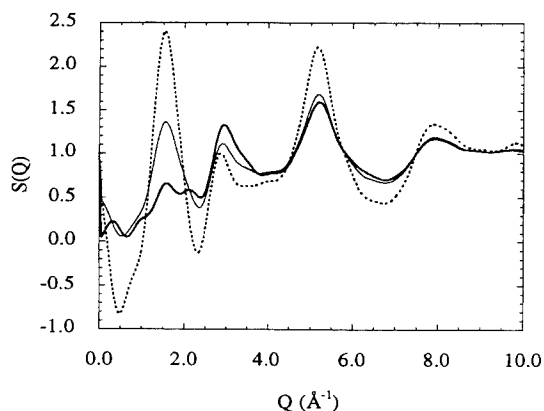
Fig. 4. Calculated total structure factors for a model of v\text{-SiO}_2 [32]: —, unmodified; (---) Li-stuffed; (—) Na-stuffed. The compositions of the alkali-stuffed structures were (M_2)(\text{SiO}_2)_2 ( M = \text{Li}, \text{Na} ).
