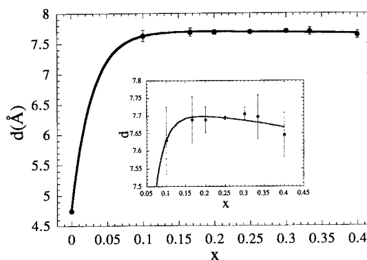
Fig. 3. The composition, x , dependence of the measured room-temperature basal spacing of [(\text{CO}_3)_{x/2} \cdot y(\text{H}_2\text{O})]_{-x}[\text{Ni}_{1-x}\text{Al}_x(\text{OH})_2] obtained from a q -plot of the (00 l ) reflections of the powder patterns shown in Fig. 2. (See text.)
