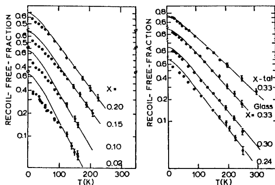
Fig. 8. Site A temperature dependence of the Mössbauer-Debye-Waller factor, f(T) , in (\text{Ge}_{0.99}\text{Sn}_{0.01})_x\text{Se}_{1-x} glasses at indicated cation concentration, x . In c- \text{GeSe}_2 , note that f(T) is well fitted by one Debye temperature, while in glasses a softening of f(T) is observed at low T on account of the floppy modes. This figure is taken from Ref. [12].
