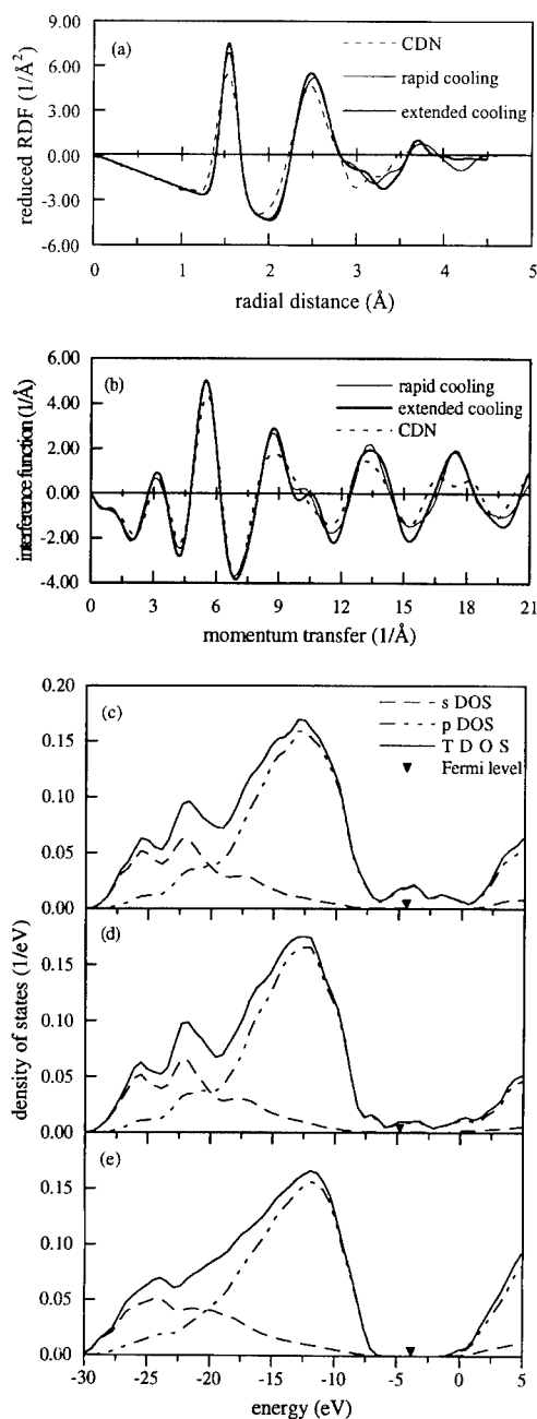
Fig. 4. Diffraction and electronic data for the diamond density a-dia models. (a) reduced radial distribution function in comparison with that of a four-fold-coordinated CDN; (b) interference function in comparison with that of a four-fold-coordinated CDN; (c) density of states for the rapidly cooled DF-MD model; (d) density of states for the extended stochastically cooled DF-MD model; (e) density of states for the 512 atoms WWW-CDN model.
