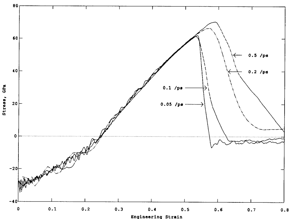
Fig. 6. Stress–strain curves at various strain rates for low cristobalite formed using the three-body FG-potential function.
