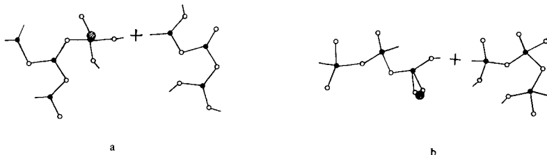
Fig. 10. Two elementary agglomeration processes: (a) in a B_2O_3 + nLi_2O glass ( B_3 + B_3 ( m' = 3 , m = 2 )); (b) in a SiO_2 + n(CaO, Na_2O) glass ( Si_3 + Si_3 ( m' = 1 , m = 3 )).
