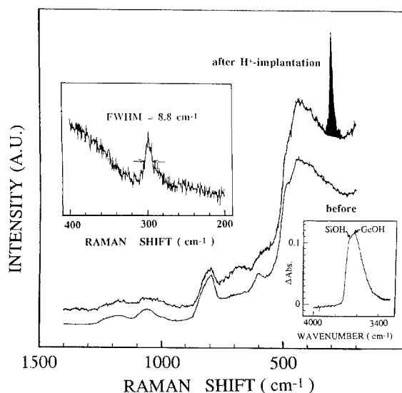
Fig. 6. Raman spectra of 10\text{GeO}_2 - 90\text{SiO}_2 glass substrate before and after \text{H}^+ ( 1.5\text{ MeV} , 1 \times 10^{18}\text{ cm}^{-2} ) implantation. The inset (upper left) shows a portion of the sharp band appearing at \sim 300\text{ cm}^{-1} measured at a resolution of 1\text{ cm}^{-1} . Excitation: \text{Ar}^+ laser ( 514.5\text{ nm} , 250\text{ mW} ). Infrared absorption bands of \text{SiOH} and \text{GeOH} are observed in the substrate after implantation as shown in the inset (lower right).
