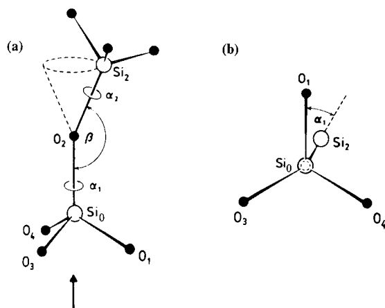
Fig. 1. Definitions of Si–O–Si bond angle, \beta , and dihedral angles, \alpha_1 and \alpha_2 . Dashed cone in (a) represents the locus of possible positions of \text{Si}_2 obtainable by varying \alpha_1 for fixed \beta . Panel (b) is a view along direction of arrow in (a). (Adapted from Ref. [2].)
