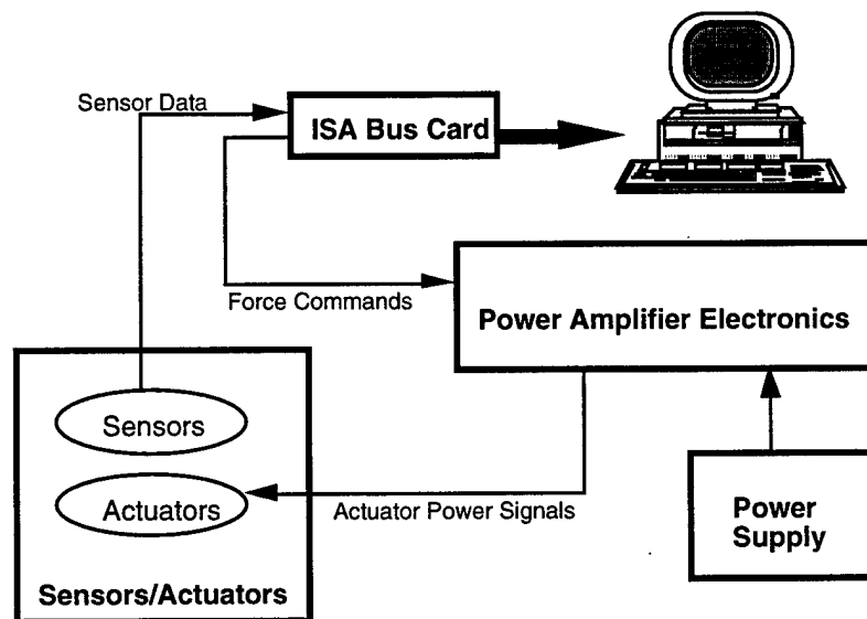
Figure C-5, Electronics Design Overview
