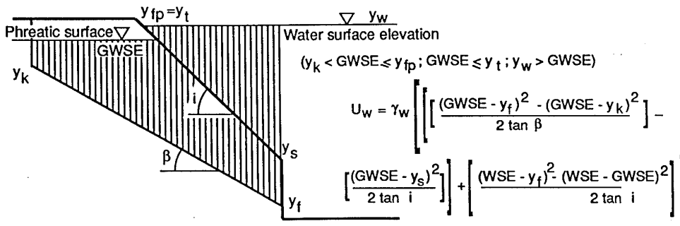
Figure 6 Solutions for pore water pressure
