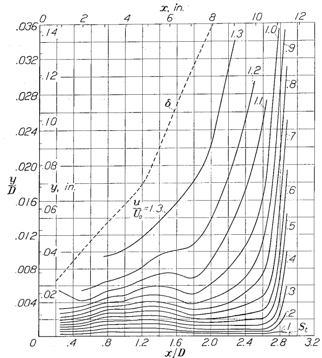
FIGURE 12.—Contours of equal speed in boundary layer of elliptic cylinder. Air speed ( U_0 ), 60 feet per second; R , 118,000; stream turbulence as shown by figure 9.
