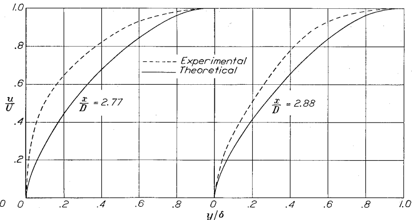
FIGURE 14.—Comparison of observed profiles with Fediaevsky theory.
