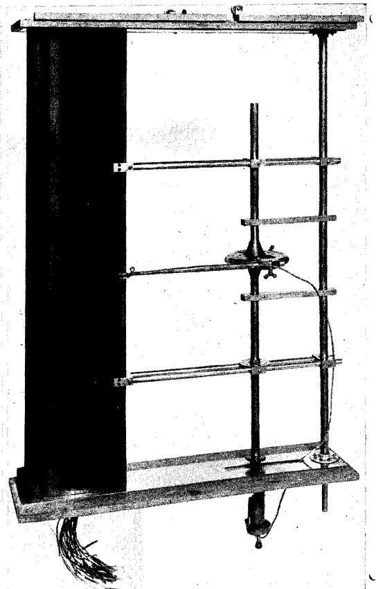
FIGURE 2.—Photograph showing over-all view of elliptic cylinder and traversing equipment.
