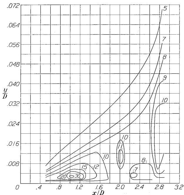
FIGURE 18.—Contours of equal u/U_0 in boundary layer. Numbers on curves give values of 100 u/U_0 . Air speed, 60 feet per second; stream turbulence as show in figure 9.
